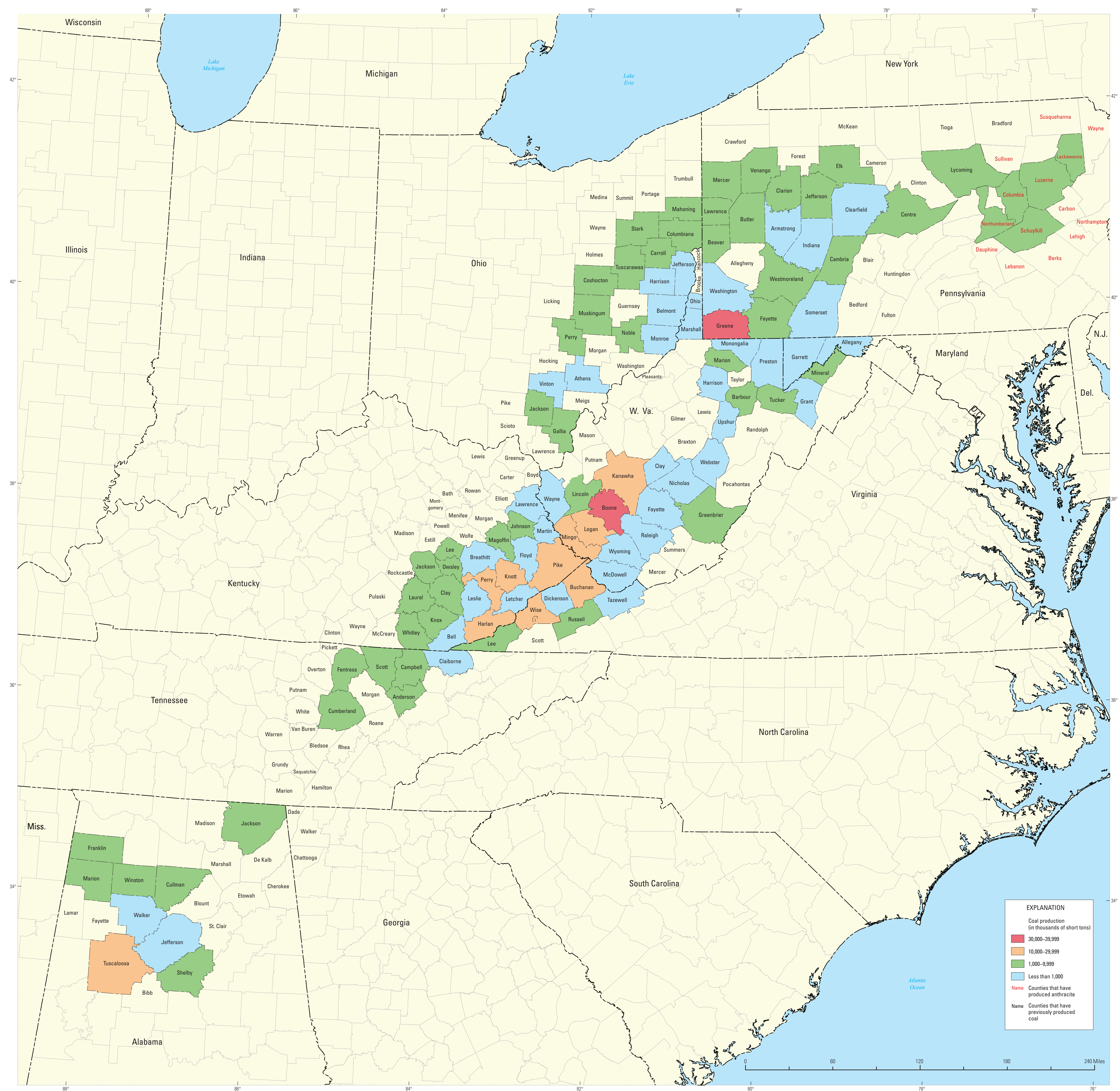
Figure 4. Current (2003) annual coal production by county. D.C., District of Columbia; Del., Delaware; Miss., Mississippi; N.J., New Jersey; W. Va., West Virginia.
