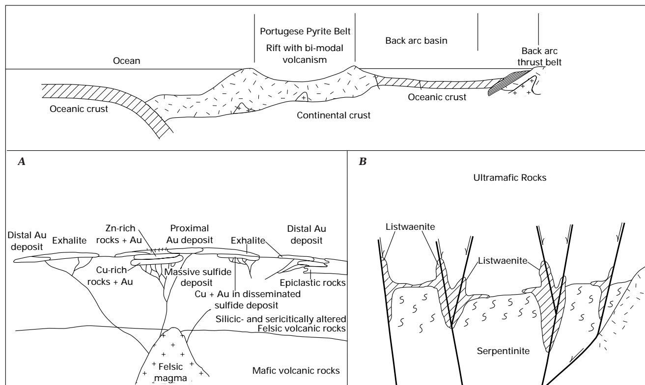
Figure 4. Schematic cross section across the South Portuguese Zone showing tectonic setting and theoretical gold occurrences. Enlarged sections of schematic cross sections of A , Portuguese Pyrite Belt and B , Mobile Belt. Back arc rocks in South Portuguese Zone preserved only in back arc thrust (Mobile Belt).
