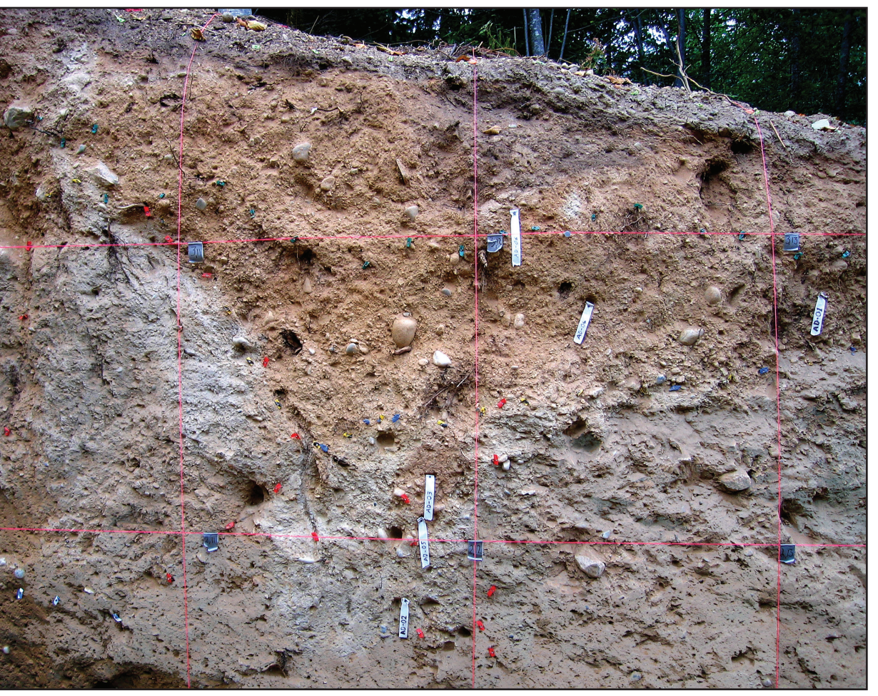
Figure 9. Photograph of upper part of fault zone (F5) in center of Saguache trench. Unit labels correspond with those on trench log. White flagging shows location of ^{14}\text{C} samples (table 1). Red marks are placed along fault.
