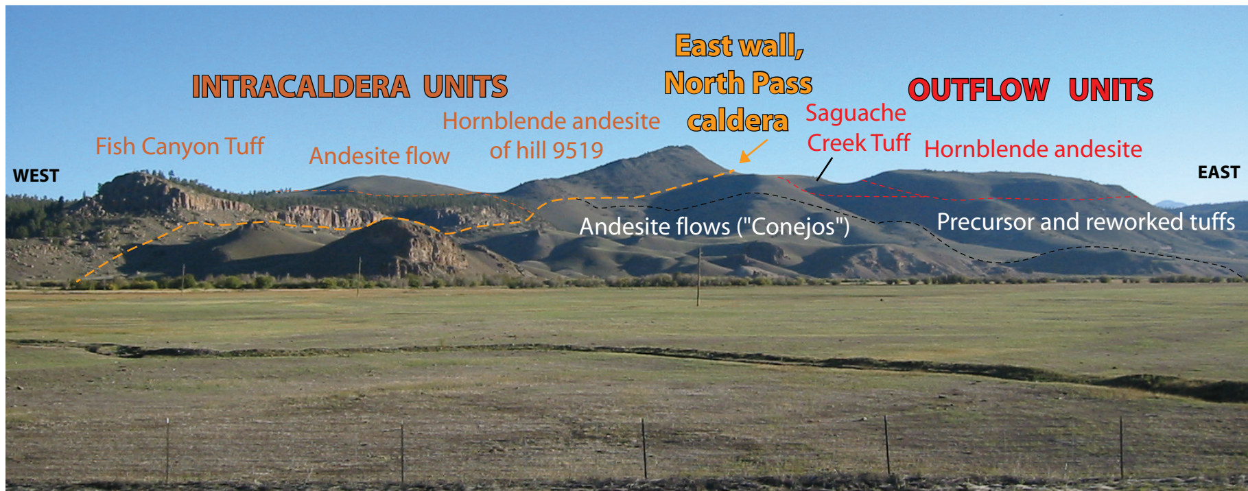
Photo 6 (fig. 8, pamphlet). East wall of North Pass caldera , as viewed obliquely from the south across Saguache valley (along Colorado Hwy 114). Outflow Saguache Creek Tuff (32.2 Ma) and underlying Conejos lavas and tuffs are abruptly truncated along caldera wall; then onlapped by ponded caldera-filling dacite and andesite lavas (~30 Ma) and overlying Fish Canyon Tuff (28.02 Ma).
