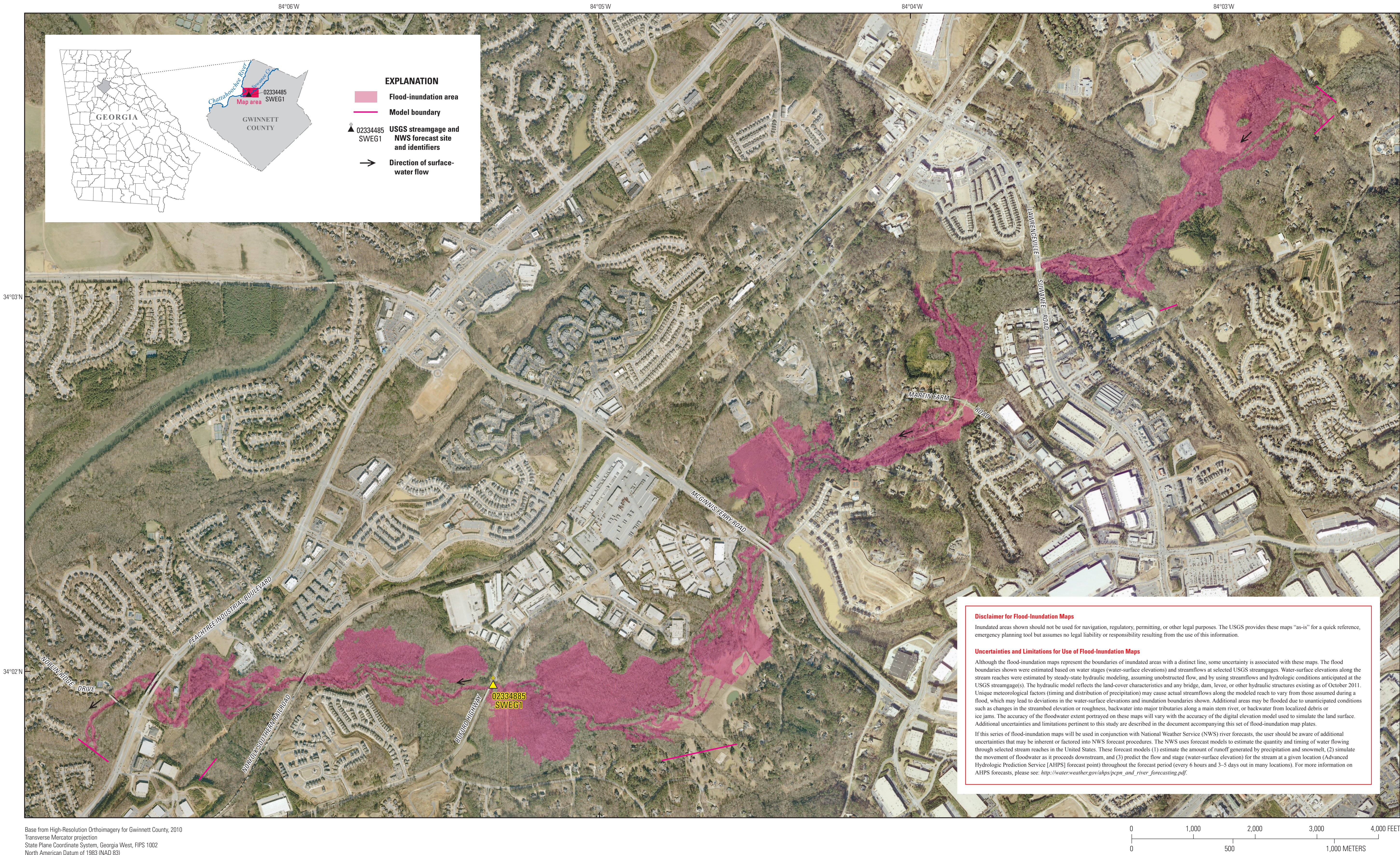
Flood-Inundation Map of Suwanee Creek in Gwinnett County, GA, Corresponding to a Gage Height of 7.5 Feet and an Elevation of 917.4 Feet (NAVD 88) at U.S. Geological Survey Streamgage Suwanee Creek at Suwanee, GA (02334885)
