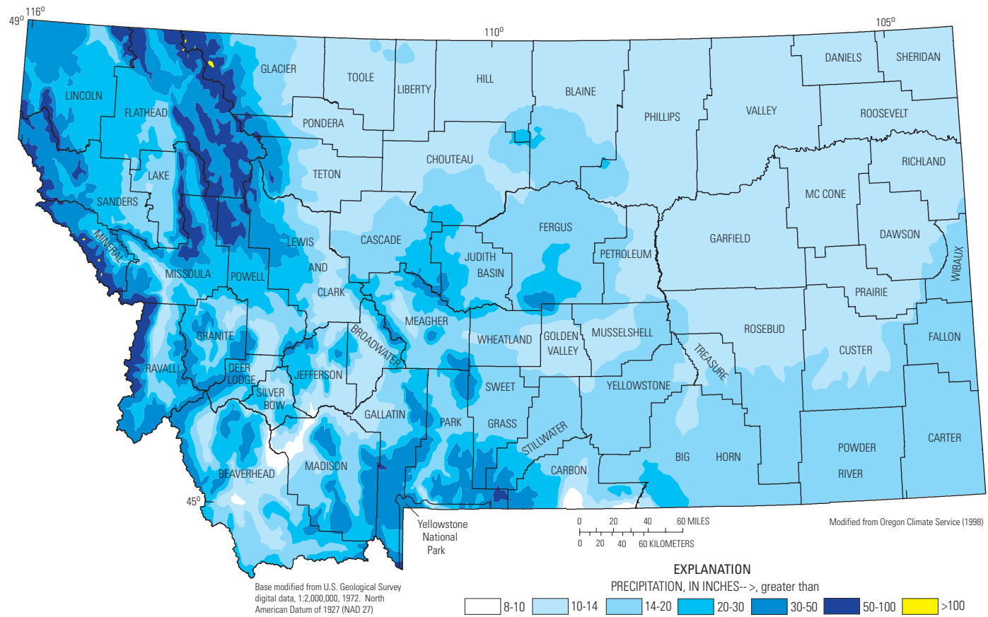
Figure 3. Average annual precipitation in Montana, 1961-90.
