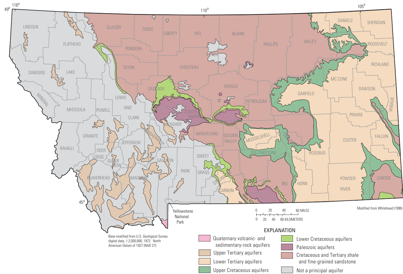
Figure 5. General extent of major aquifers in near-surface bedrock and semiconsolidated sediments in Montana.
