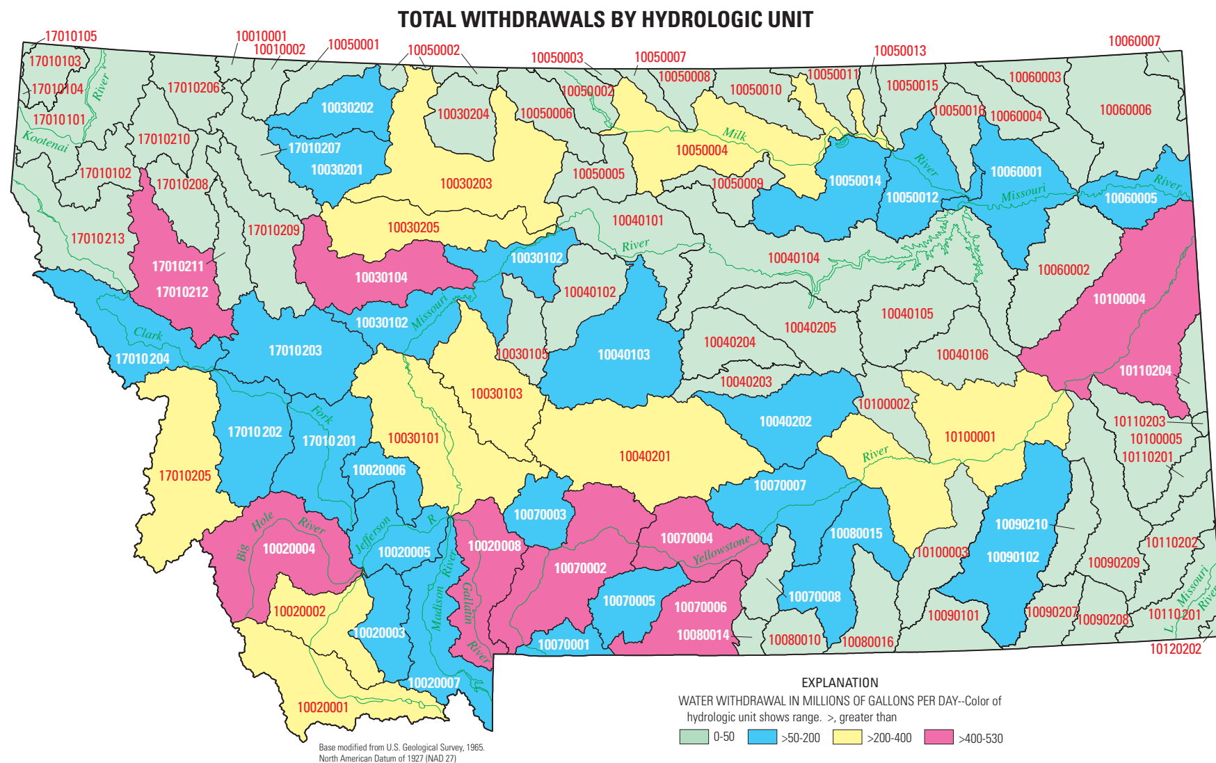
Figure 9. Total water withdrawals in Montana hydrologic units (stream basins) in 2000.
