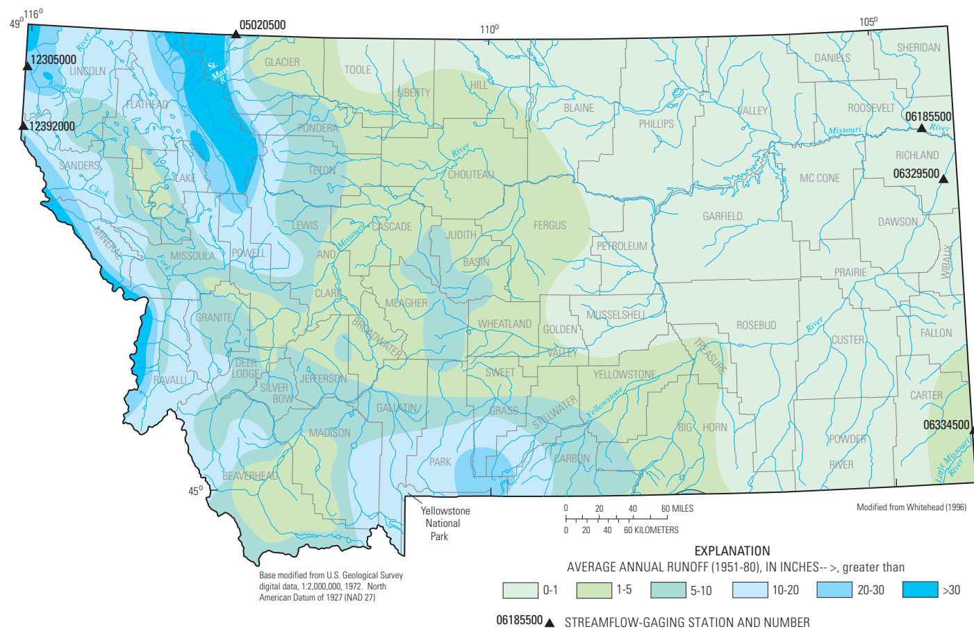
Figure 4. Average annual runoff in Montana, 1951-80.
