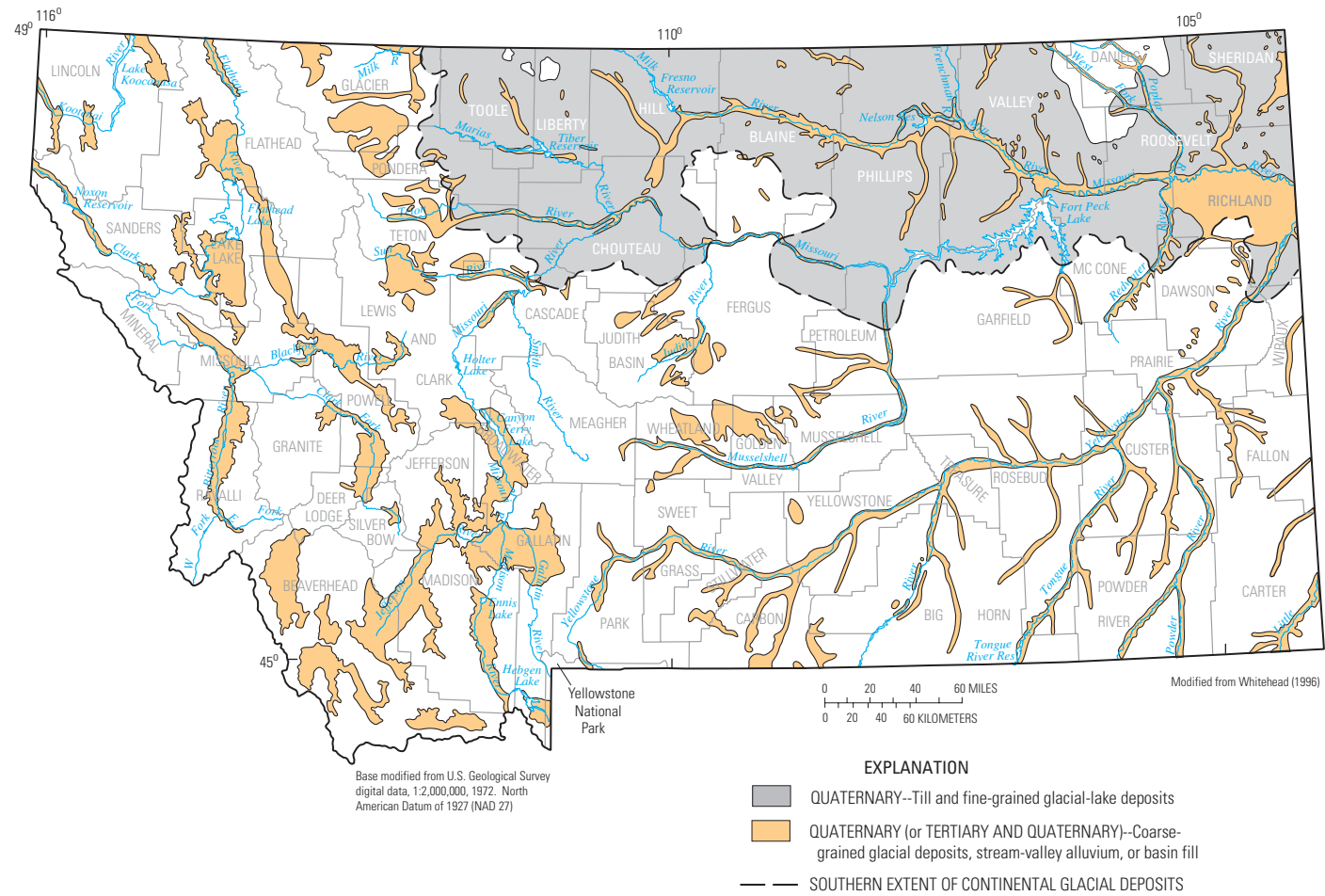
Figure 6. General extent of unconsolidated deposits that yield water to shallow wells in Montana.
