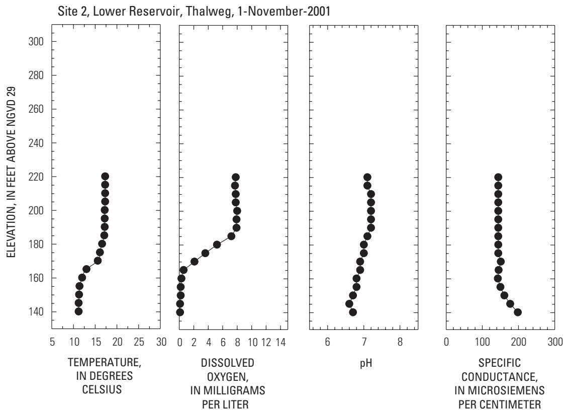
Figure D4. November 1, 2001, Site 2, Lower Reservoir, Thalweg.
