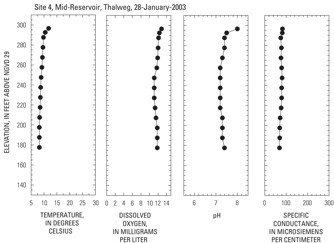
Figure D40. January 28, 2003, Site 4, Mid-Reservoir, Thalweg.
