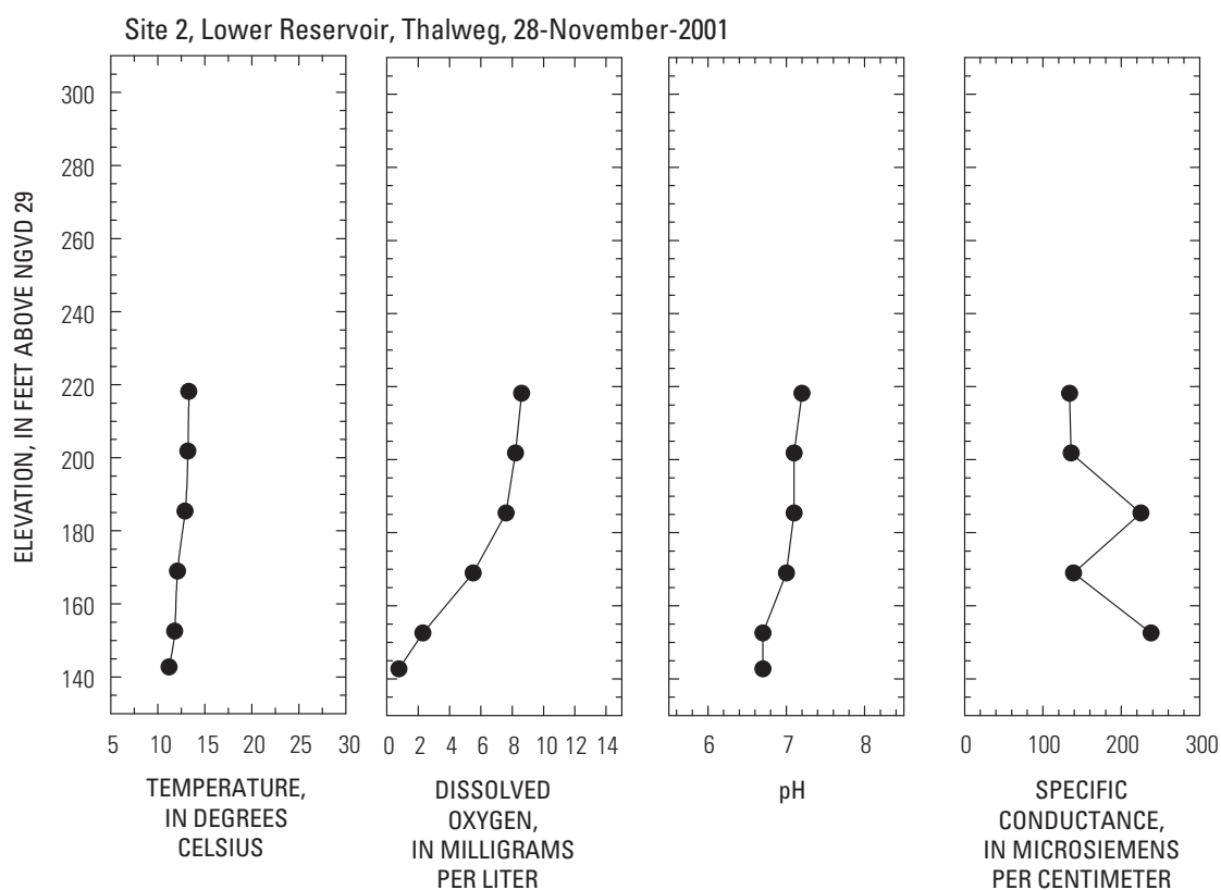
Figure D5. November 28, 2001, Site 2, Lower Reservoir, Thalweg.
