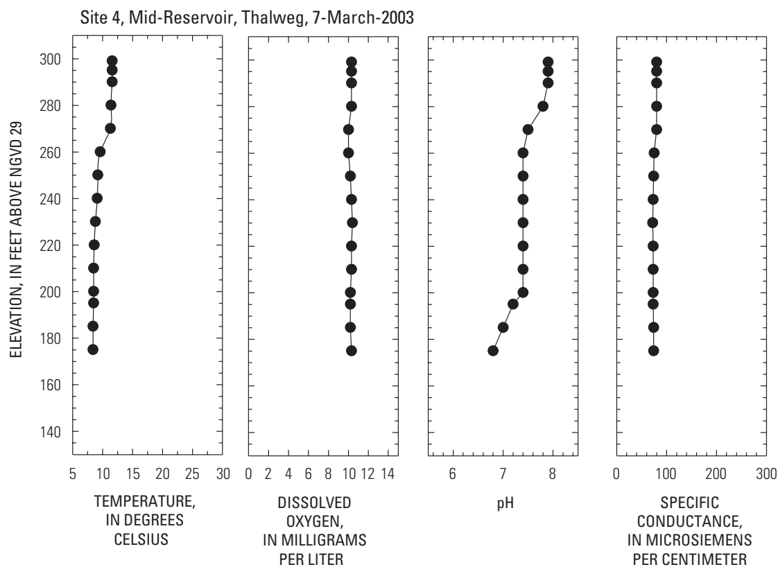
Figure D41. March 7, 2003, Site 4, Mid-Reservoir, Thalweg.
