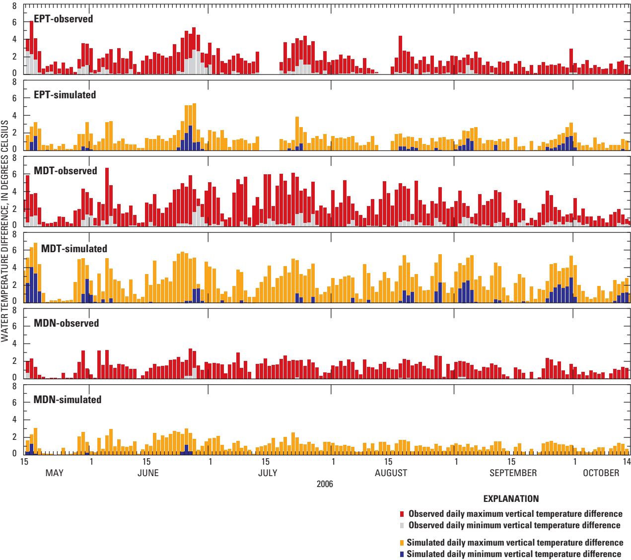
Figure 24. Daily maximum and minimum difference in temperature between near-surface and near-bottom of the water column at three deep sites in Upper Klamath Lake, Oregon, 2006.
