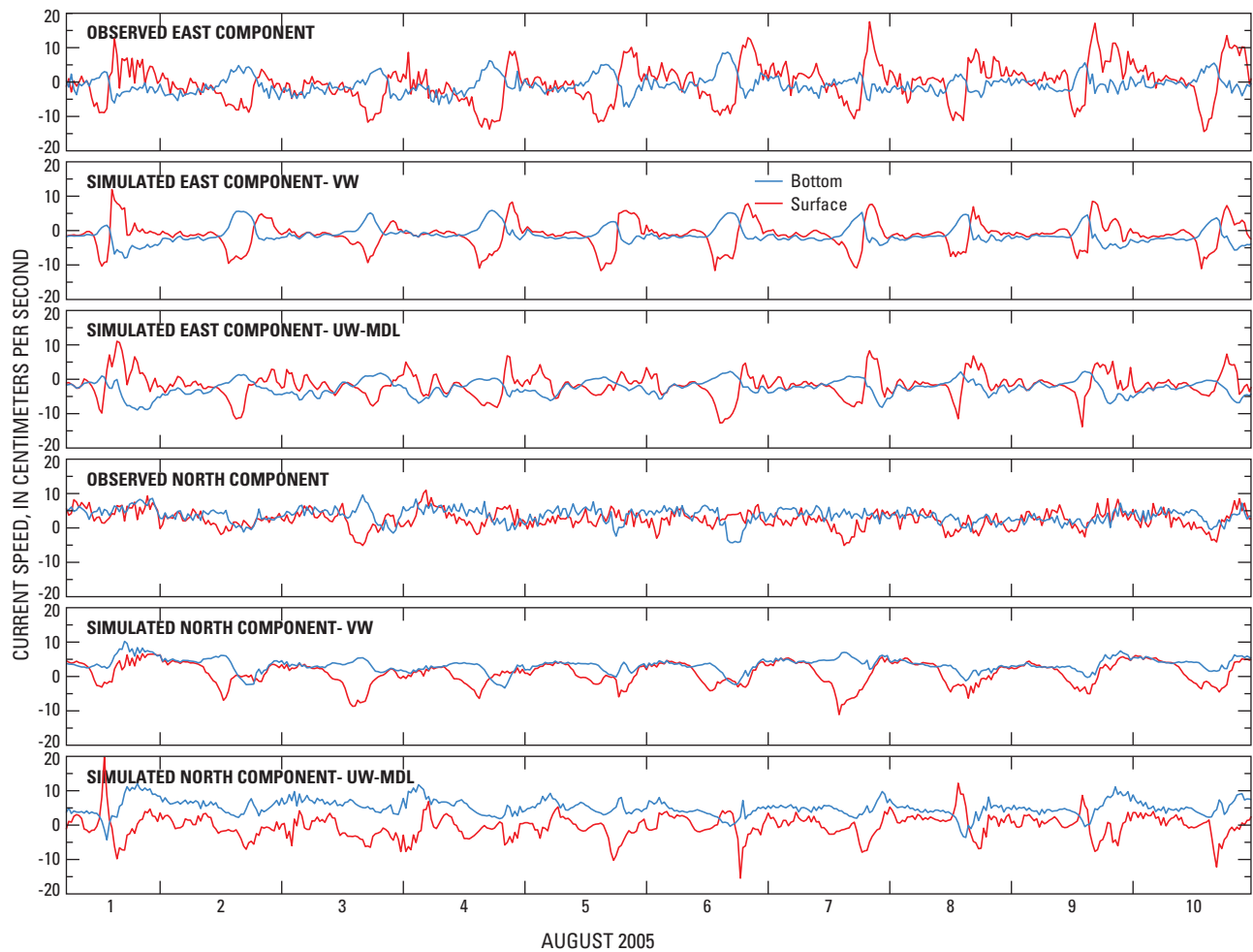
Figure 13. Observed and simulated east-west and north-south current components at site ADCP3 in Upper Klamath Lake, Oregon, 2005.
