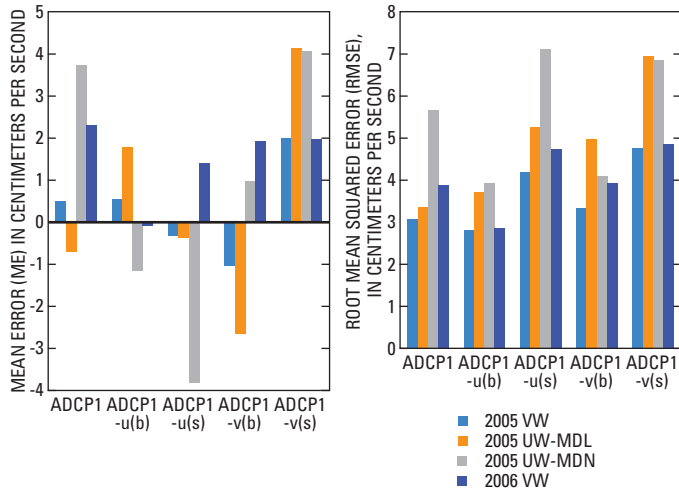
Figure 12. Goodness-of-fit velocity statistics at site ADCP1 in Upper Klamath Lake, Oregon, 2005 and 2006.
