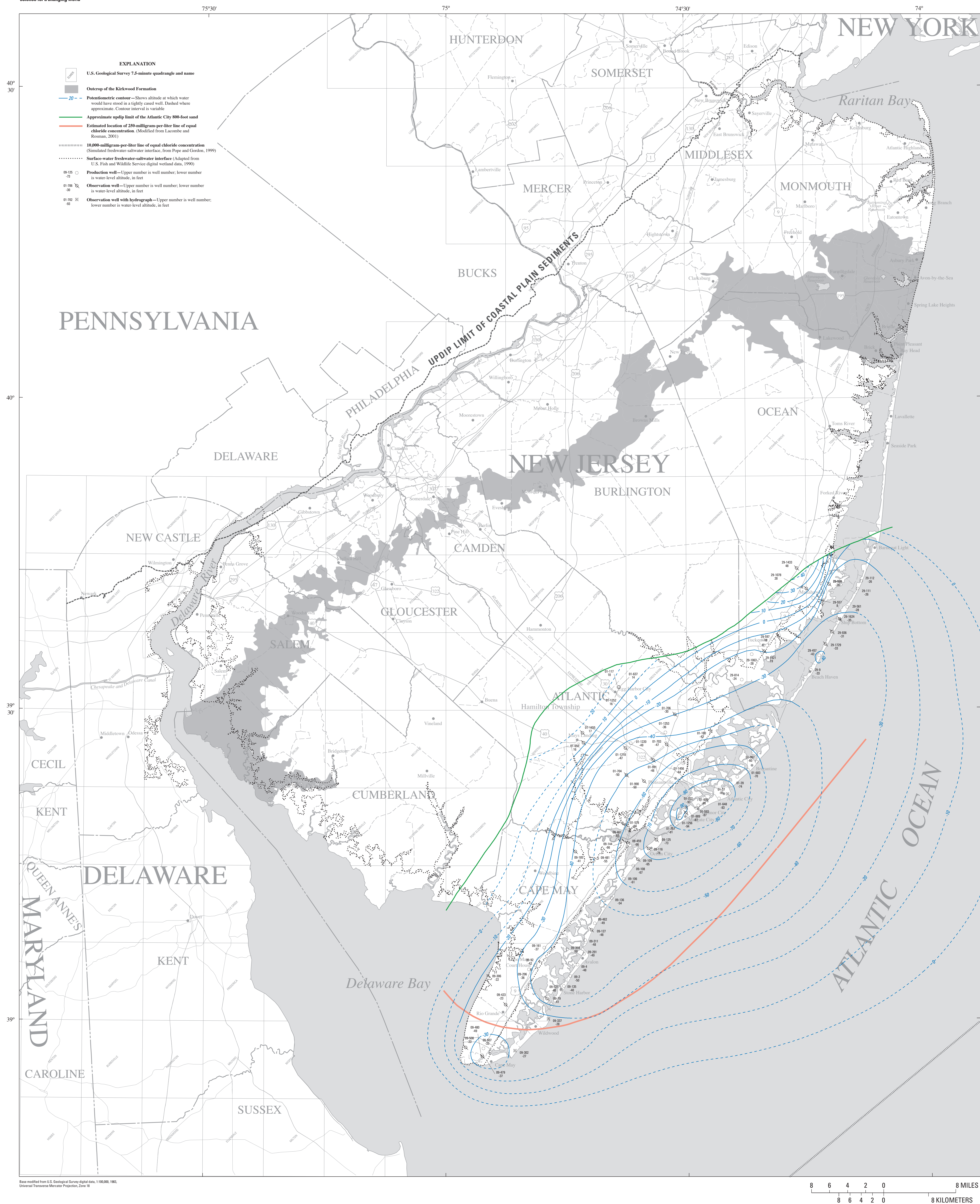
Potentiometric Surface of the Atlantic City 800-foot sand, 2003
