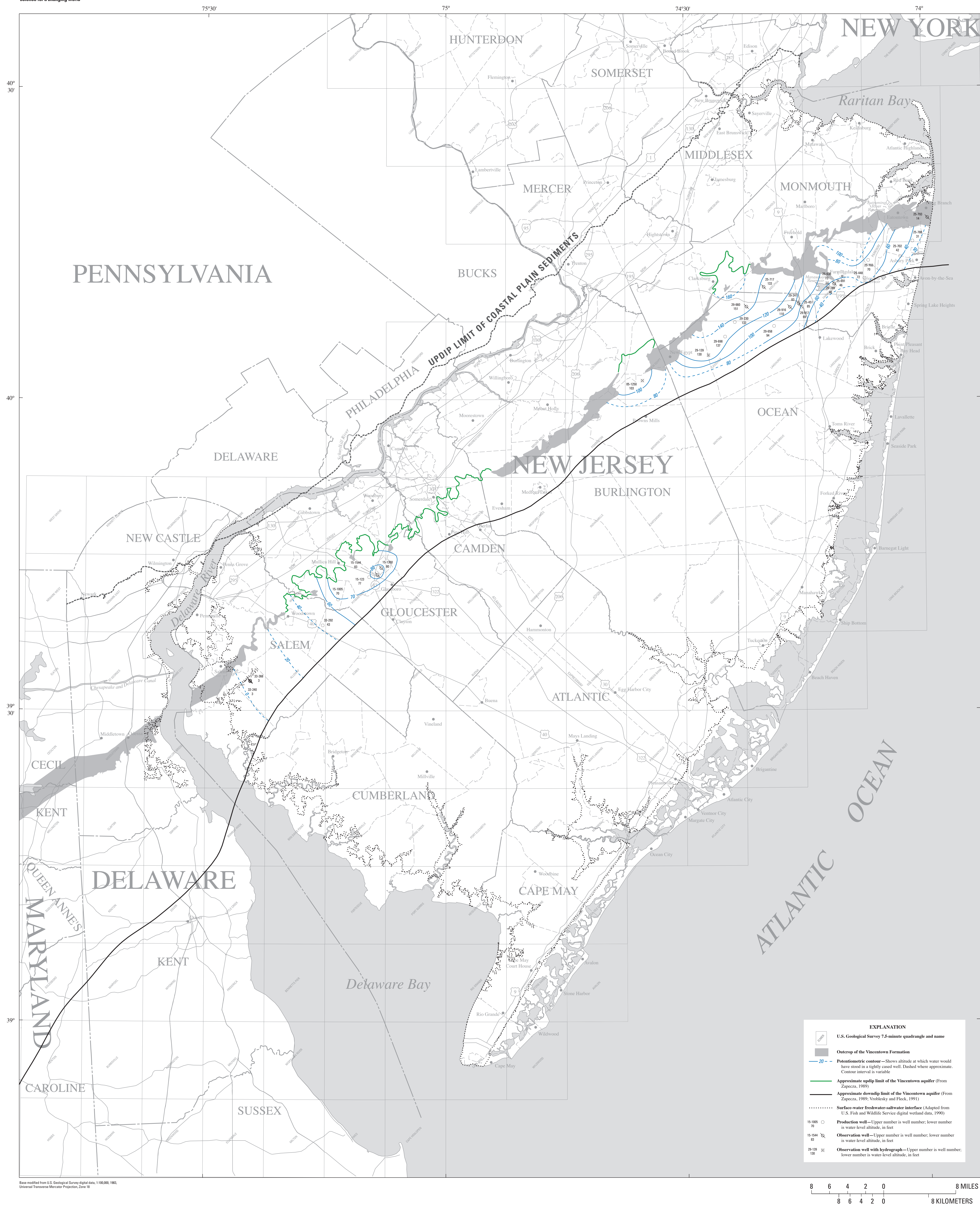
Potentiometric Surface of the Vincenttown aquifer, 2003
