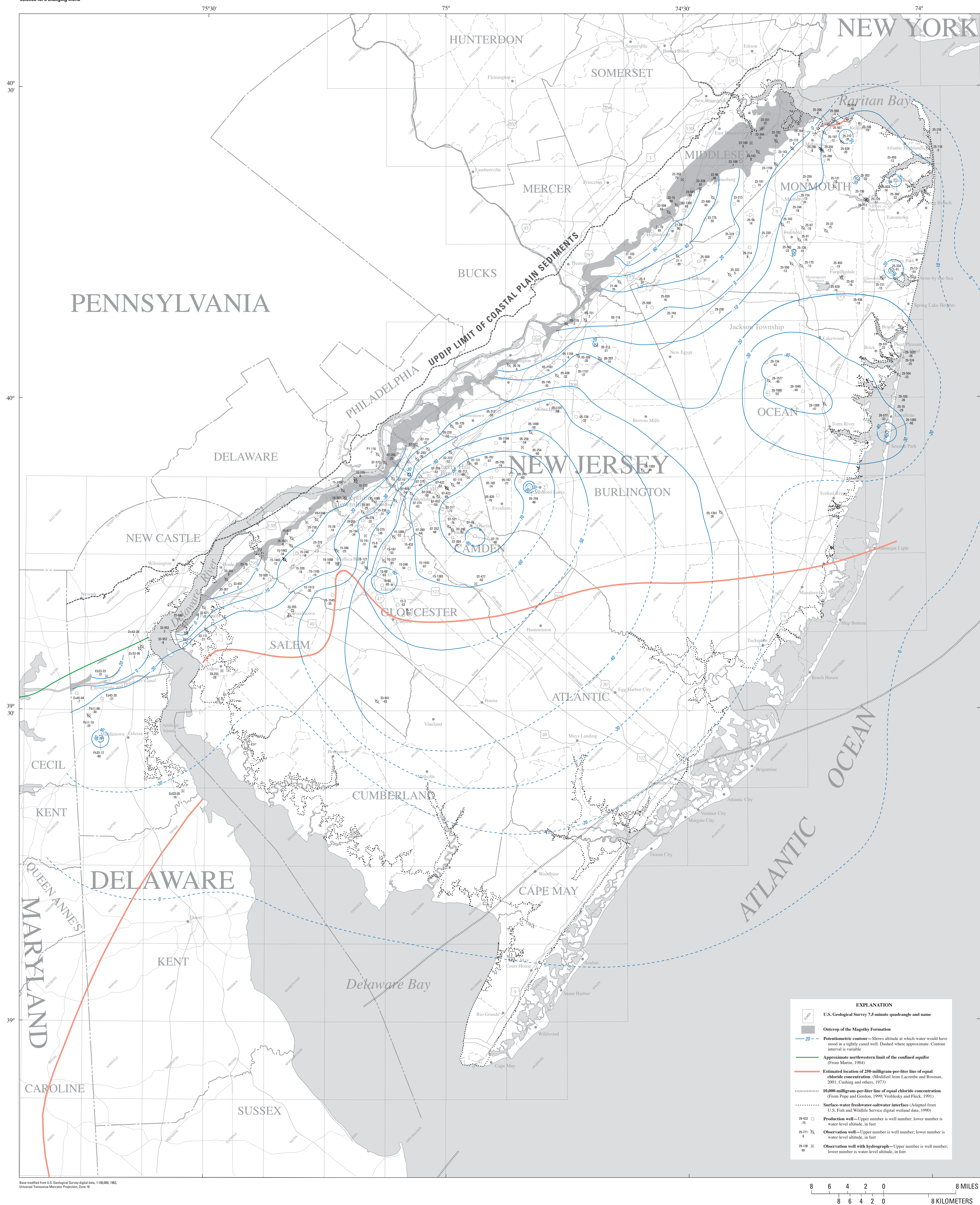
Potentiometric Surface of the Upper Potomac-Raritan-Magothy aquifer, 2003
