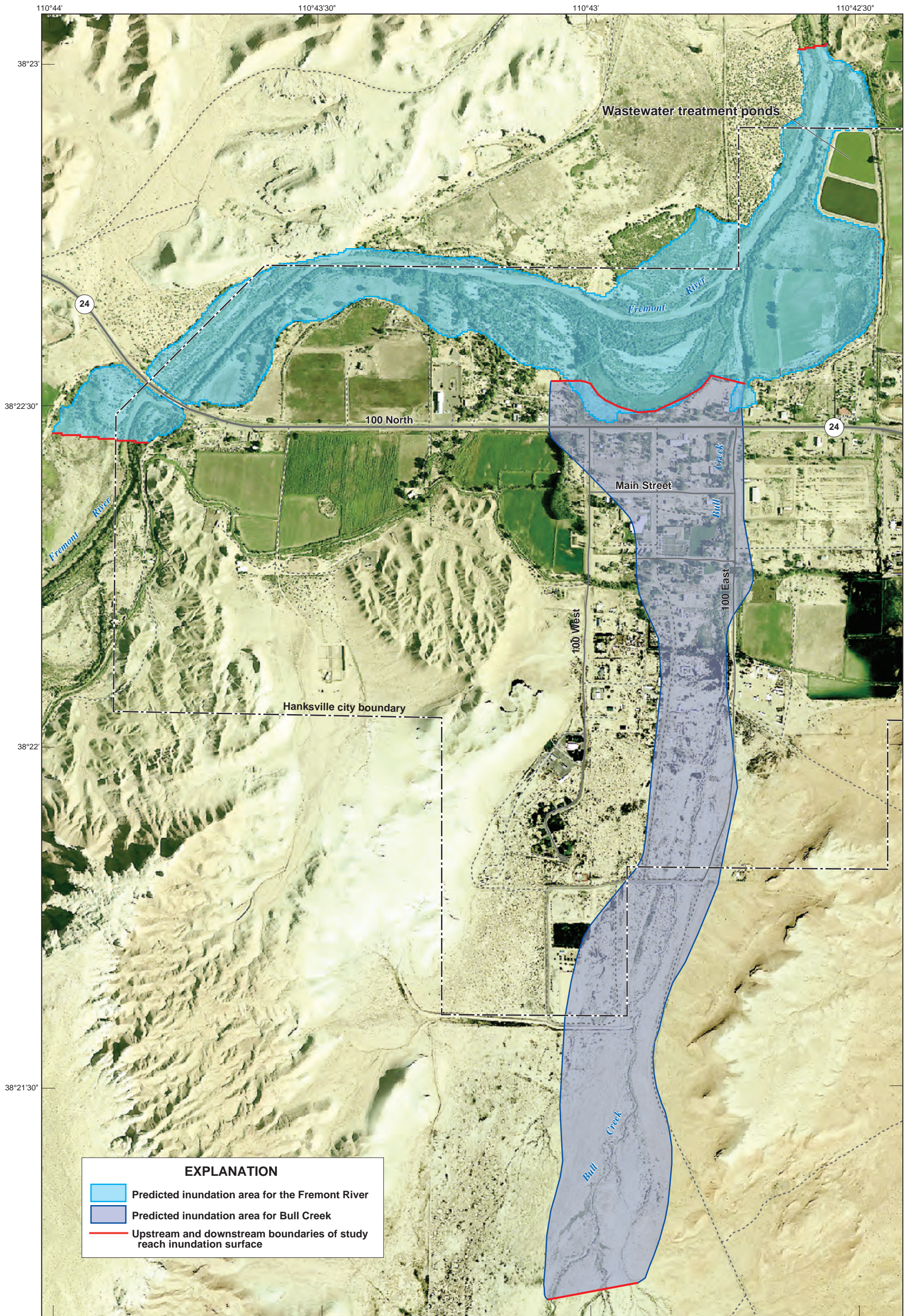
Predicted inundation associated with 1 percent chance peak streamflows for the Fremont River and Bull Creek study reaches, Hanksville, Utah
