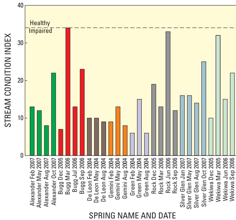
Figure 57. Stream Condition Index (SCI) values for dip net samples of macroinvertebrates collected from selected springs of the St. Johns River drainage, 2004-07. Horizontal dashed line indicates SCI value separating categories classified as “impaired” (0-34) and “healthy” (35-70) as recognized by the Florida Department of Environmental Protection (Fore and others, 2007).
