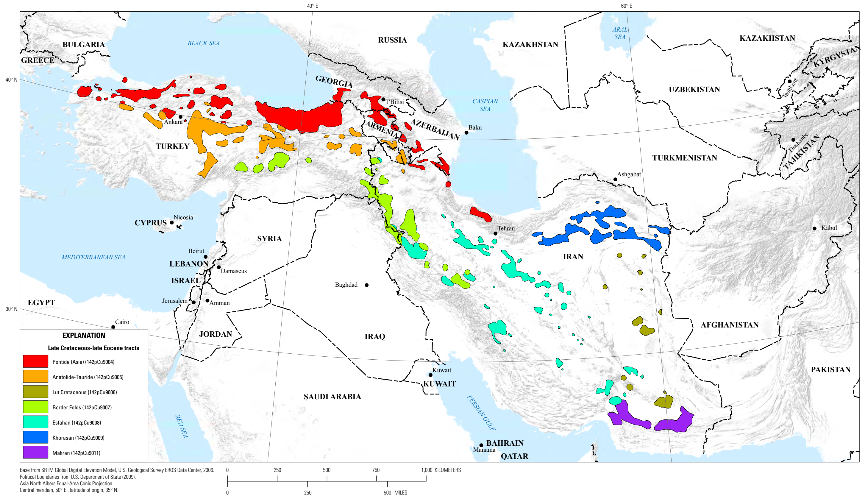
Figure 6. Late Cretaceous to late Eocene permissive tracts for porphyry copper deposits in the Tethys region of western and southern Asia.
