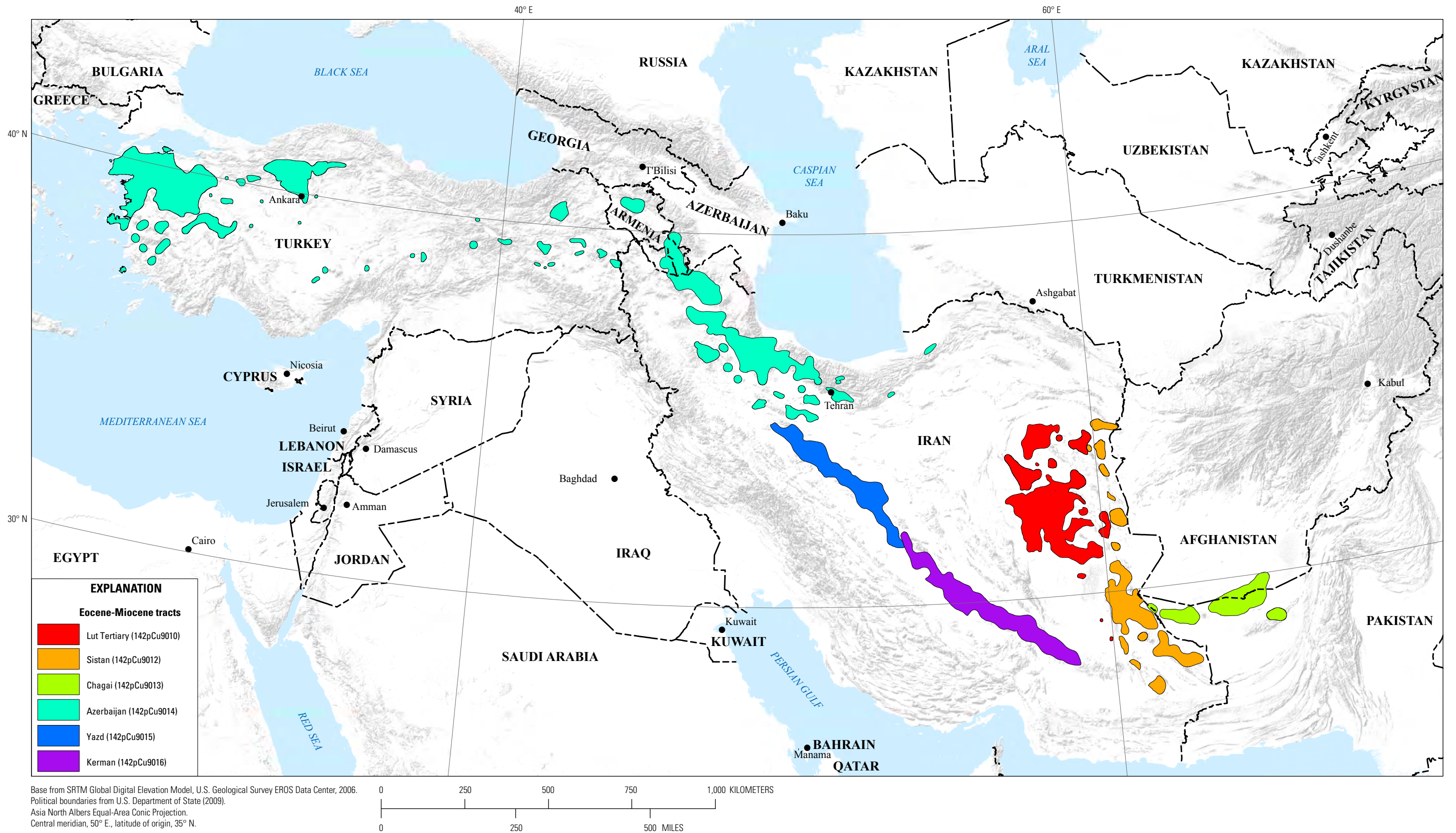
Figure 7. Eocene to Miocene permissive tracts for porphyry copper deposits in the Tethys region of western and southern Asia.
