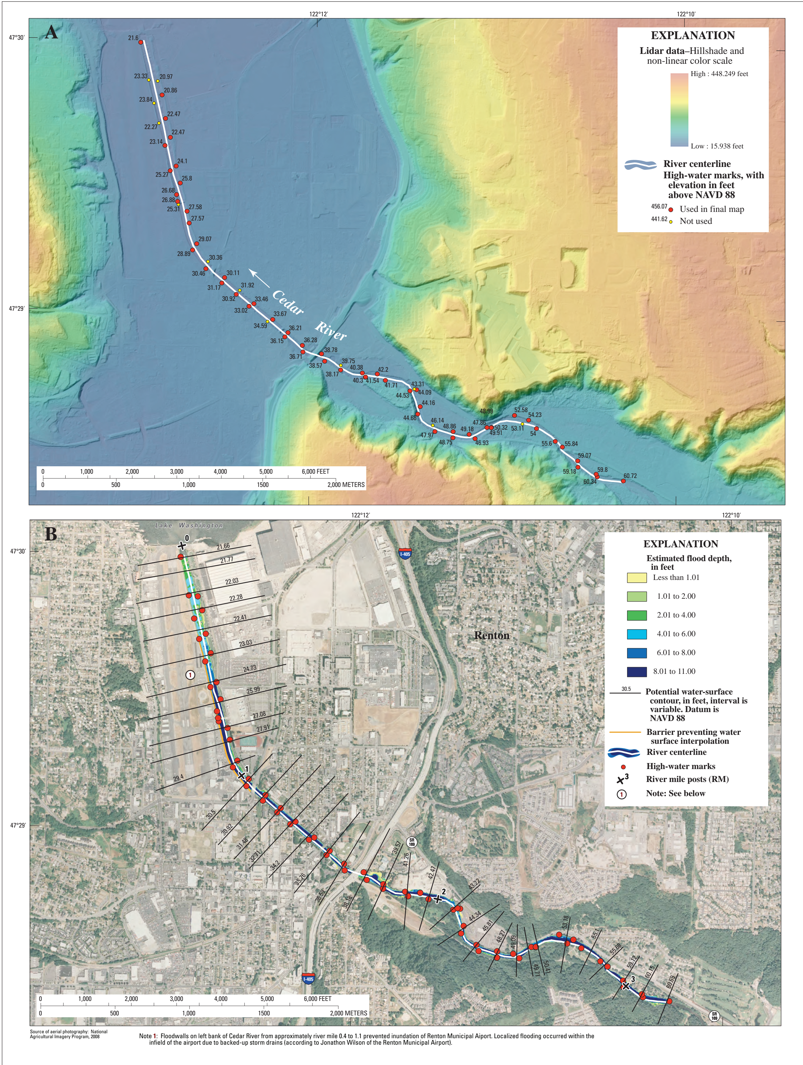
Map showing magnitude and extent of January 2009 flooding on river mile 0.1 to 3.2, Cedar River, King County, Washington.
