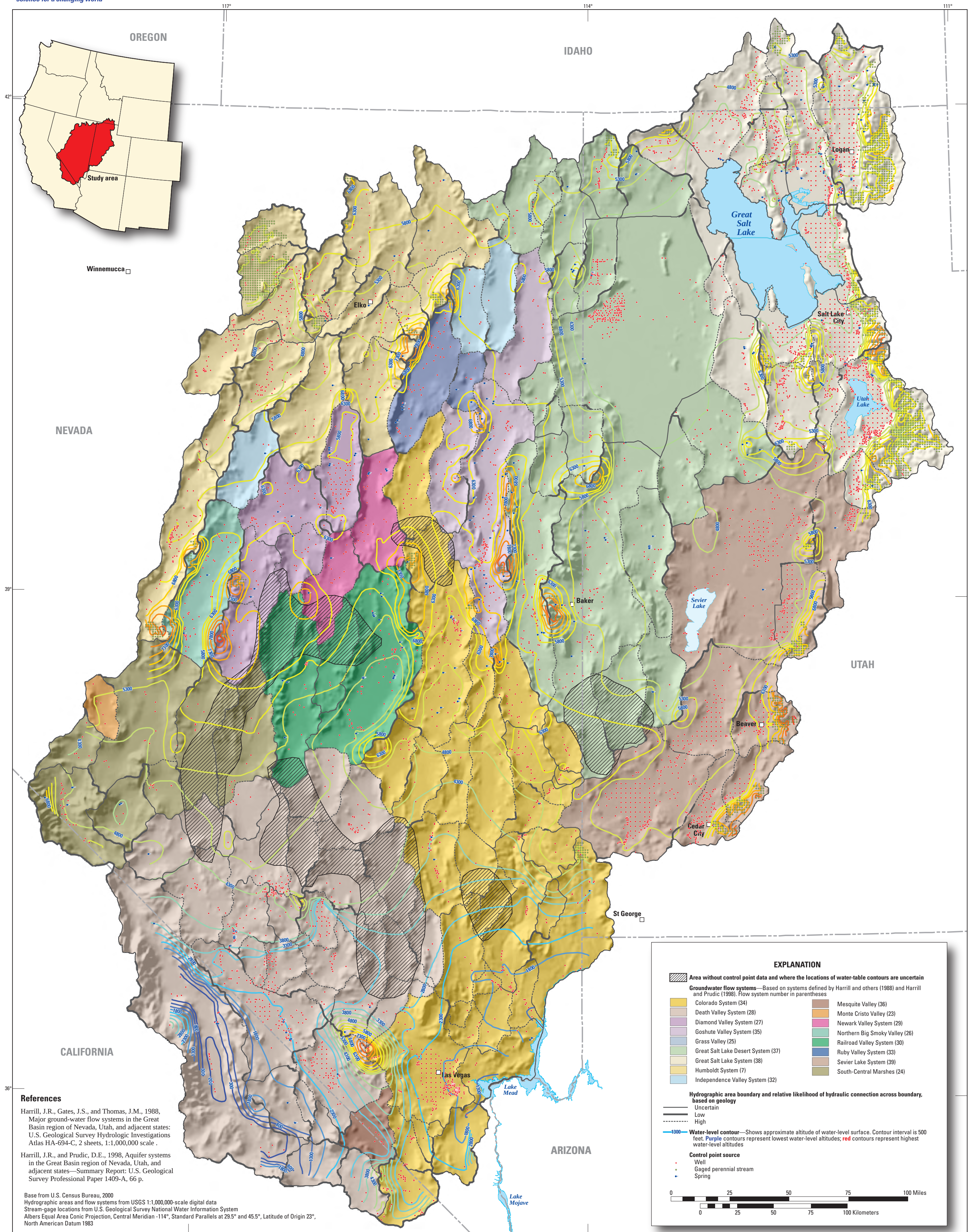
Potentiometric-Surface Map and Likelihood of Hydraulic Connections Across Hydrographic Area Boundaries of the Great Basin Carbonate and Alluvial Aquifer System Study Area
