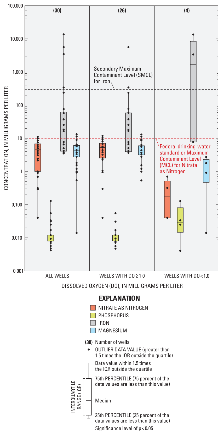
Figure 6. Distribution of nutrients (nitrate as nitrogen and total phosphorus), major ions (magnesium), and trace elements (iron) concentrations in different oxidation-reduction (redox) environments in the Columbia aquifer among the 30 public water-supply wells sampled in 2008.
