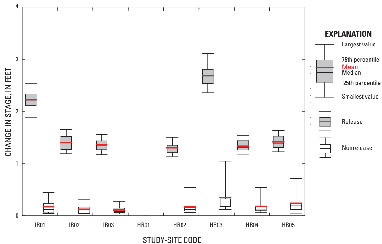
Figure 6. Change in stage at eight study sites on the Indian and Hudson Rivers, Adirondack Mountains, New York, on release and nonrelease days from July 1 to August 1, 2005. Locations of study sites are shown in figure 1; study-site codes are listed in table 1.
