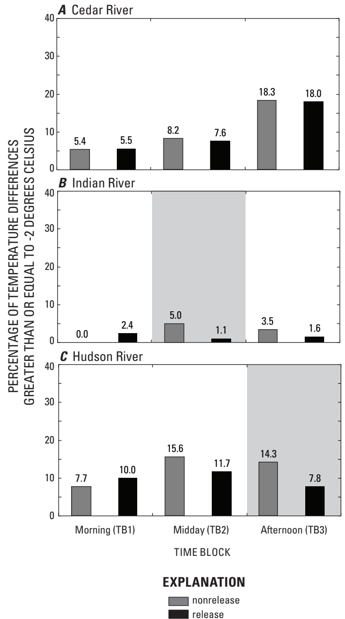
Figure 26. Percentages of temperature differences that were greater than or equal to -2^{\circ} Celsius on nonrelease and release days within time blocks TB1, TB2, and TB3 in the A , Cedar River (2006), B , Indian River (2005–06), and C , Hudson River (2005–06), Adirondack Mountains, New York. Gray backgrounds indicate time blocks when the release bubble passed through study reaches in the Indian River (TB2) and Hudson River (TB3) on release days.
