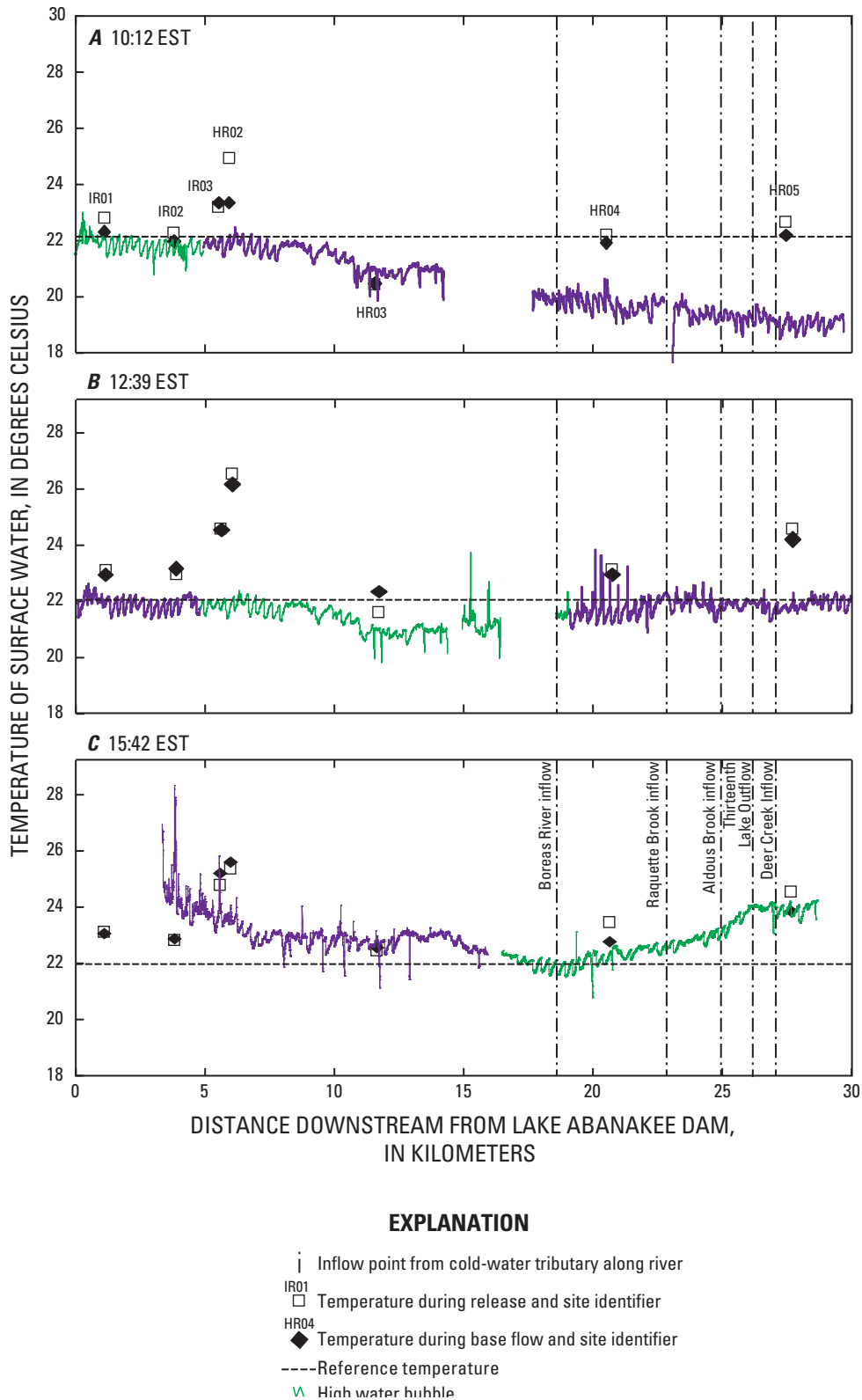
Figure 14. Longitudinal temperature profiles of the three Indian Rivers study sites IR01–IR03 and Hudson River study sites HR02–HR05 in the Adirondack Mountains, New York, at A, 10:12, B, 12:39, and C, 15:42 Eastern Standard Time (EST) during release and nonrelease flows on July 25, 2005; mean temperature at the seven study sites from July 21, 2005 through September 21, 2005, on release and nonrelease days; and inflow points for five cool-water tributaries.
