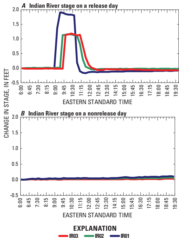
Figure 4. Change in stage at three Indian River sites A , on July 7, 2005, a release day, and B , on July 8, 2005, a nonrelease day, Adirondack Mountains, New York. Locations of study sites are shown in figure 1; study-site codes are listed in table 1.
