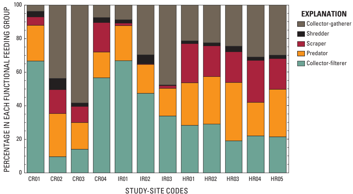
Figure 22. The percentages of macroinvertebrates in each of five functional feeding groups at 12 sites surveyed in the Cedar, Indian, and Hudson Rivers, Adirondack Mountains, New York, August 2006. Locations of study sites are shown in figure 1; study-site codes are listed in table 1.
