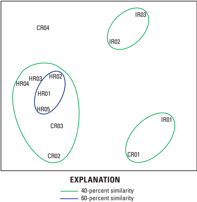
Figure 24. Ordination plot of macroinvertebrate assemblages based on square-root-transformed relative abundance data from 3 combined replicates at each of 12 sites in the Indian, Hudson, and Cedar Rivers, Adirondack Mountains, New York, August 2006. The bubbles denote significant group membership (40 and 60 percent Bray-Curtis similarity, p \leq 0.05 ) based on group-averaged cluster analysis. Locations of study sites are shown in figure 1; study-site codes are listed in table 1.
