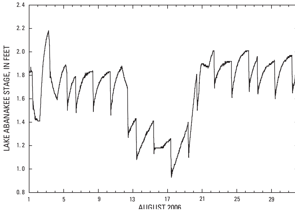
Figure 9. Lake stage at Lake Abanakee at Route 28 bridge near Indian Lake (AB02), Adirondack Mountains, New York, during August 2006. Location of AB02 is shown in figure 1; study-site code is listed in table 1.
