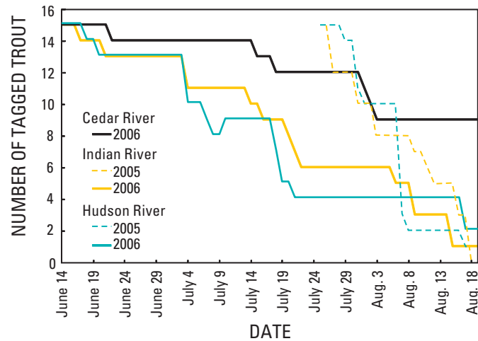
Figure 36. The number of tagged trout apparently alive each day and with the study reach in the Indian and Hudson Rivers during 2005 and 2006 and in the Cedar River during 2006, Adirondack Mountains, New York.
