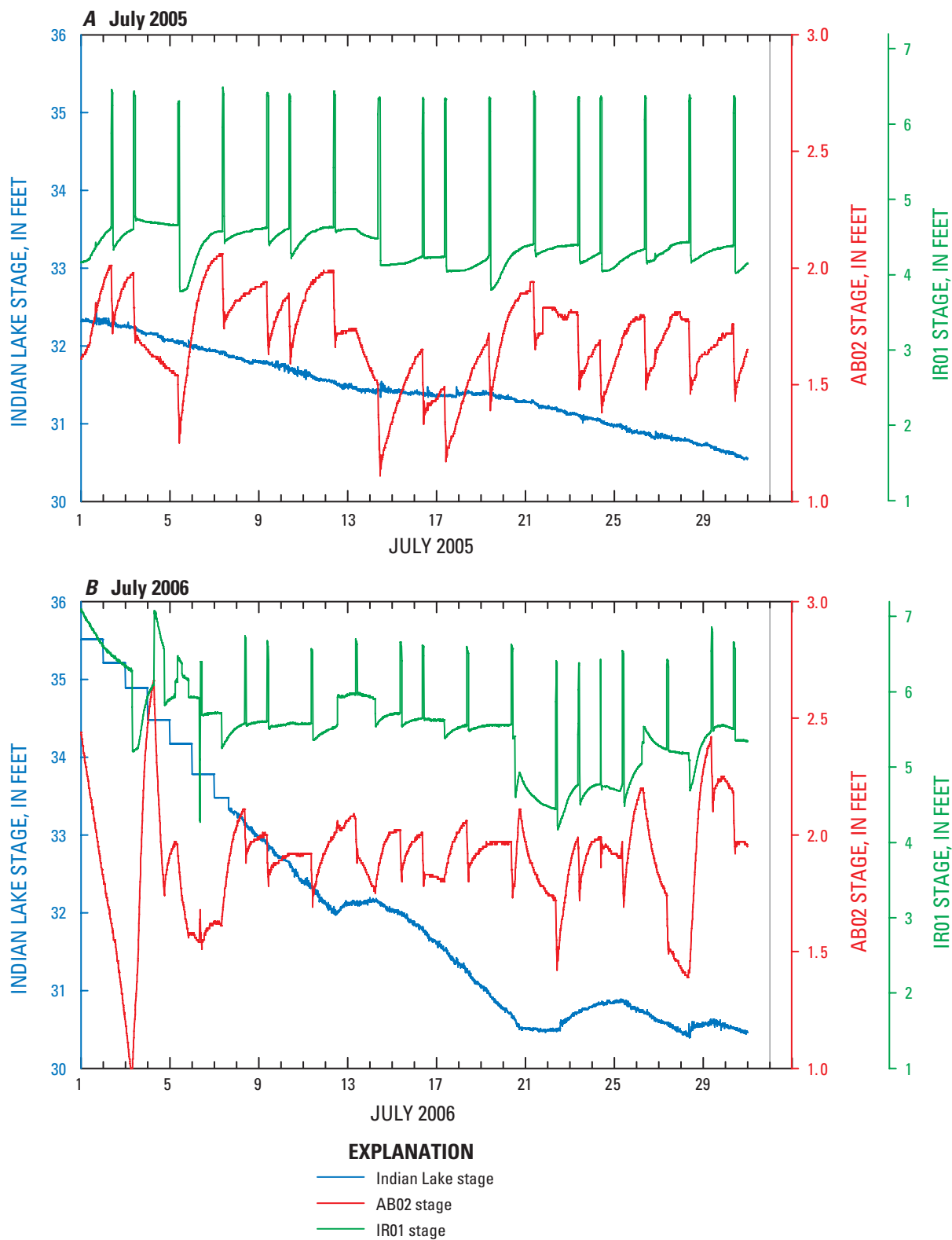
Figure 10. Stage at Indian Lake, Lake Abanakee (AB02), and Indian River (IR01), Adirondack Mountains, New York, during A , July 2005, and B , July 2006. Locations of study sites are shown in figure 1; study-site codes are listed in table 1.
