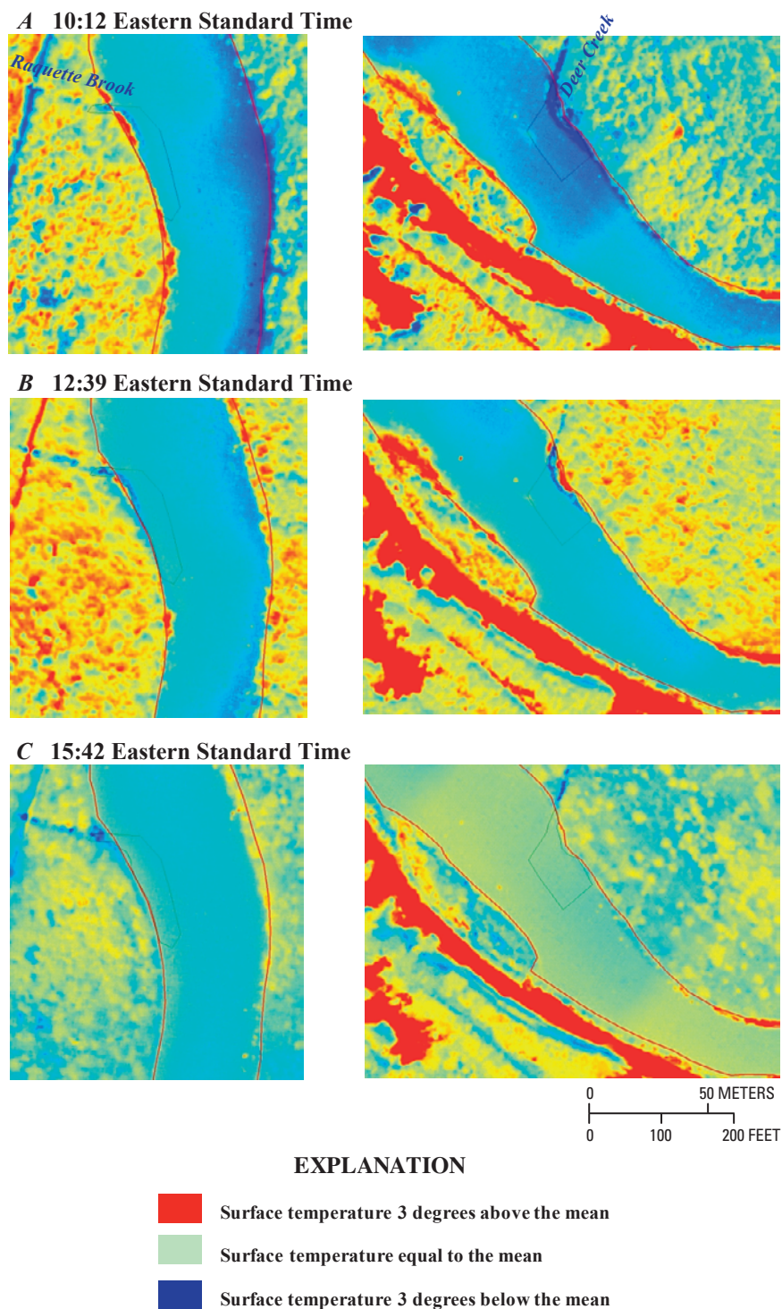
Figure 16. False-color images of the confluences of Raquette Brook at kilometer 24 and Deer Creek at kilometer 27 with the Hudson River during flights at A , 10:12, B , 12:39, and C , 15:42 Eastern Standard Time in the Adirondack Mountains, New York. The release slug passed these tributaries during the third flight, reducing any cold-water effect.
