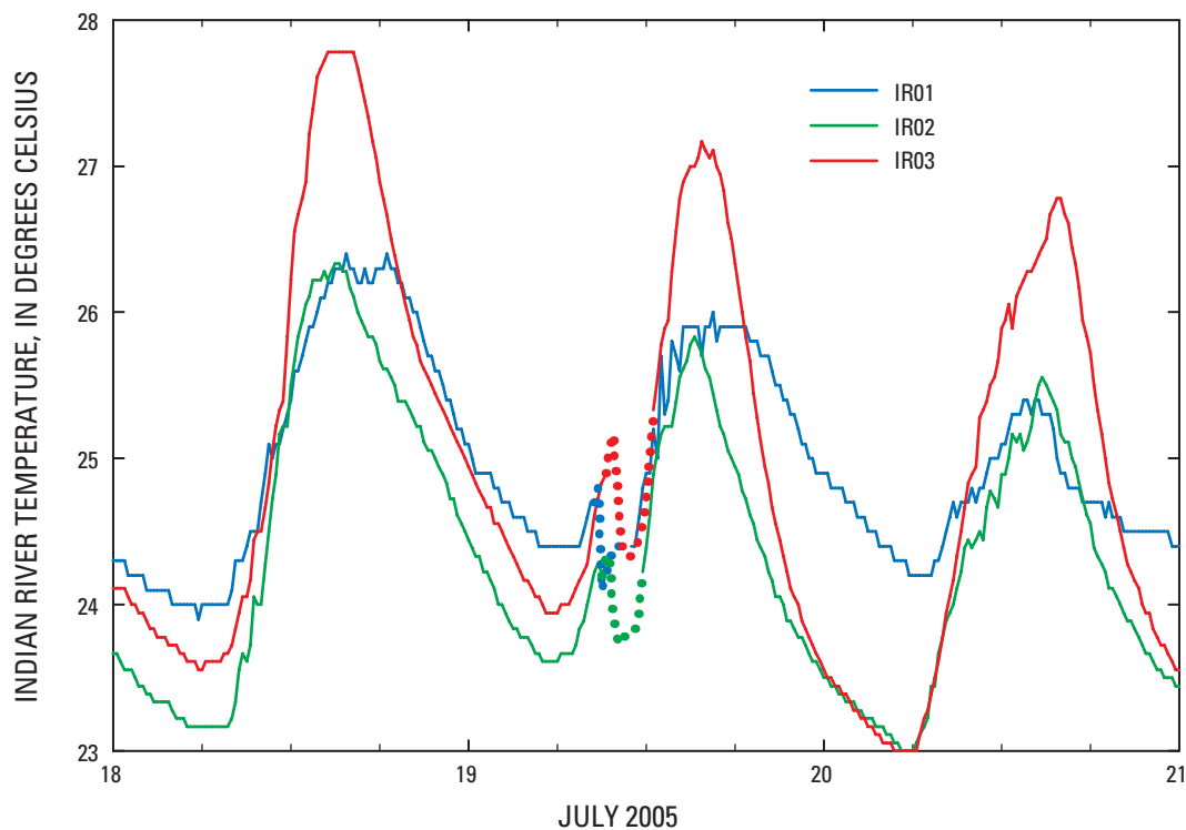
Figure 11. Change in temperature of the Indian River at three study sites in the Adirondack Mountains, New York, from July 18 to July 21, 2005. Dotted lines represent temperature recorded during a release. Locations of study sites are shown in figure 1; study-site codes are listed in table 1.
