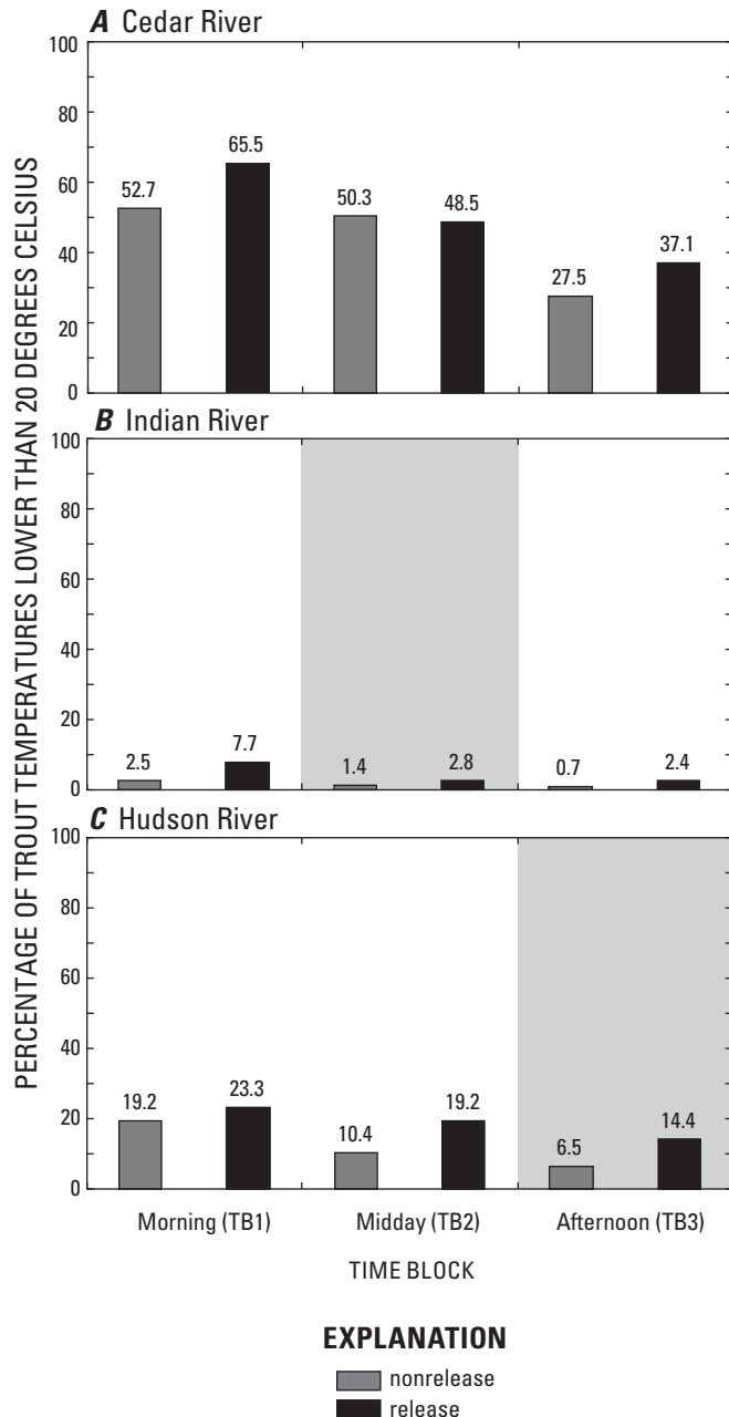
Figure 28. Percentage of observations of trout temperature lower than 20°Celsius on nonrelease and release days within time blocks TB1, TB2, and TB3 in the A , Cedar River (2006), B , Indian River (2005–06), and C , Hudson River (2005–06), Adirondack Mountains, New York. Gray backgrounds indicate time blocks when the release bubble passed through study reaches in the Indian River (TB2) and Hudson River (TB3) on release days.
