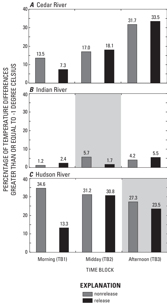
Figure 25. Percentages of temperature differences that were greater than or equal to -1^{\circ} Celsius on nonrelease days within time blocks TB1, TB2, and TB3 in the A , Cedar River (2006), B , Indian River (2005–06), and C , Hudson River (2005–06), Adirondack Mountains, New York. Gray backgrounds indicate time blocks when the release bubble passed through study reaches in the Indian River (TB2) and Hudson River (TB3) on release days.
