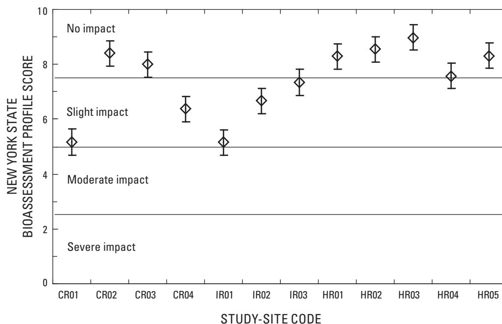
Figure 21. Average New York State Bioassessment Profile scores and 95-percent confidence intervals for Fisher's least significant difference in relation to impact categories at 12 sites surveyed in the Cedar, Indian, and Hudson Rivers, Adirondack Mountains, New York, August 2006. Locations of study sites are shown in figure 1; study-site codes are listed in table 1.
