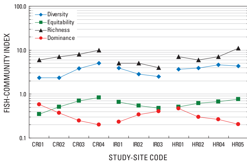
Figure 18. Diversity, equitability, richness, and dominance for fish communities at 11 study sites in the Cedar, Indian, and Hudson Rivers, Adirondack Mountains, New York, 2005–06. Locations of study sites are shown in figure 1; study-site codes are listed in table 1.
