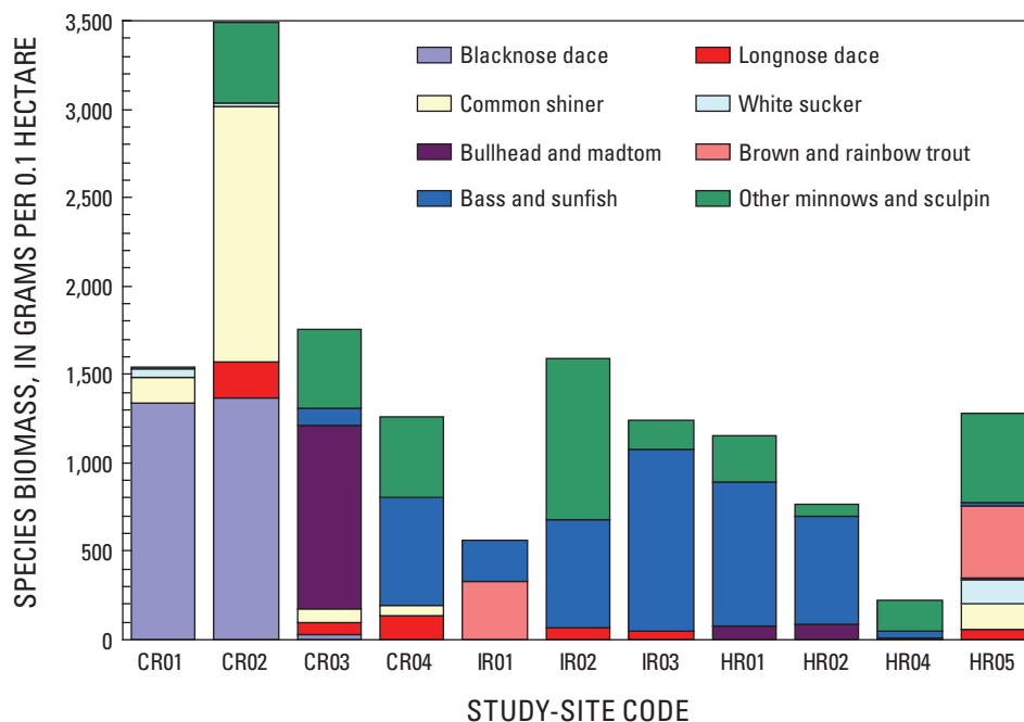
Figure 20. Biomass (grams per 0.1 hectare) of each fish or species at 11 study sites on the Cedar, Indian, and Hudson Rivers, Adirondack Mountains, New York, 2005–06. Locations of study sites are shown in figure 1; study-site codes are listed in table 1.
