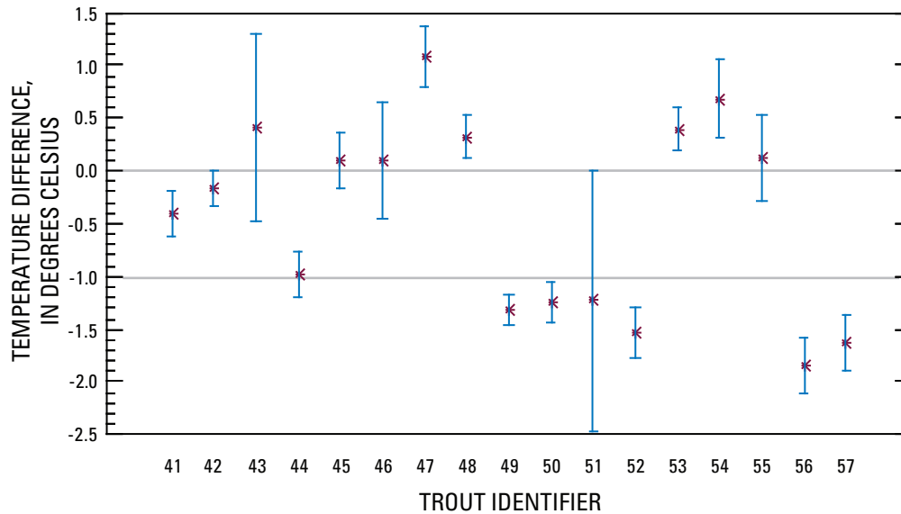
Figure 27. Average differences between trout and river temperatures and standard errors for all observations of 17 trout tracked in the Hudson River, Adirondack Mountains, New York, during 2006. Trout identifier refers to the last two digits of the frequency of each implanted transmitter.
