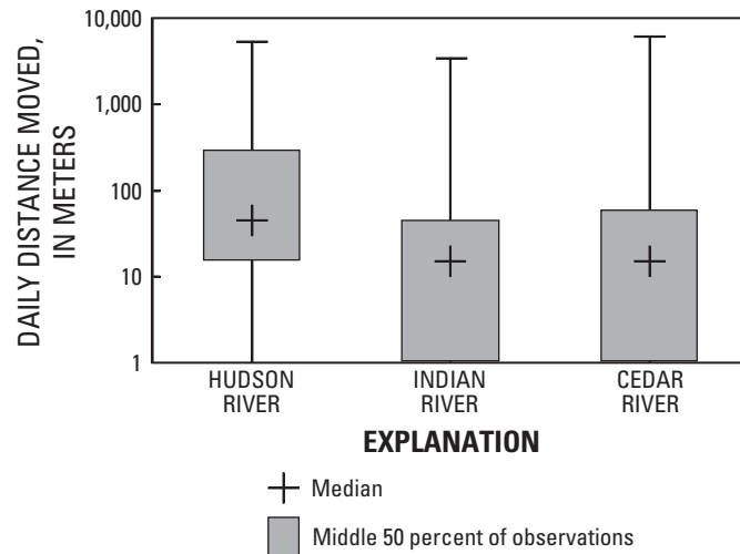
Figure 34. Summary of brown-trout activity (distance trout moved between consecutive days) in the Cedar, Indian, and Hudson Rivers, Adirondack Mountains, New York, during 2006.
