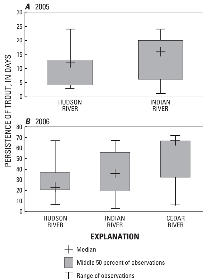
Figure 35. Persistence of brown trout (number of days trout were apparently alive and within the study reach) in the Cedar, Indian, and Hudson Rivers, Adirondack Mountains, New York, during A, 2005, and B, 2006.
