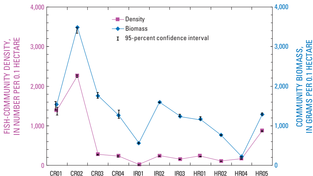
Figure 17. Estimates of density, biomass, and 95-percent confidence intervals for fish communities surveyed at 11 study sites on the Cedar, Indian, and Hudson Rivers, Adirondack Mountains, New York, 2005–06. Locations of study sites are shown in figure 1; study-site codes are listed in table 1.
