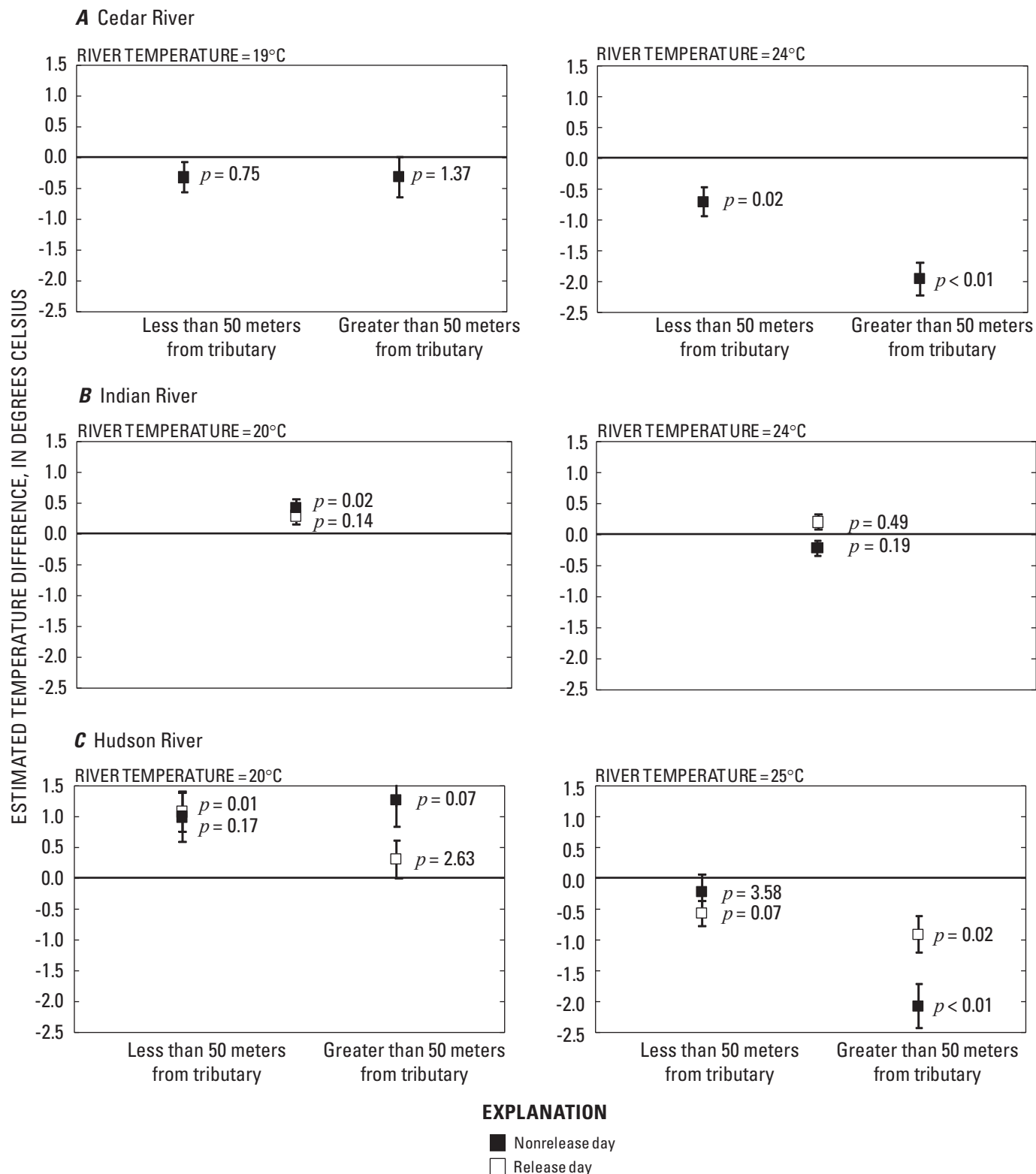
Figure 29. Estimated least-square mean temperature differences and standard errors calculated from the best supported multilevel model for the A , Cedar and B , Indian Rivers, Adirondack Mountains, New York, during the afternoon time block (TB3), and the C , Hudson River during the midday time block (TB2) during 2006. Interactions terms, denoted by multiple estimates, included river temperature and (or) release day and proximity to tributaries. The results of significance tests comparing temperature differences with zeros are indicated by p -values next to each symbol. <, less than
