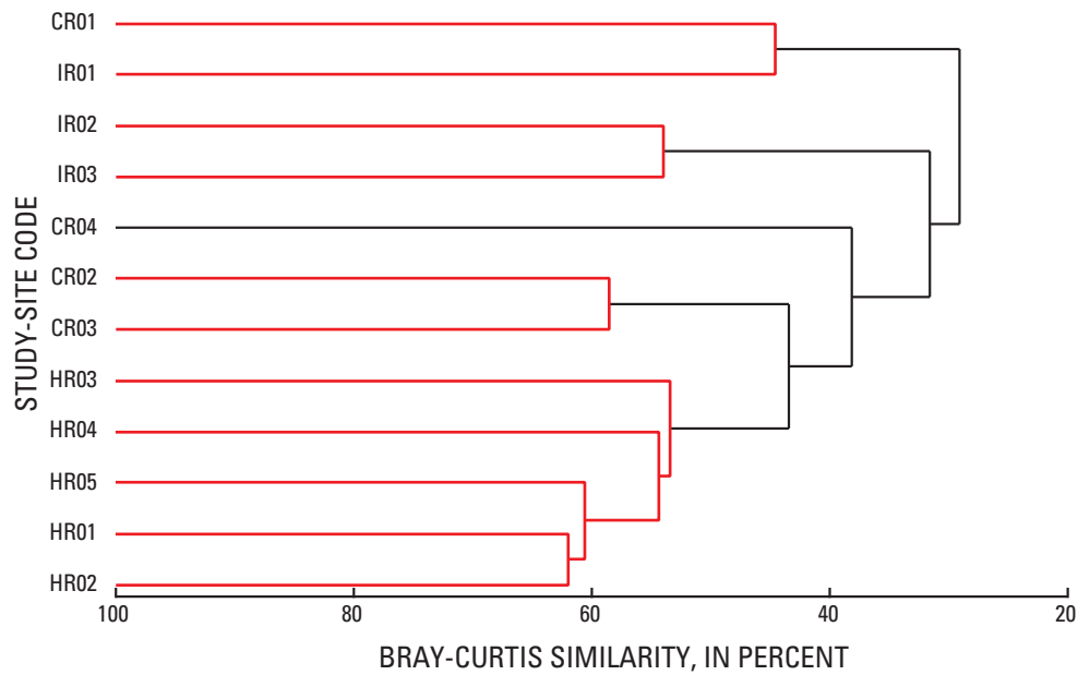
Figure 23. Cluster analysis of Bray-Curtis similarities for macroinvertebrate assemblages based on square-root-transformed relative abundance data from 3 combined replicates collected at each of 12 sites in the Cedar, Indian, and Hudson Rivers, Adirondack Mountains, New York, August 2006. The red links identify sites at which replicates did not differ significantly ( p \leq 0.05 ) from each other. Locations of study sites are shown in figure 1; study-site codes are listed in table 1.
