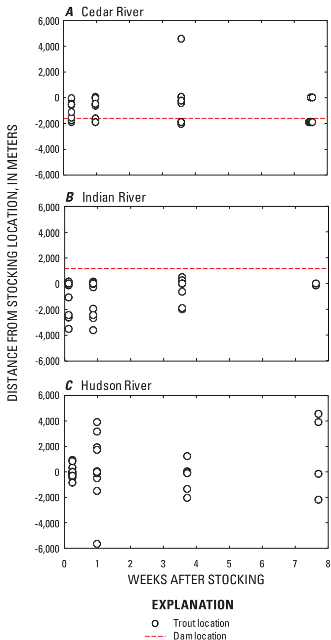
Figure 31. Dispersal of individual brown trout upstream (positive) and downstream (negative) from stocking locations in the A, Cedar, B, Indian, and C, Hudson Rivers, Adirondack Mountains, New York, at approximately 1, 7, 30, and 60 days after stocking during 2006.
