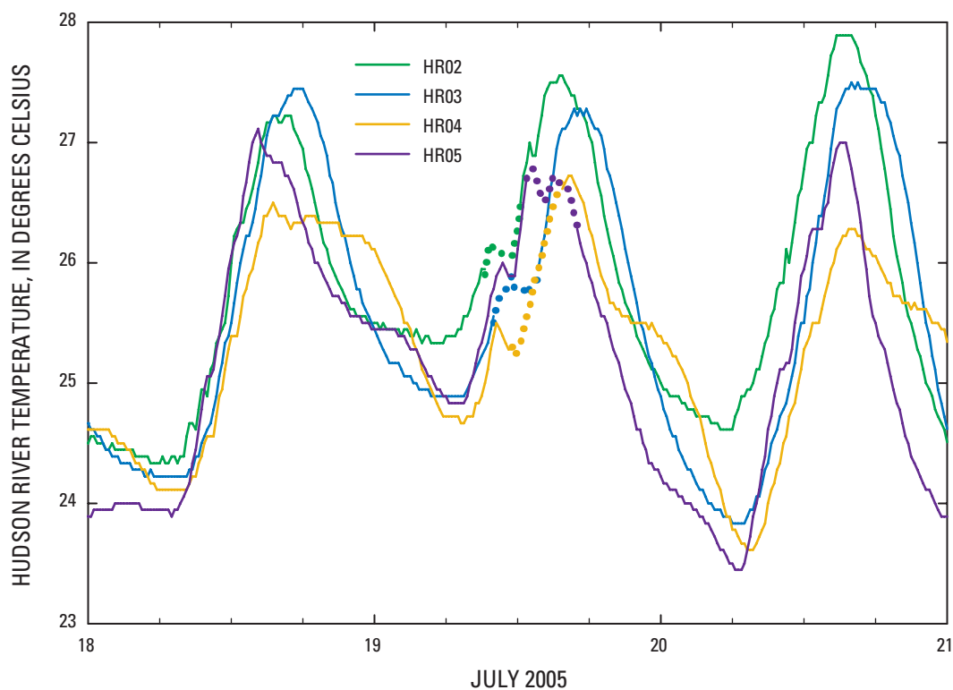
Figure 12. Change in temperature of the Hudson River at four sites, in the Adirondack Mountains, New York, from July 18 to July 21, 2005. Dotted lines represent temperatures recorded during a release. Locations of study sites are shown in figure 1; study-site codes are listed in table 1.
