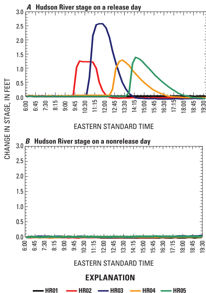
Figure 5. Change in stage at five Hudson River sites A , on July 7, 2005, a release day, and B , on July 8, 2005, a nonrelease day, Adirondack Mountains, New York. Locations of study sites are shown in figure 1; study-site codes are listed in table 1.
