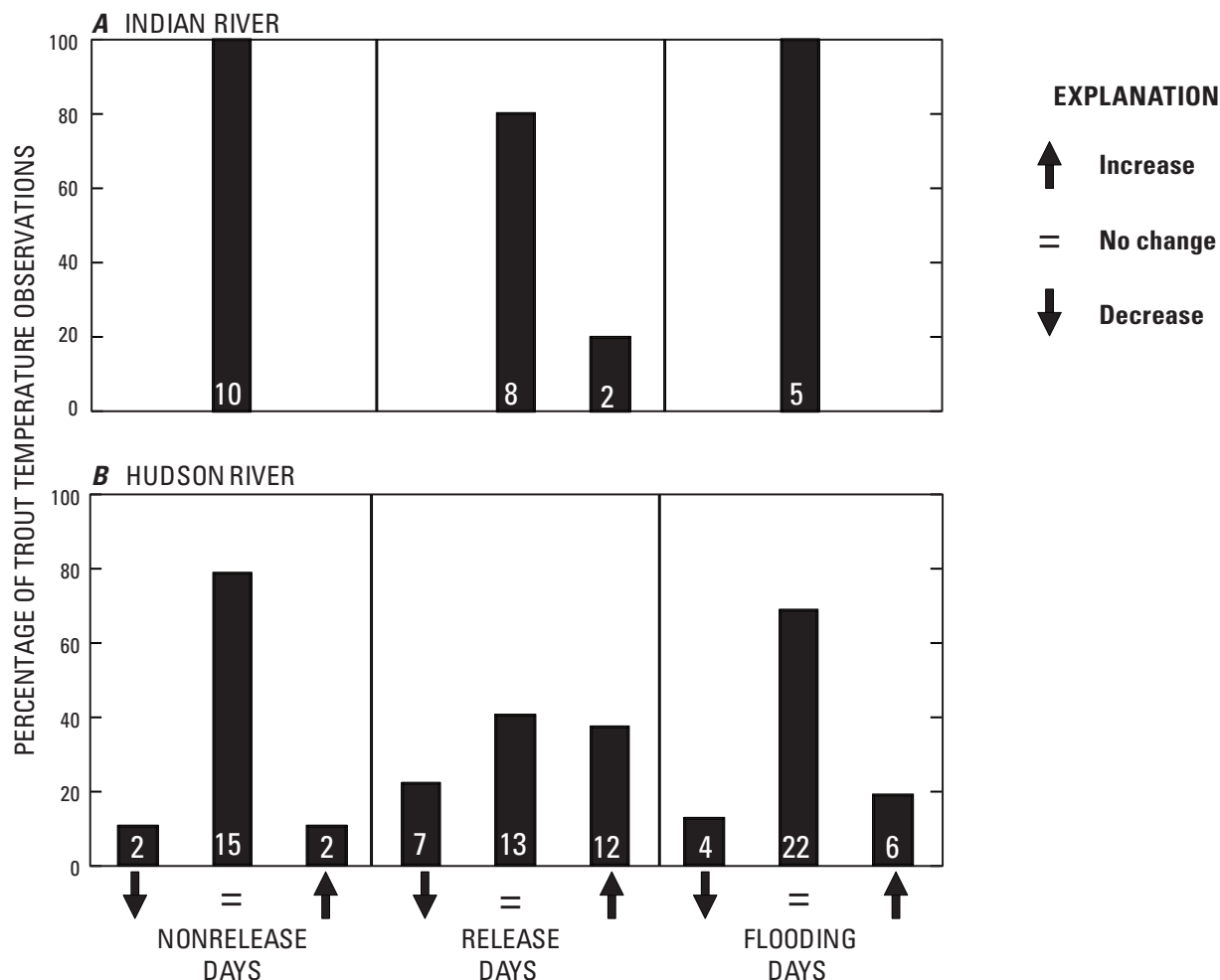
Figure 30. Percentage (and number) of trout temperatures that increased, stayed the same, or decreased over the time span when release bubbles arrived at the trout's location on nonrelease, release, and flooding days in the A , Indian River and B , Hudson River, Adirondack Mountains, New York, during 2006.
