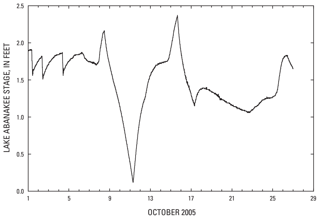
Figure 7. Lake stage at Lake Abanakee at Route 28 bridge near Indian Lake (AB02), Adirondack Mountains, New York, during October 2005. Location of AB02 is shown in figure 1; study-site codes are listed in table 1.
