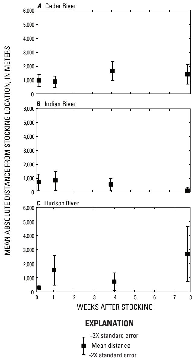
Figure 32. Mean absolute distance ( \pm 2 \times standard error) of all brown trout from the stocking locations in the A , Cedar, B , Indian, and C , Hudson Rivers, Adirondack Mountains, New York, at approximately 1, 7, 30, and 60 days after stocking during 2006.
