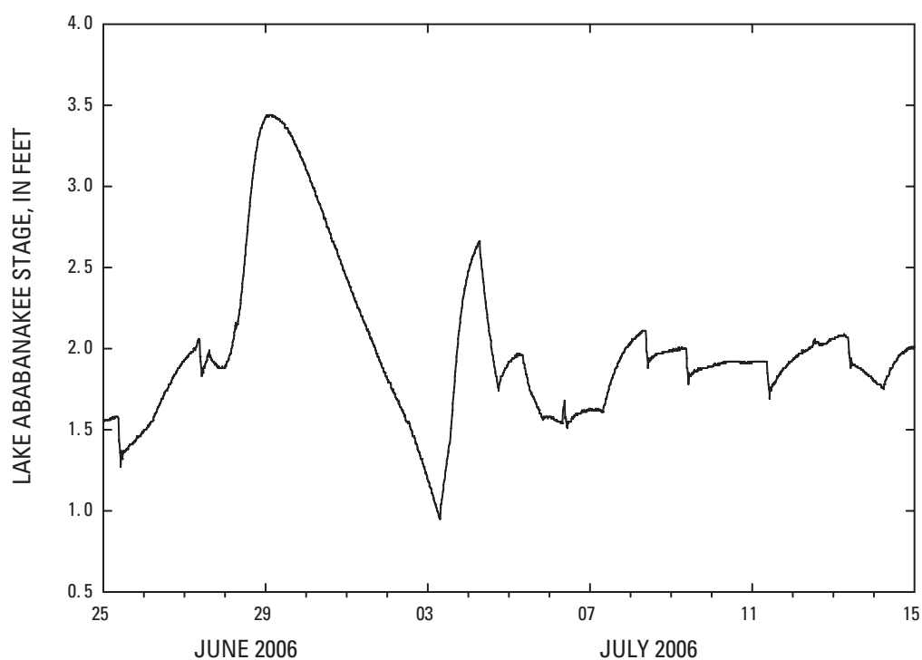
Figure 8. Lake stage at Lake Abanakee at Route 28 bridge near Indian Lake (AB02), Adirondack Mountains, New York, during June and July 2006. Location of AB02 is shown in figure 1; study-site codes are listed in table 1.
