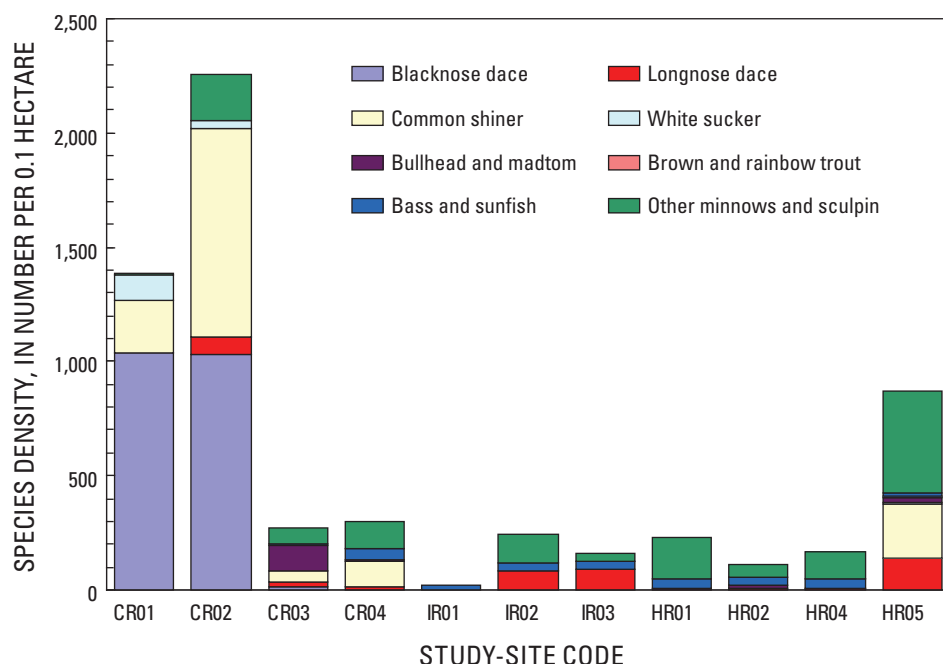
Figure 19. Density (number of fish per 0.1 hectare) of each fish group or species at 11 study sites on the Indian, Hudson, and Cedar Rivers, Adirondack Mountains, New York, 2005–06. Locations of study sites are shown in figure 1; study-site codes are listed in table 1.
