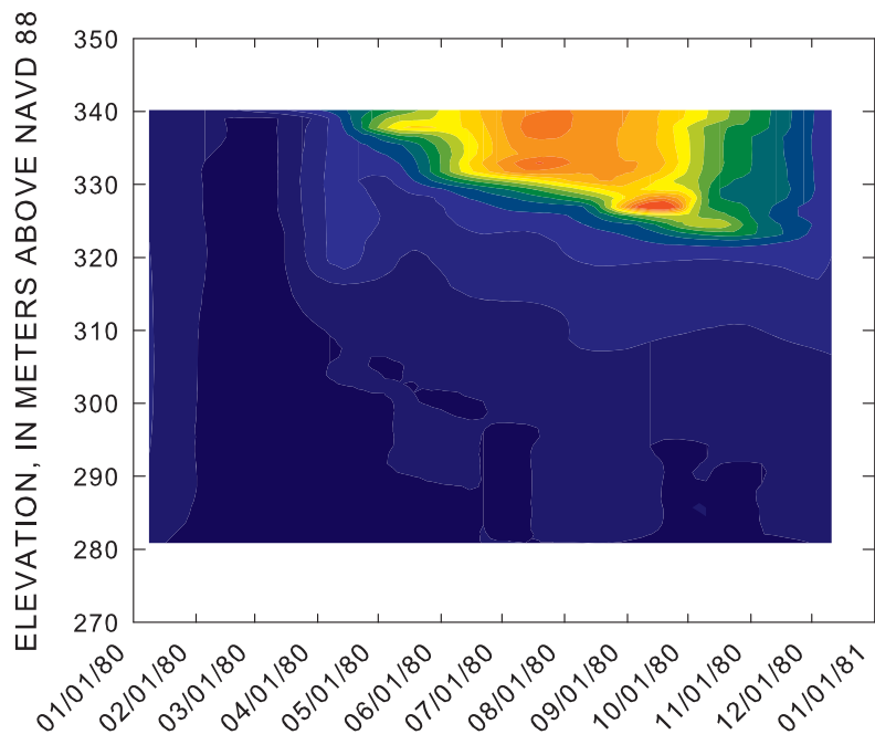
TIME-DEPTH DISTRIBUTION OF TEMPERATURE NEAR BEAVER LAKE DAM.
