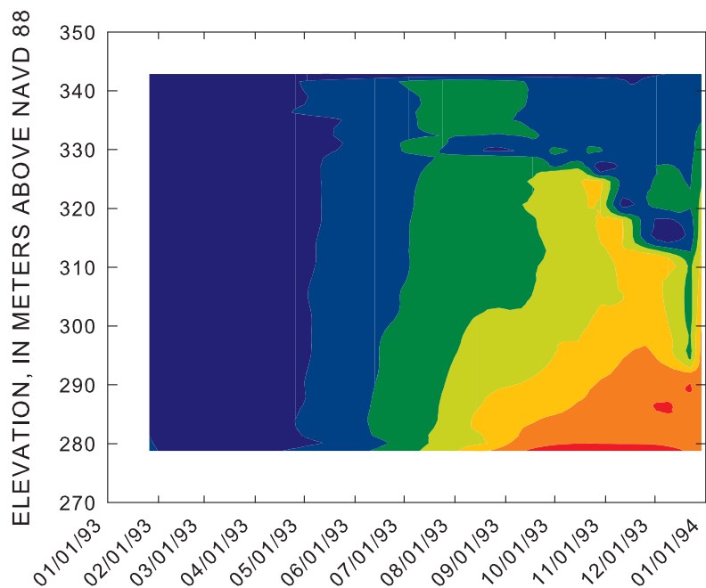
TIME-DEPTH DISTRIBUTION OF DISSOLVED OXYGEN NEAR BEAVER LAKE DAM.
