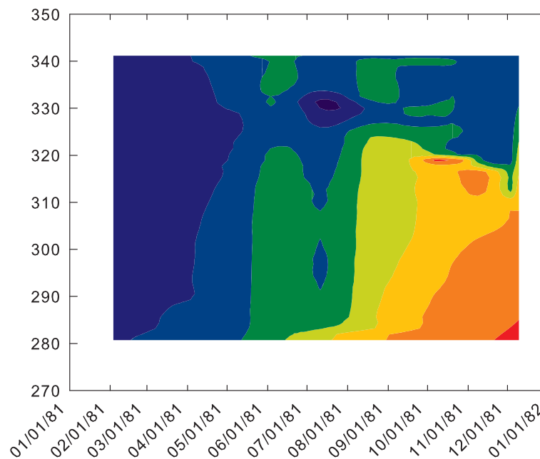
TIME-DEPTH DISTRIBUTIO OF DISSOLVED OXYGEN NEAR BEAVER LAKE DAM.
