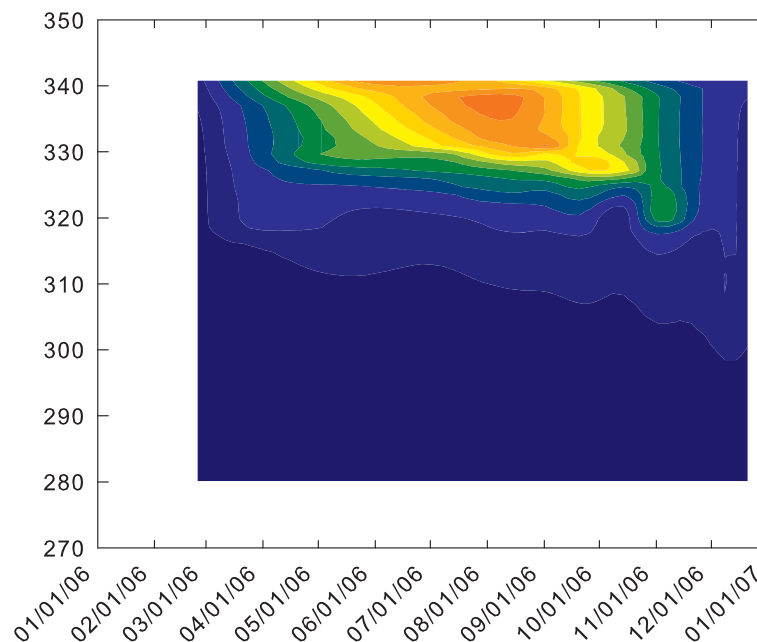
TIME-DEPTH DISTRIBUTION OF TEMPERATURE NEAR BEAVER LAKE DAM.
