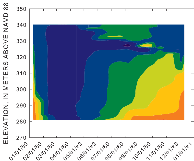
TIME-DEPTH DISTRIBUTIO OF DISSOLVED OXYGEN NEAR BEAVER LAKE DAM.
