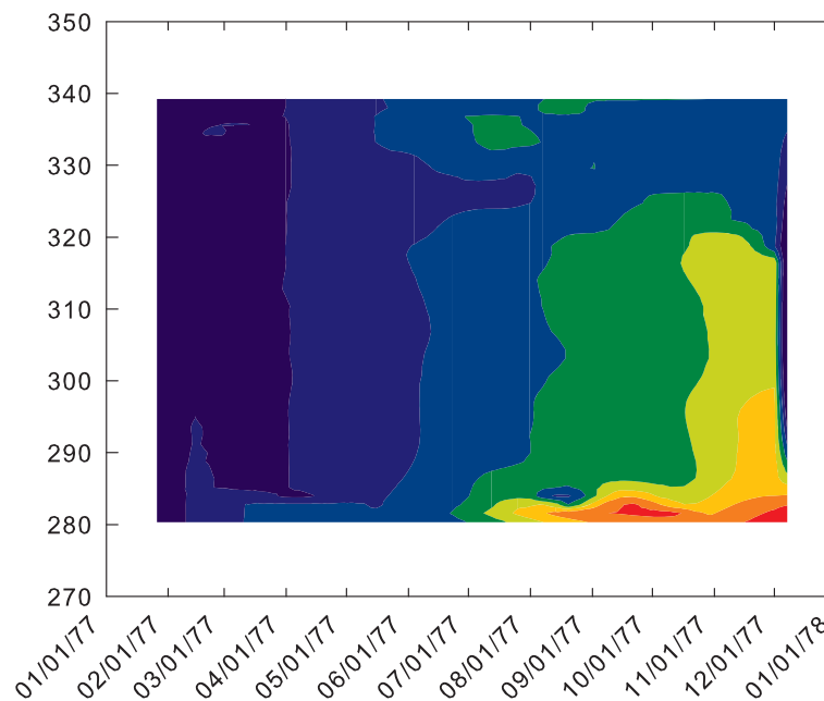
TIME-DEPTH DISTRIBUTION OF DISSOLVED OXYGEN NEAR BEAVER LAKE DAM.
