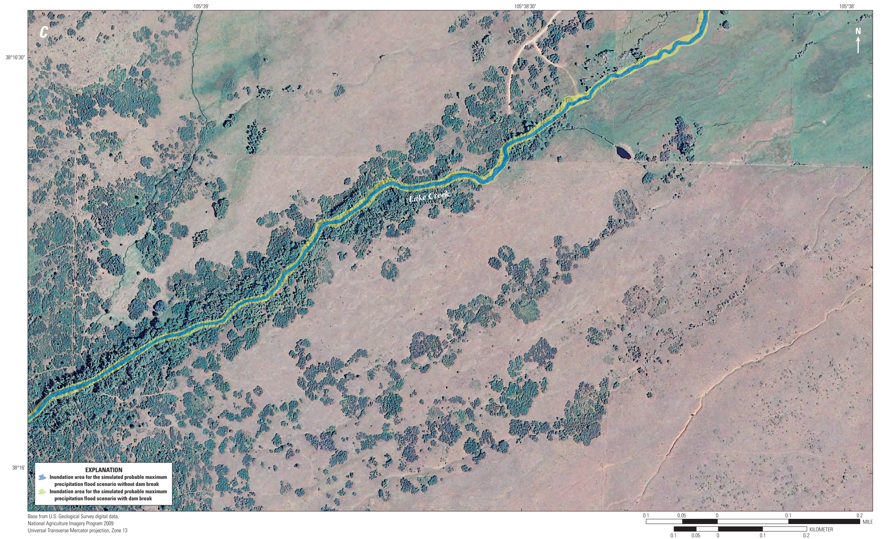
Figure 20. Flood inundation map for a simulated dam breach at Balman Reservoir from a probable maximum precipitation, 24-hour inflow design flood in six stream reaches (A), (B), (C), (D), (E), and (F), southeast to northeast.—Continued
