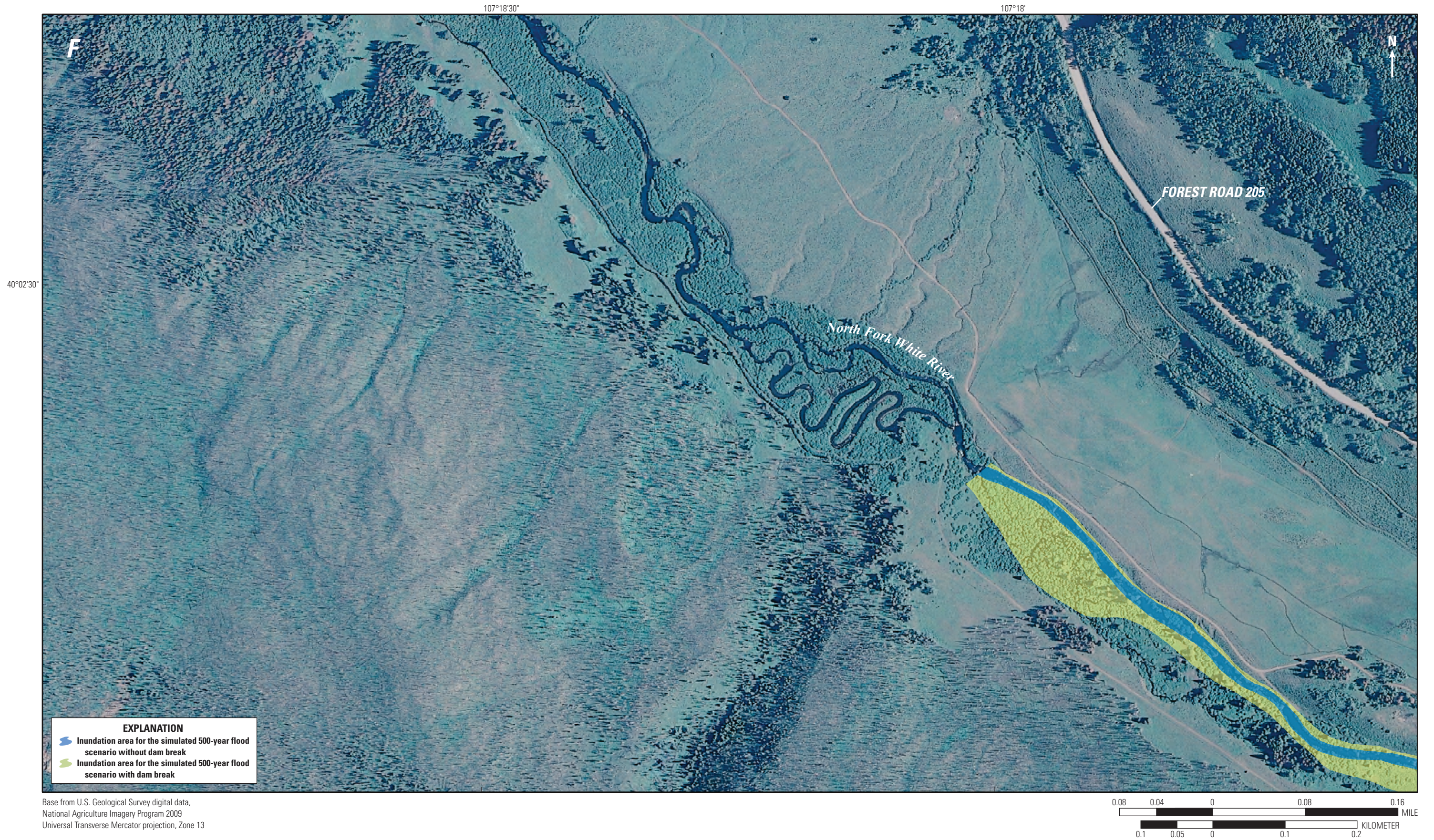
Figure 28. Flood inundation map for a simulated dam breach at McGinnis Lake from a 500-year, 24-hour inflow design flood in six stream reaches (A), (B), (C), (D), (E), and (F), east to northwest.—Continued
