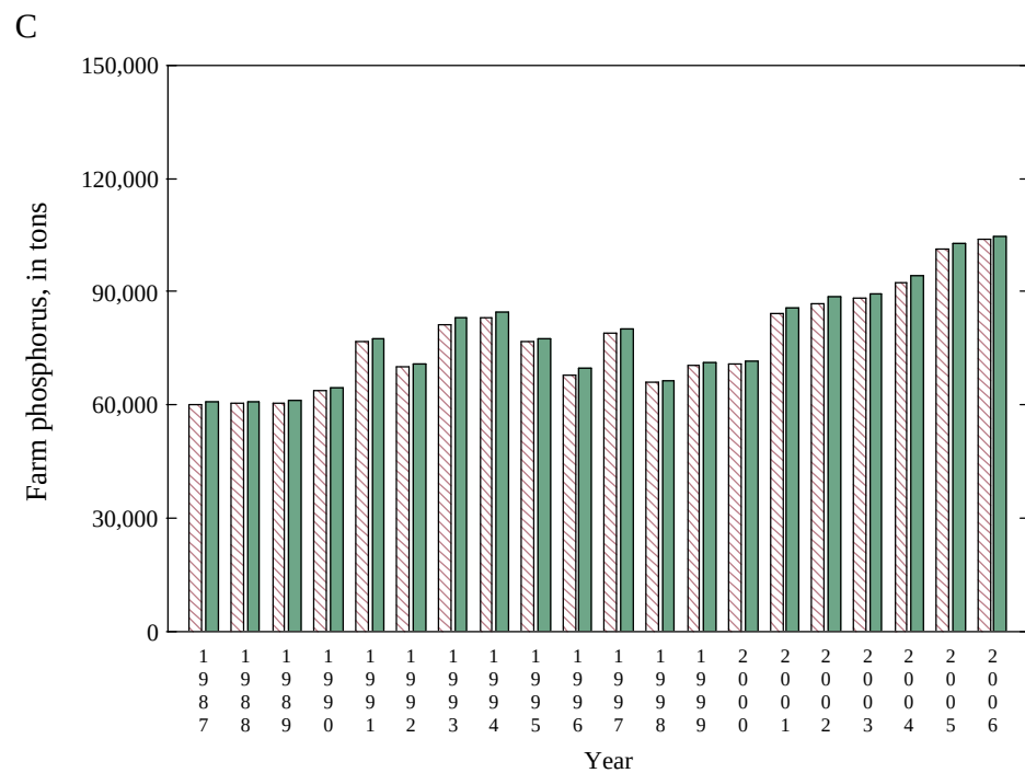
Appendix 6 Figure 23. Nitrogen and phosphorus tonnage based on national (red) and state (green) farm and nonfarm proportions for North Dakota
