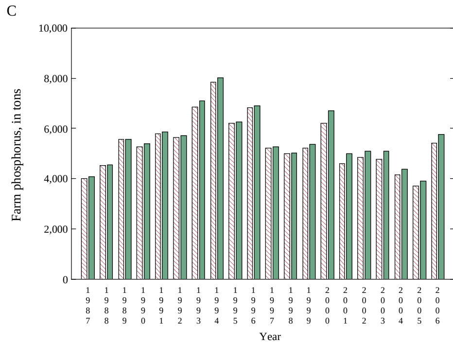
Appendix 6 Figure 21. Nitrogen and phosphorus tonnage based on national (red) and state (green) farm and nonfarm proportions for New Mexico
