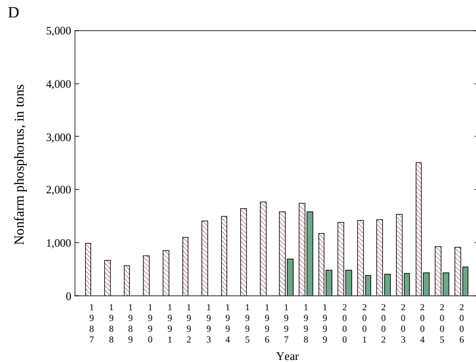
Appendix 6 Figure 9. Nitrogen and phosphorus tonnage based on national (red) and state (green) farm and nonfarm proportions for Kentucky
