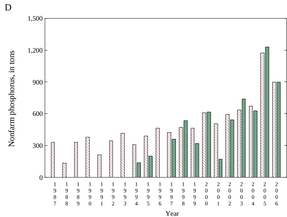
Appendix 6 Figure 4. Nitrogen and phosphorus tonnage based on national (red) and state (green) farm and nonfarm proportions for Connecticut
