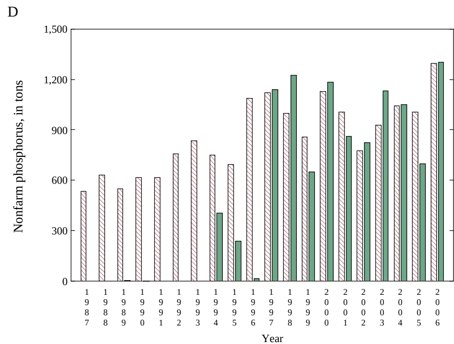
Appendix 6 Figure 13. Nitrogen and phosphorus tonnage based on national (red) and state (green) farm and nonfarm proportions for Massachusetts
