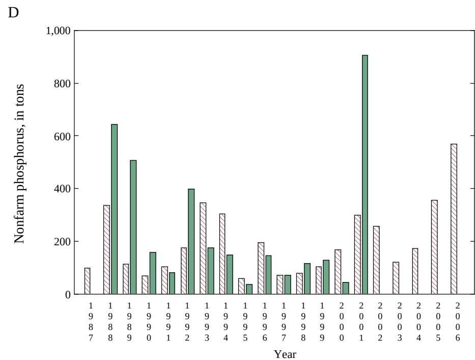
Appendix 6 Figure 1. Nitrogen and phosphorus tonnage based on national (red) and state (green) farm and nonfarm proportions for Arizona
