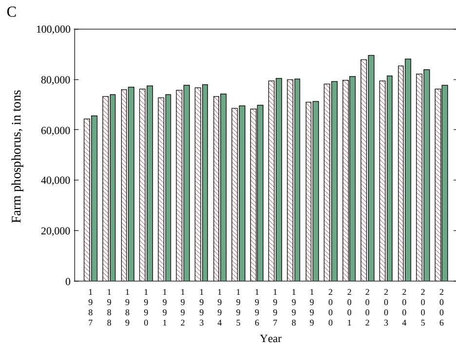
Appendix 6 Figure 16. Nitrogen and phosphorus tonnage based on national (red) and state (green) farm and nonfarm proportions for Missouri
