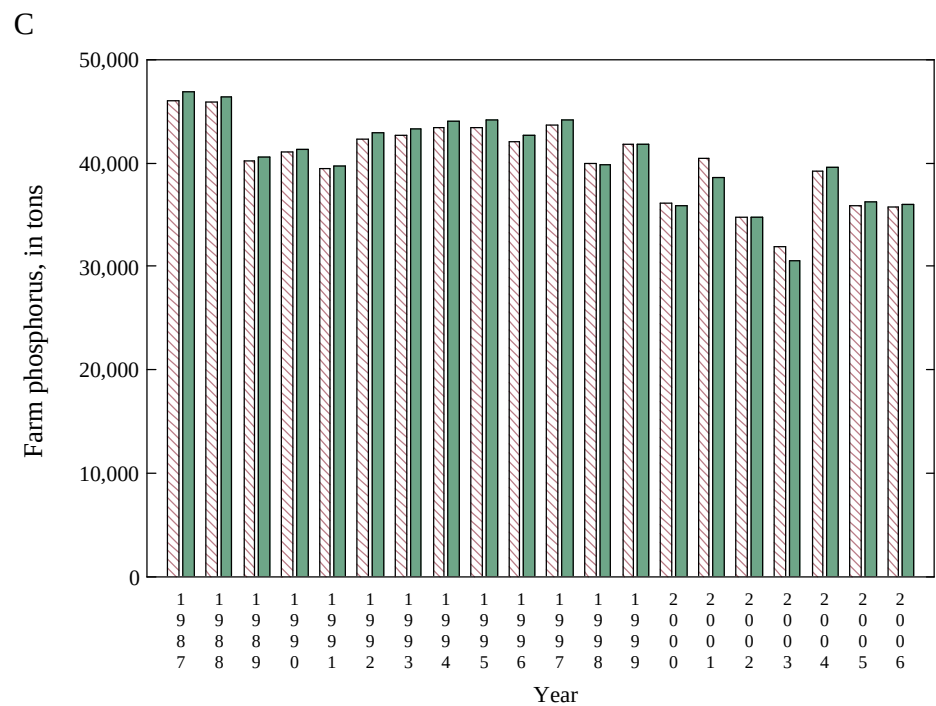
Appendix 6 Figure 29. Nitrogen and phosphorus tonnage based on national (red) and state (green) farm and nonfarm proportions for Tennessee
