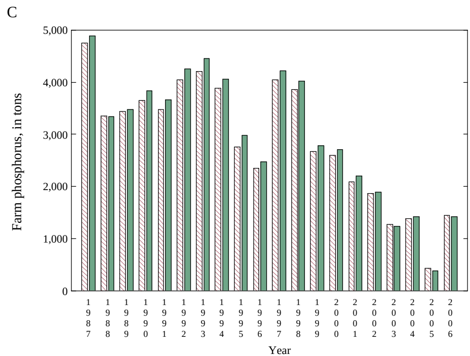
Appendix 6 Figure 34. Nitrogen and phosphorus tonnage based on national (red) and state (green) farm and nonfarm proportions for West Virginia
