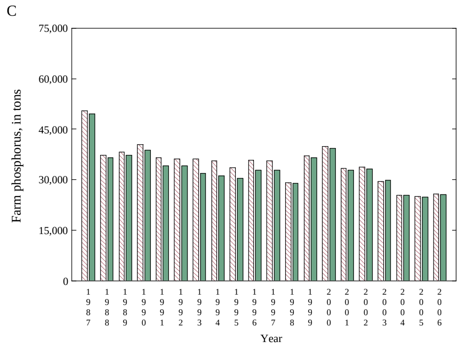
Appendix 6 Figure 6. Nitrogen and phosphorus tonnage based on national (red) and state (green) farm and nonfarm proportions for Florida
