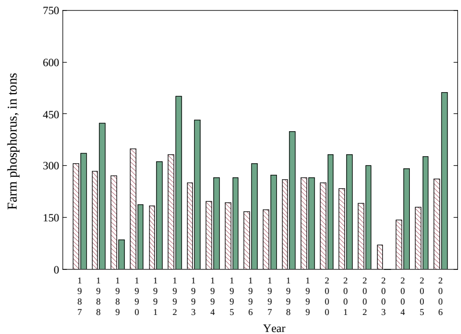
Appendix 6 Figure 27. Nitrogen and phosphorus tonnage based on national (red) and state (green) farm and nonfarm proportions for Rhode Island
