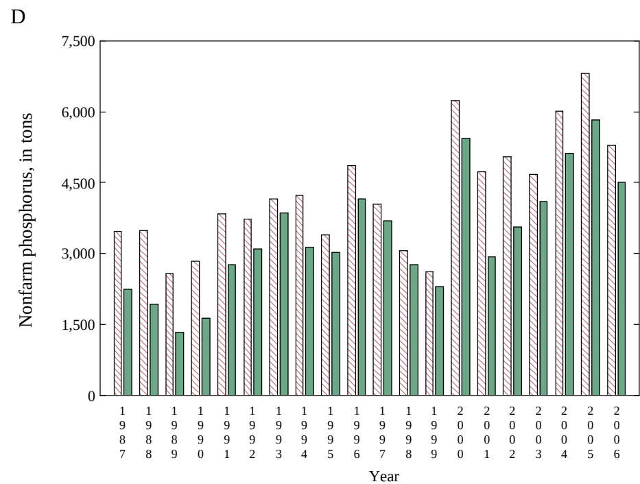
Appendix 6 Figure 2. Nitrogen and phosphorus tonnage based on national (red) and state (green) farm and nonfarm proportions for California
