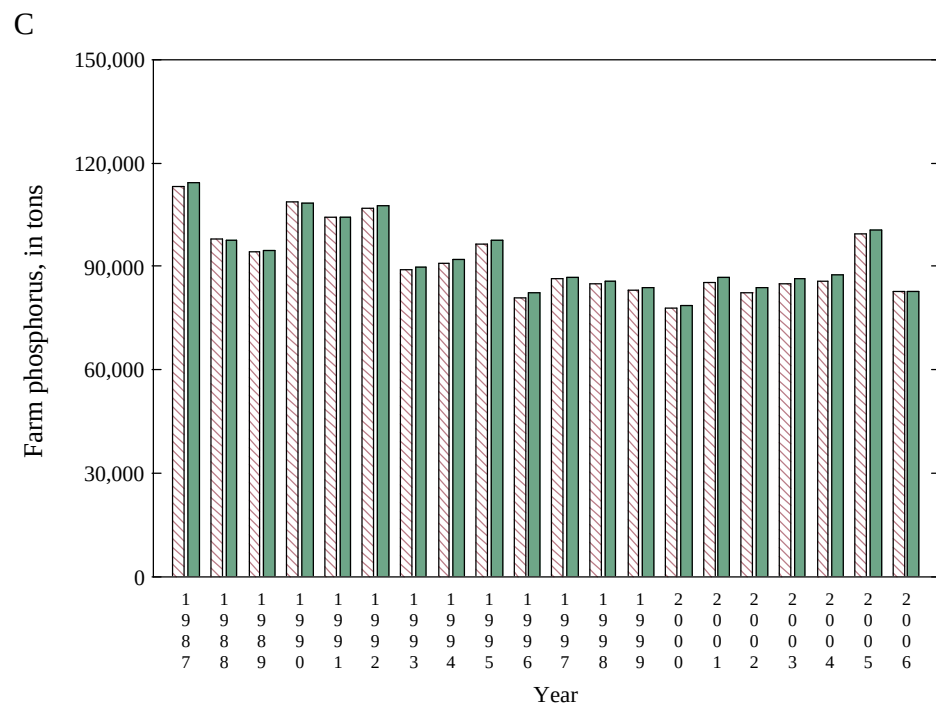
Appendix 6 Figure 8. Nitrogen and phosphorus tonnage based on national (red) and state (green) farm and nonfarm proportions for Indiana
