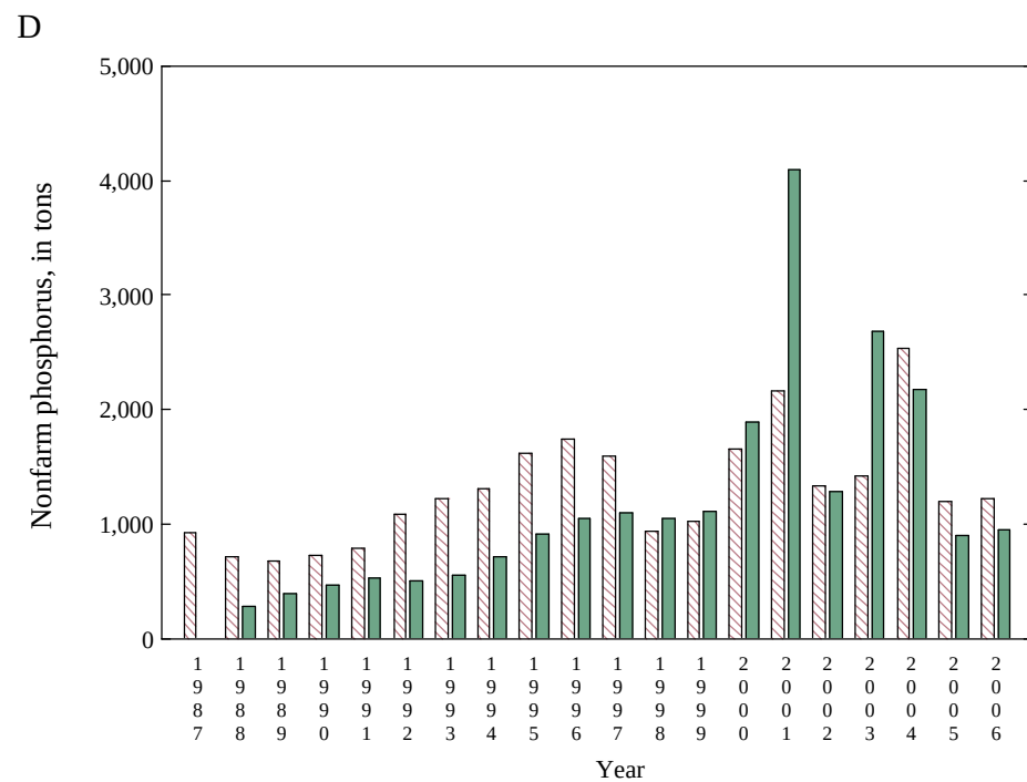
Appendix 6 Figure 29. Nitrogen and phosphorus tonnage based on national (red) and state (green) farm and nonfarm proportions for Tennessee
