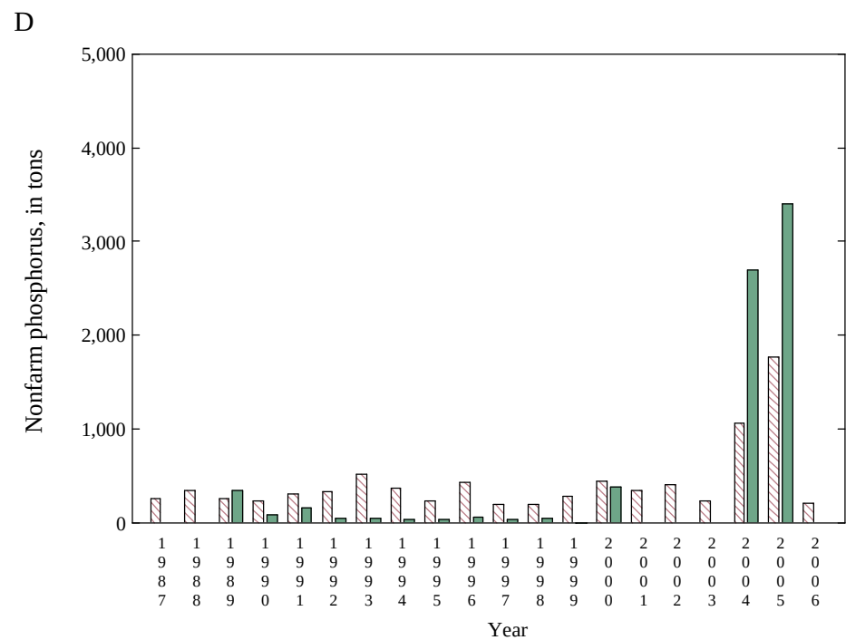
Appendix 6 Figure 25. Nitrogen and phosphorus tonnage based on national (red) and state (green) farm and nonfarm proportions for Oregon
