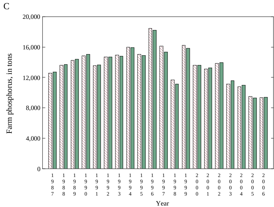
Appendix 6 Figure 28. Nitrogen and phosphorus tonnage based on national (red) and state (green) farm and nonfarm proportions for South Carolina
