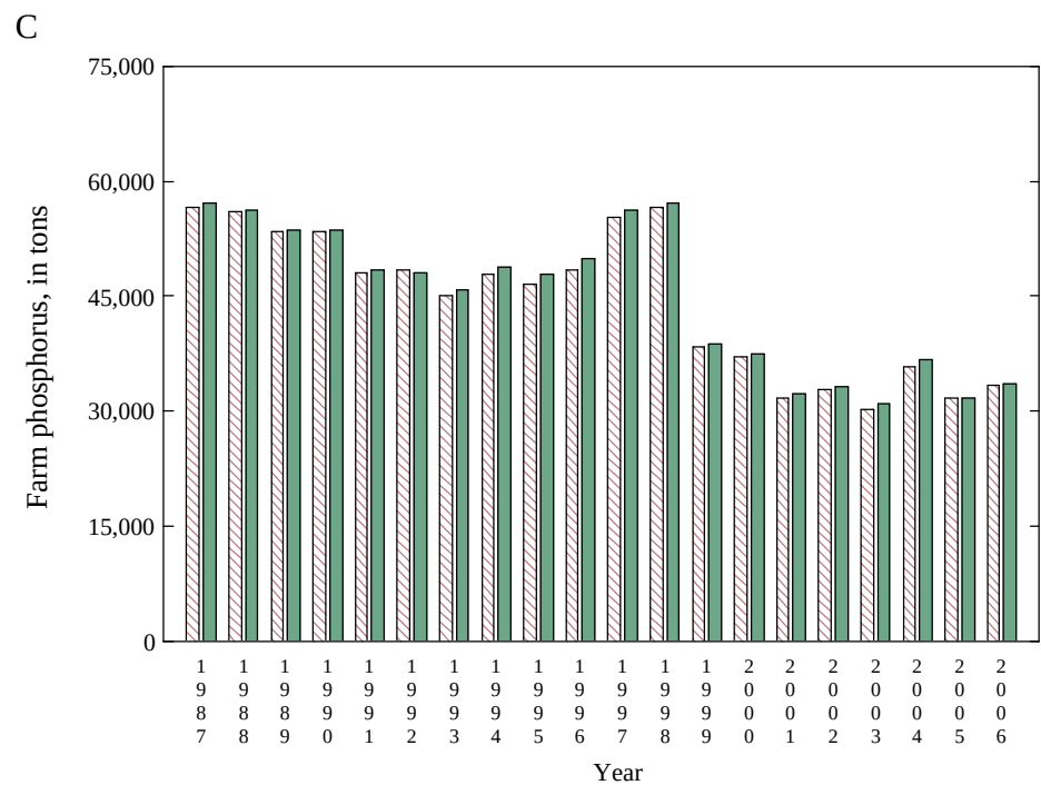
Appendix 6 Figure 35. Nitrogen and phosphorus tonnage based on national (red) and state (green) farm and nonfarm proportions for Wisconsin
