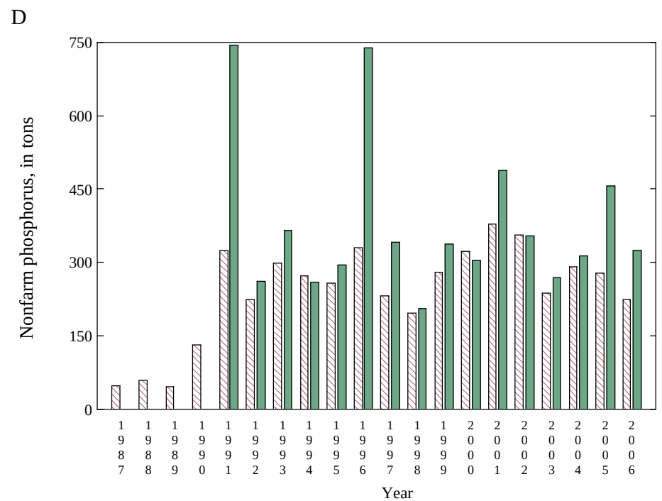
Appendix 6 Figure 30. Nitrogen and phosphorus tonnage based on national (red) and state (green) farm and nonfarm proportions for Utah
