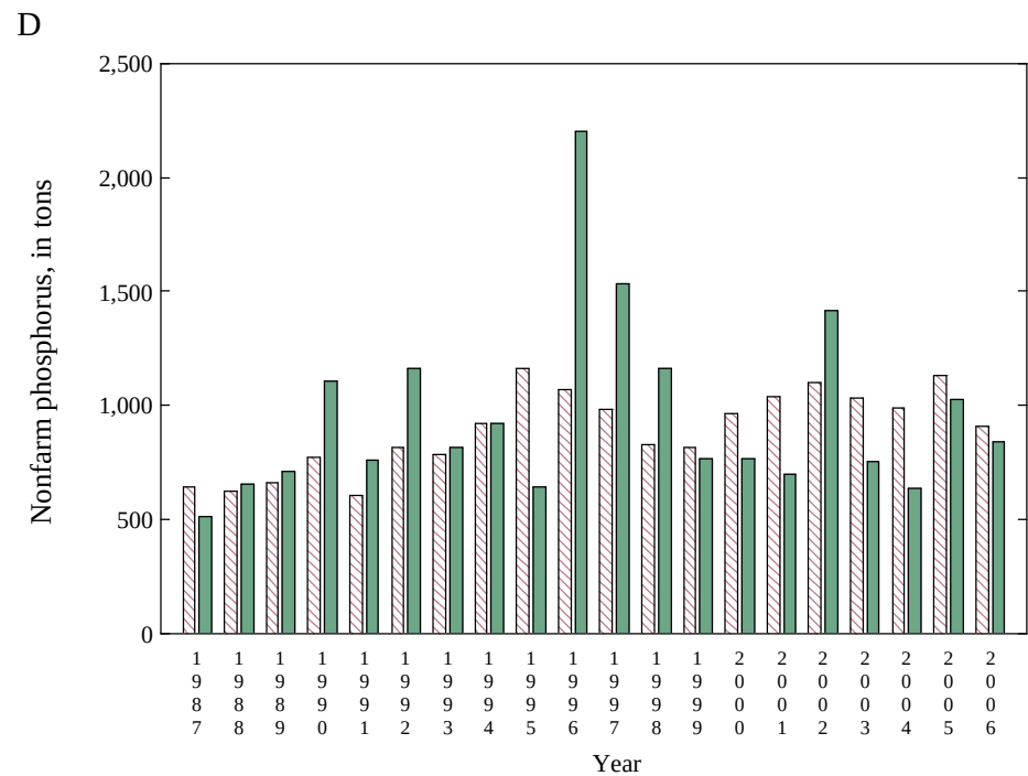
Appendix 6 Figure 10. Nitrogen and phosphorus tonnage based on national (red) and state (green) farm and nonfarm proportions for Louisiana
