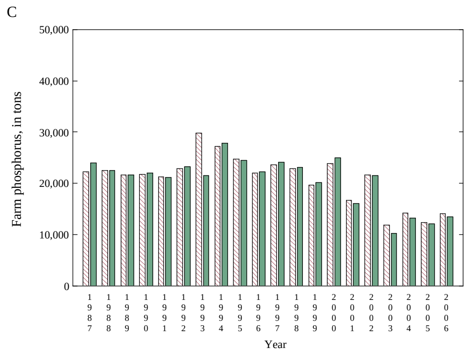
Appendix 6 Figure 26. Nitrogen and phosphorus tonnage based on national (red) and state (green) farm and nonfarm proportions for Pennsylvania
