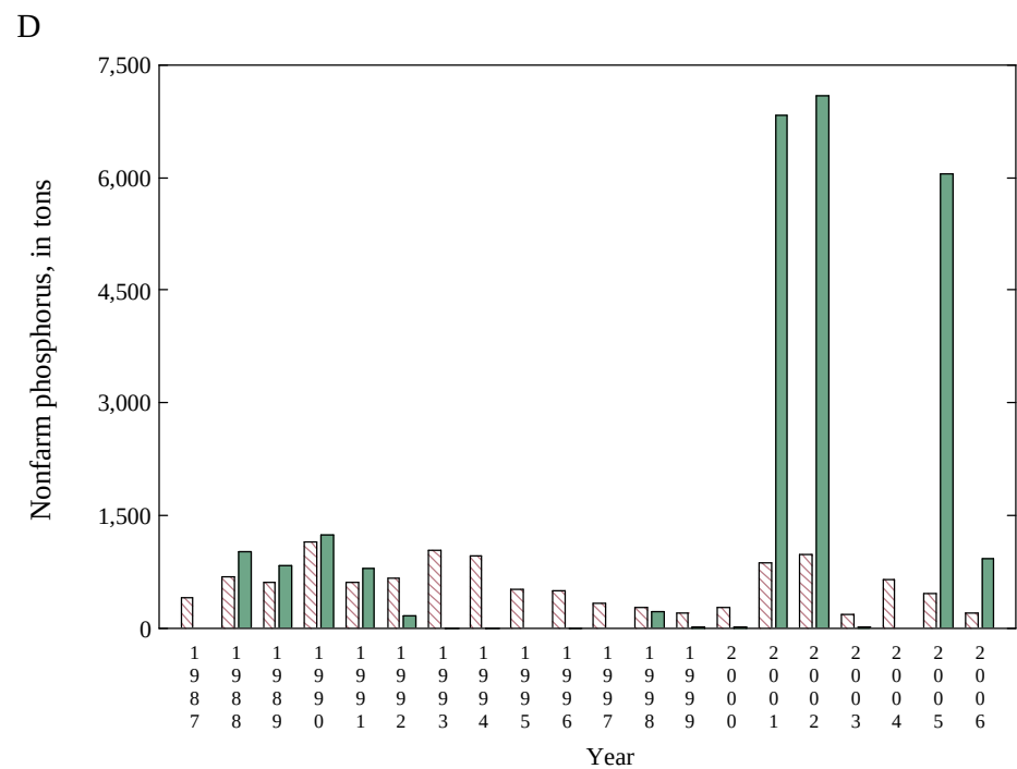
Appendix 6 Figure 3. Nitrogen and phosphorus tonnage based on national (red) and state (green) farm and nonfarm proportions for Colorado
