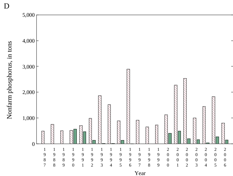
Appendix 6 Figure 17. Nitrogen and phosphorus tonnage based on national (red) and state (green) farm and nonfarm proportions for Nebraska
