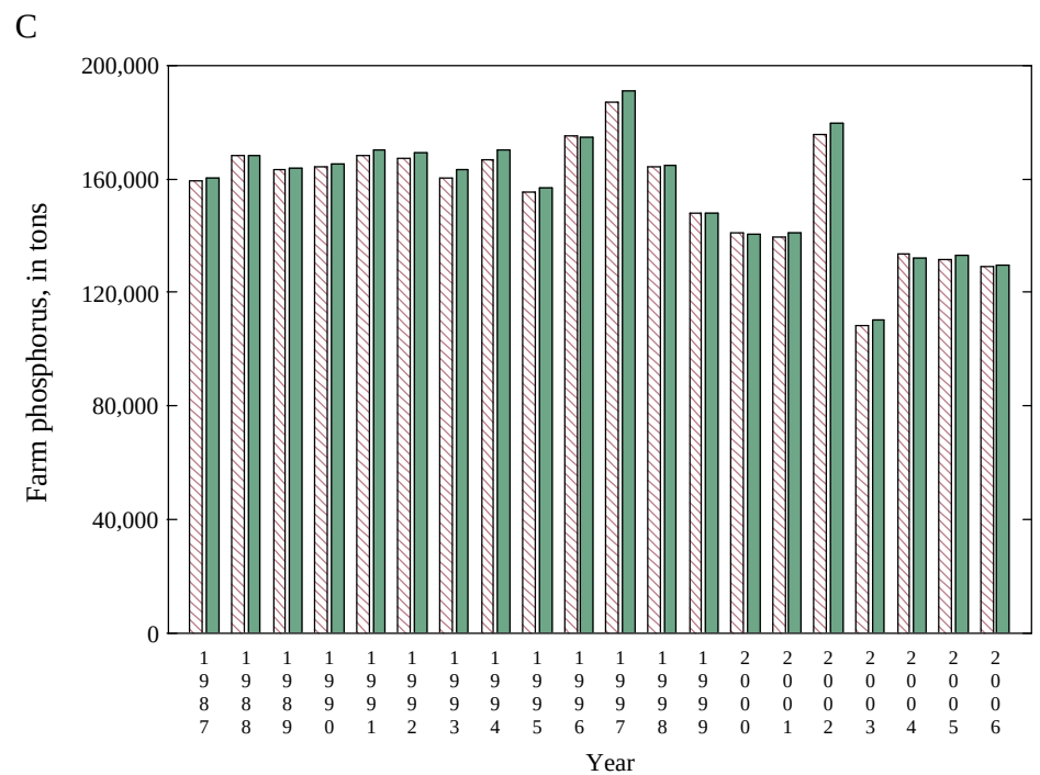
Appendix 6 Figure 7. Nitrogen and phosphorus tonnage based on national (red) and state (green) farm and nonfarm proportions for Illinois
