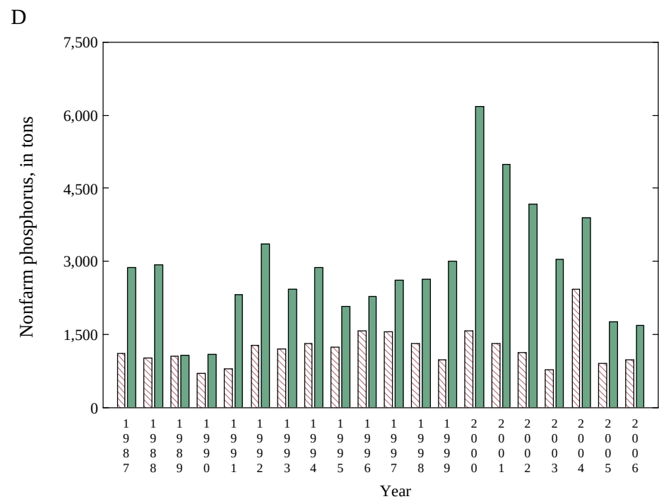
Appendix 6 Figure 12. Nitrogen and phosphorus tonnage based on national (red) and state (green) farm and nonfarm proportions for Maryland
