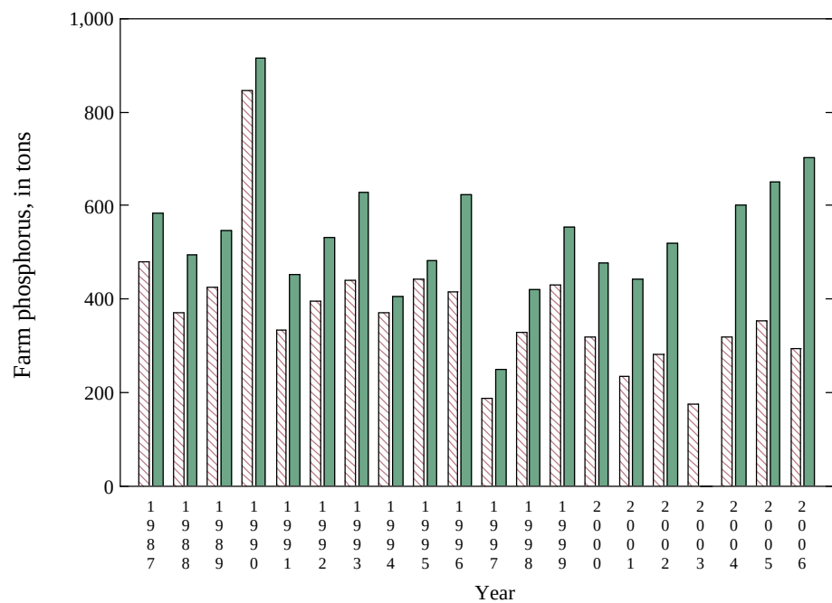
Appendix 6 Figure 19. Nitrogen and phosphorus tonnage based on national (red) and state (green) farm and nonfarm proportions for New Hampshire
