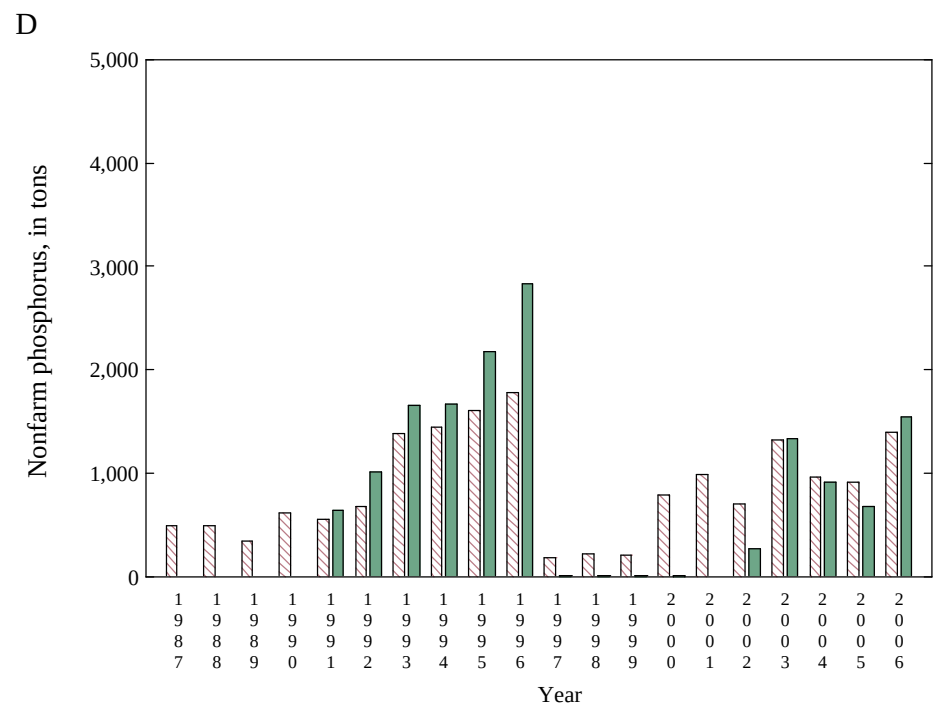
Appendix 6 Figure 33. Nitrogen and phosphorus tonnage based on national (red) and state (green) farm and nonfarm proportions for Washington
