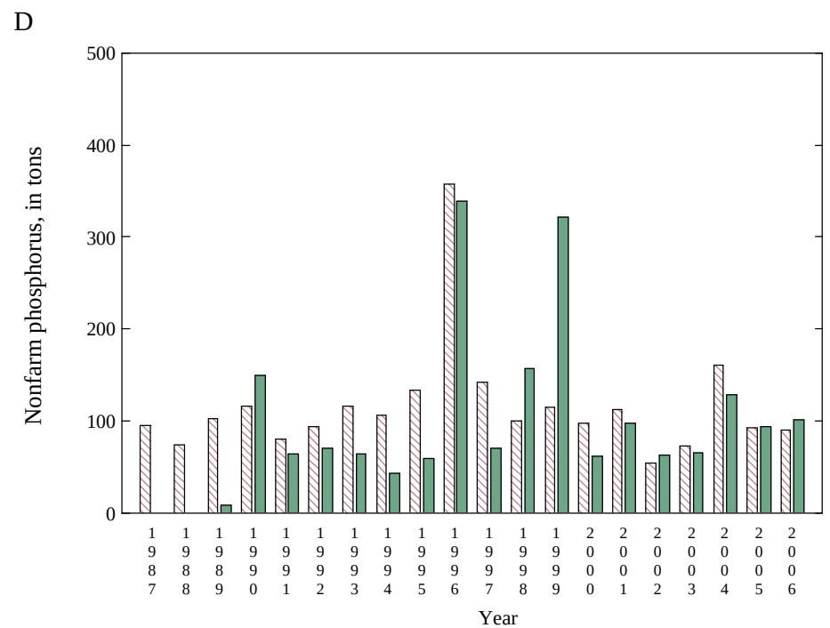
Appendix 6 Figure 31. Nitrogen and phosphorus tonnage based on national (red) and state (green) farm and nonfarm proportions for Vermont
