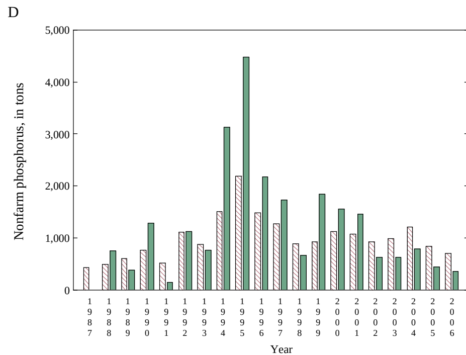
Appendix 6 Figure 15. Nitrogen and phosphorus tonnage based on national (red) and state (green) farm and nonfarm proportions for Mississippi
