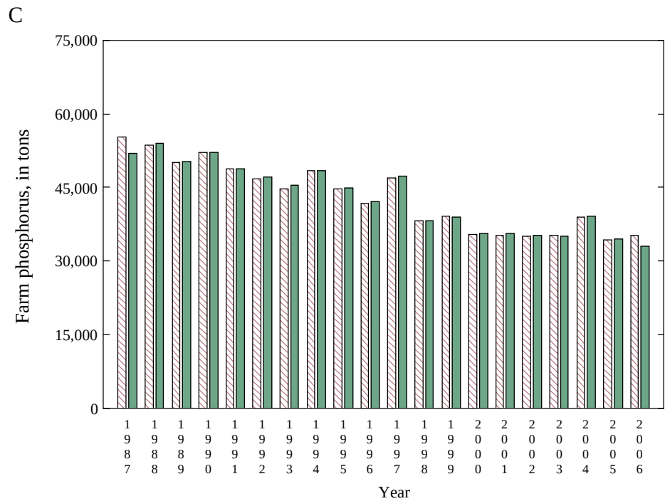
Appendix 6 Figure 14. Nitrogen and phosphorus tonnage based on national (red) and state (green) farm and nonfarm proportions for Michigan
