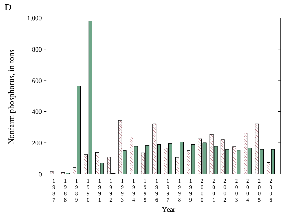
Appendix 6 Figure 36. Nitrogen and phosphorus tonnage based on national (red) and state (green) farm and nonfarm proportions for Wyoming
