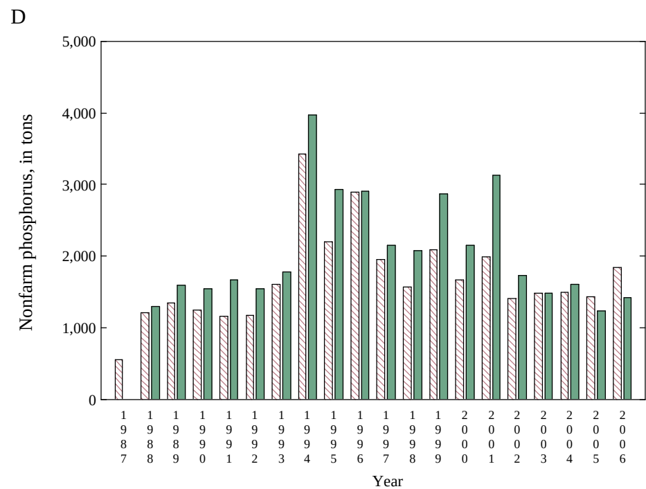
Appendix 6 Figure 20. Nitrogen and phosphorus tonnage based on national (red) and state (green) farm and nonfarm proportions for New Jersey
