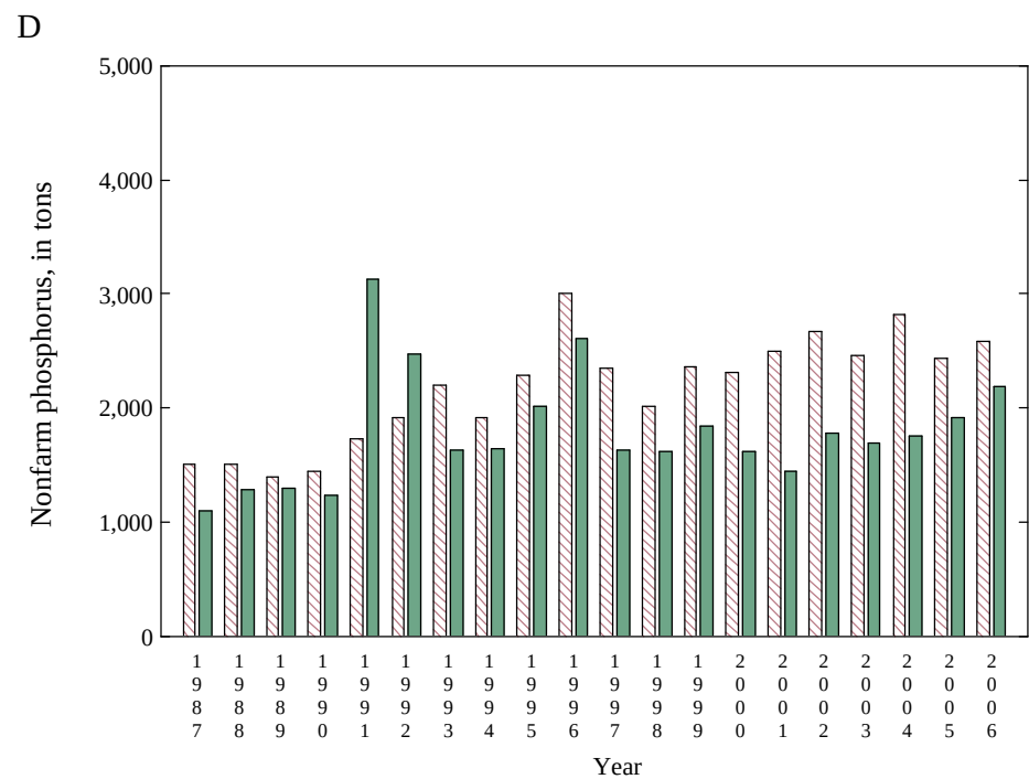
Appendix 6 Figure 32. Nitrogen and phosphorus tonnage based on national (red) and state (green) farm and nonfarm proportions for Virginia
