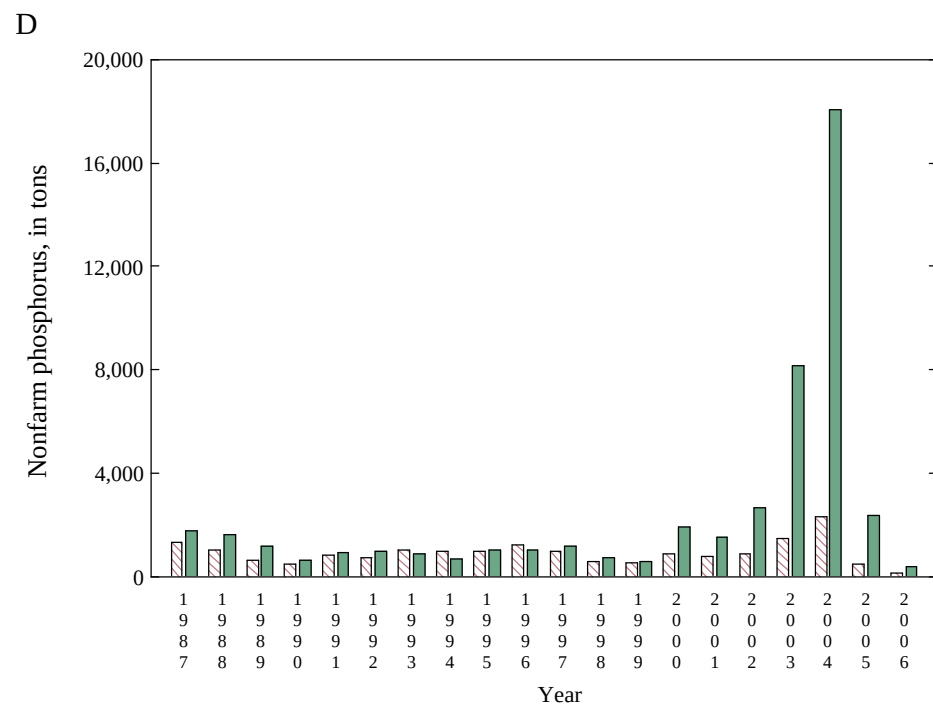
Appendix 6 Figure 24. Nitrogen and phosphorus tonnage based on national (red) and state (green) farm and nonfarm proportions for Oklahoma
