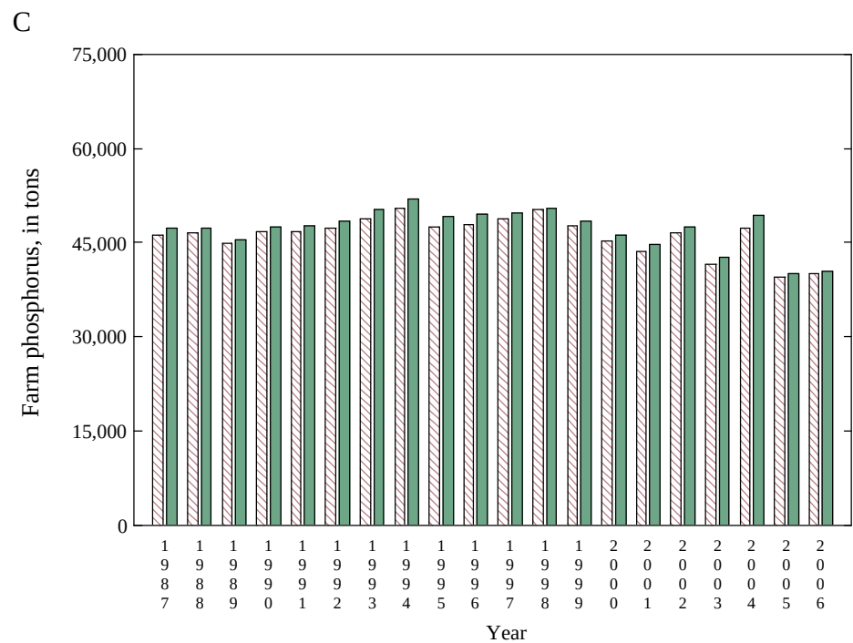
Appendix 6 Figure 9. Nitrogen and phosphorus tonnage based on national (red) and state (green) farm and nonfarm proportions for Kentucky
