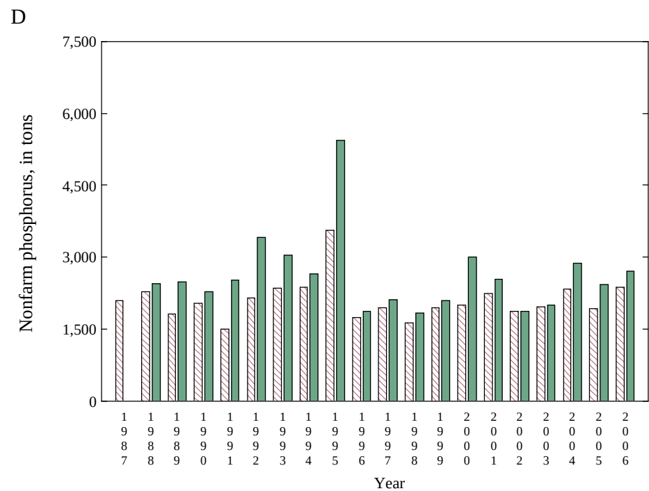
Appendix 6 Figure 22. Nitrogen and phosphorus tonnage based on national (red) and state (green) farm and nonfarm proportions for New York
