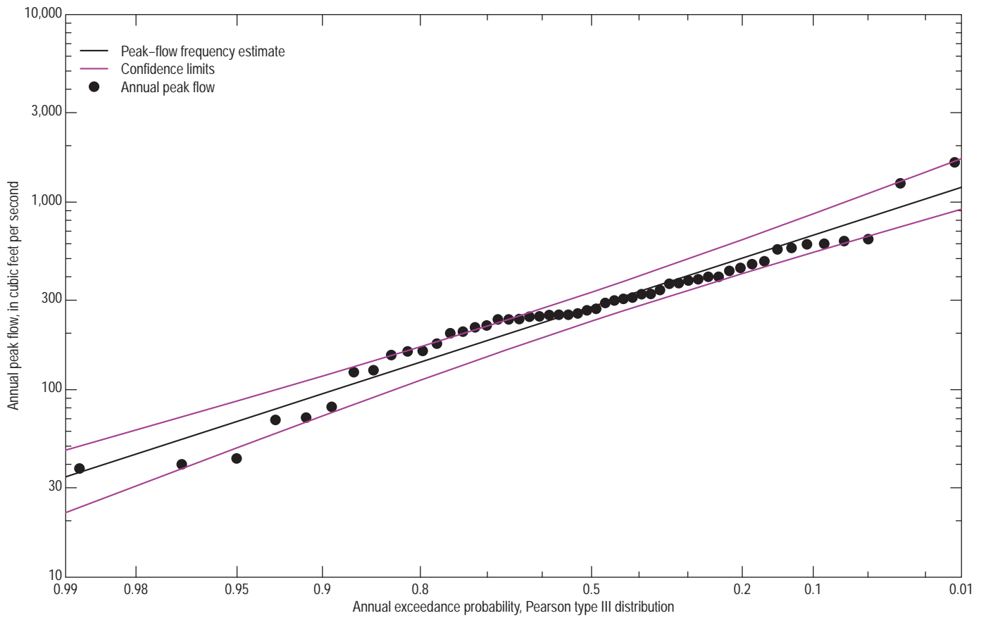
05060800 Buffalo River near Callaway, Minn.
