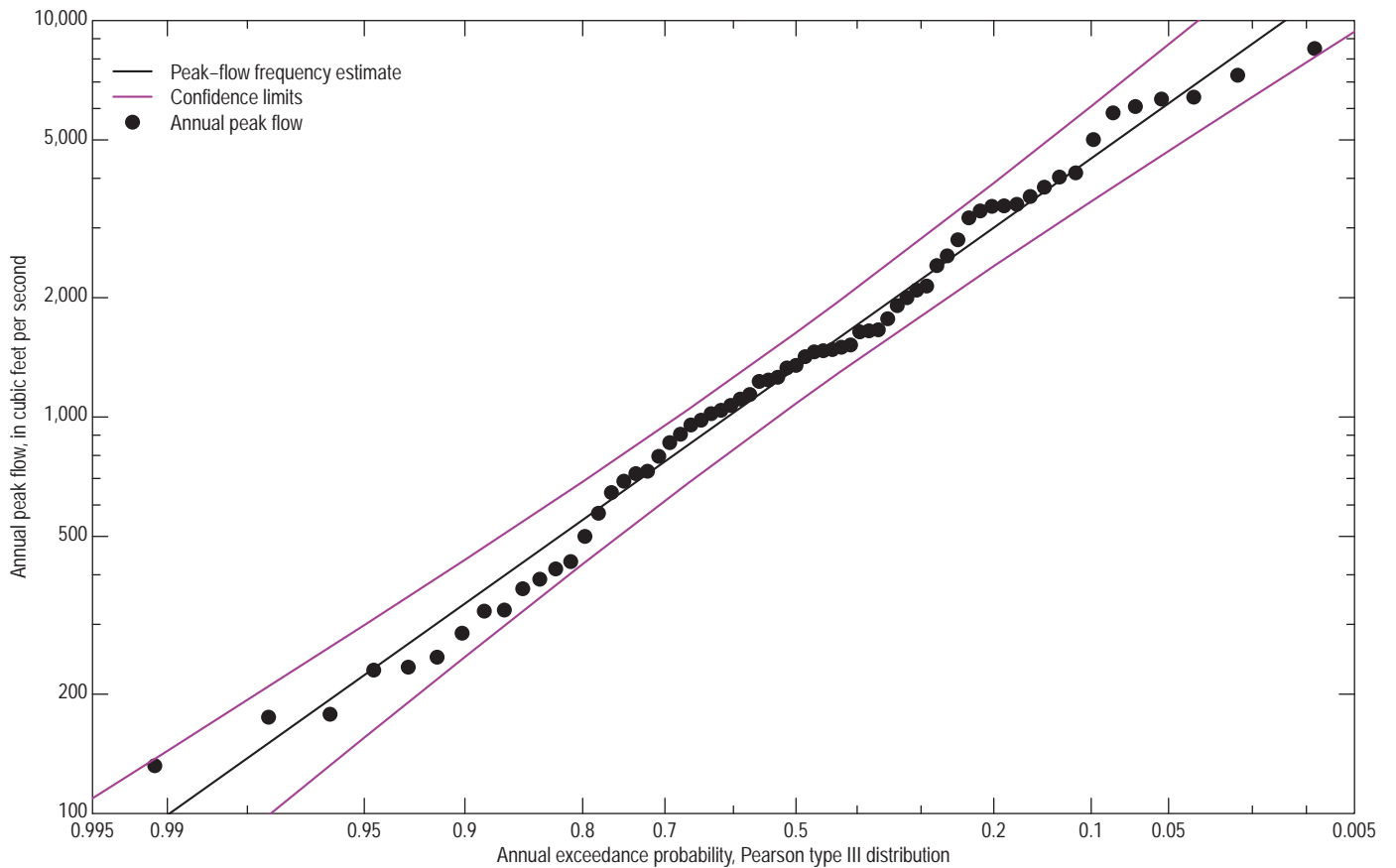
05061500 South Branch Buffalo River at Sabin, Minn.
