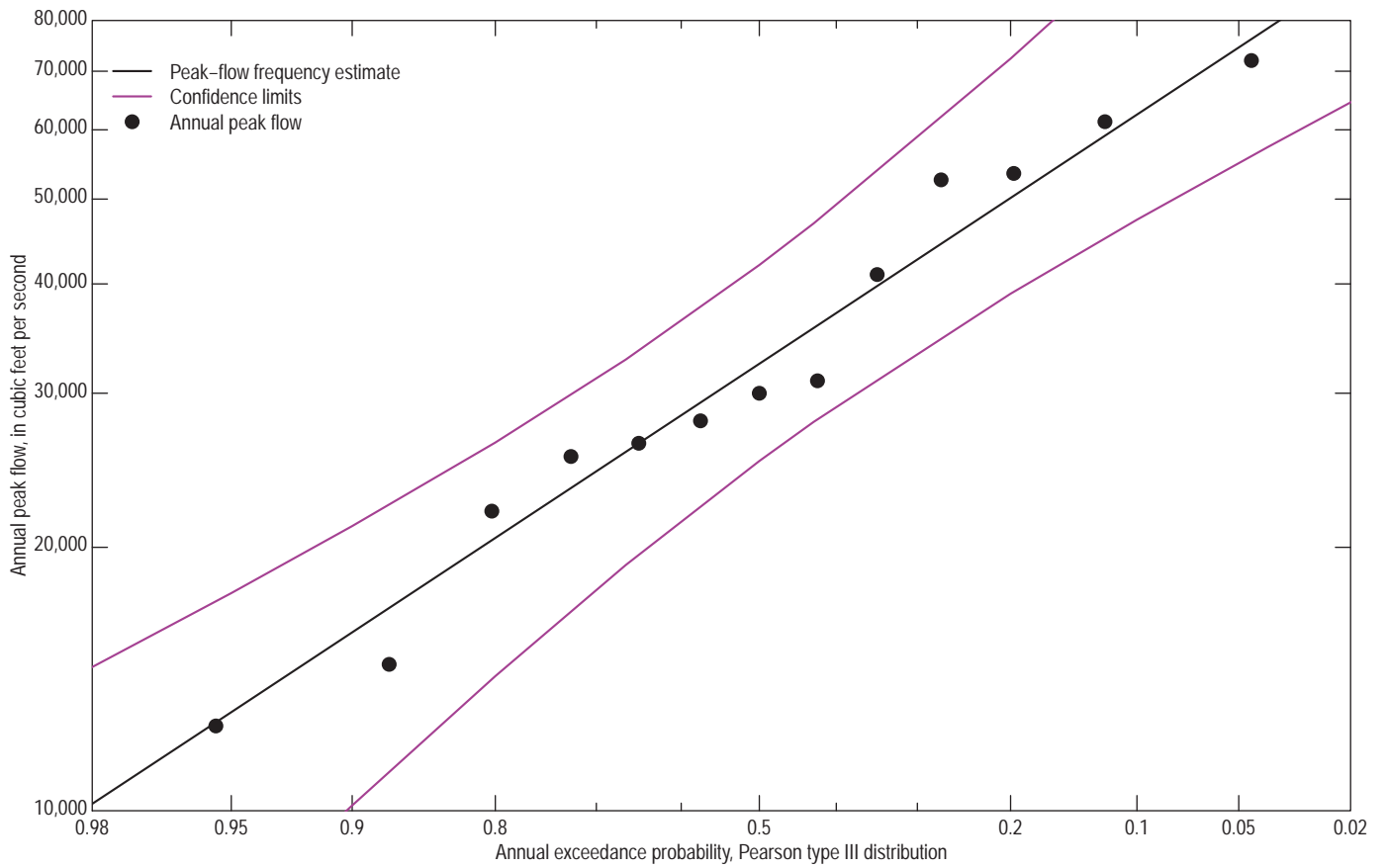
05070000 Red River of the North near Thompson, N. Dak.
