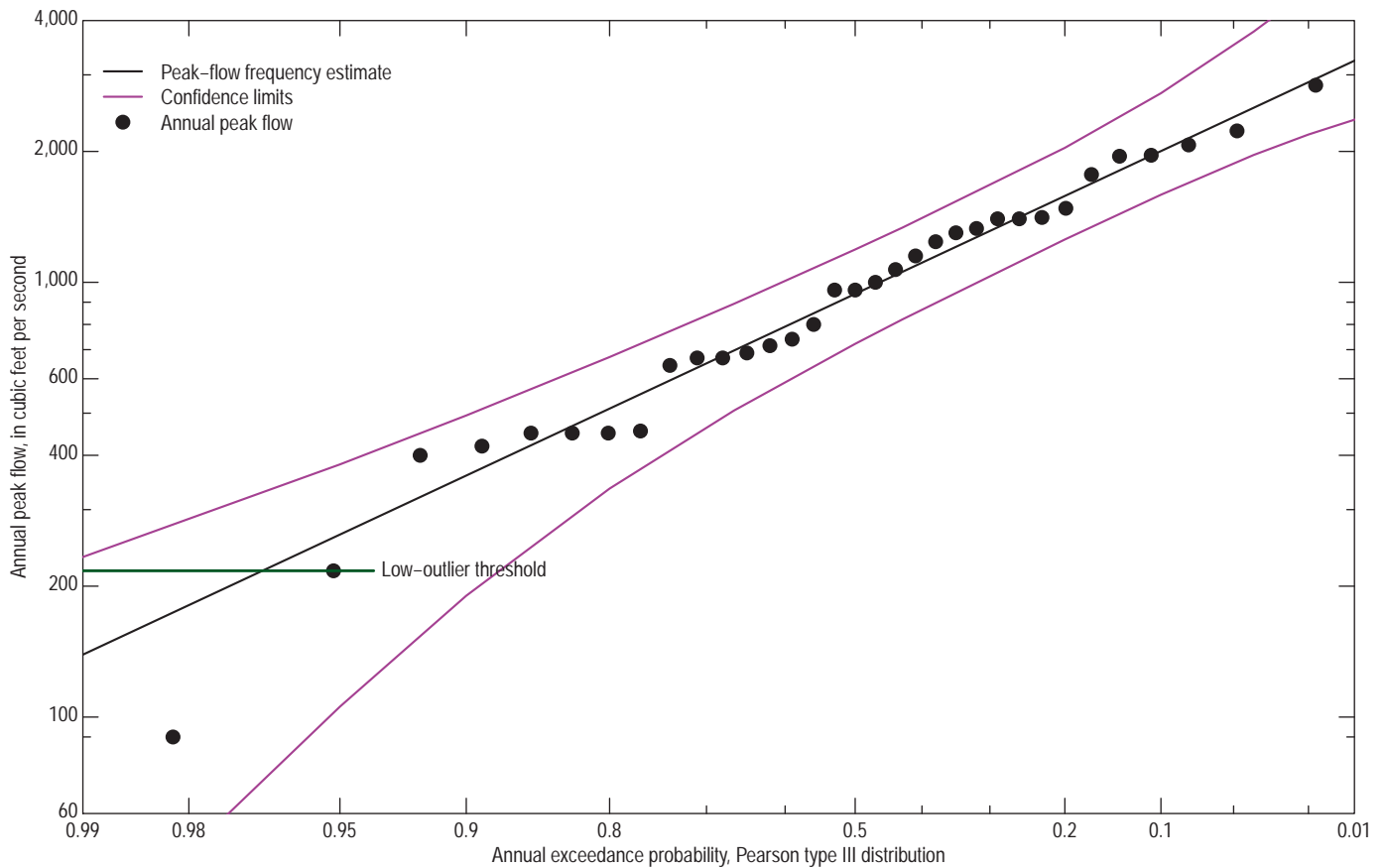
05075700 Mud River near Grygla, Minn.
