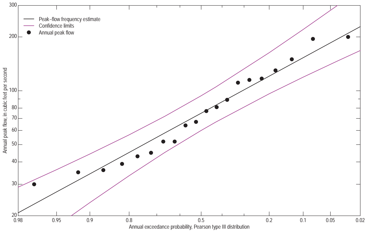
05076600 Red Lake River tributary near Thief River Falls, Minn.
