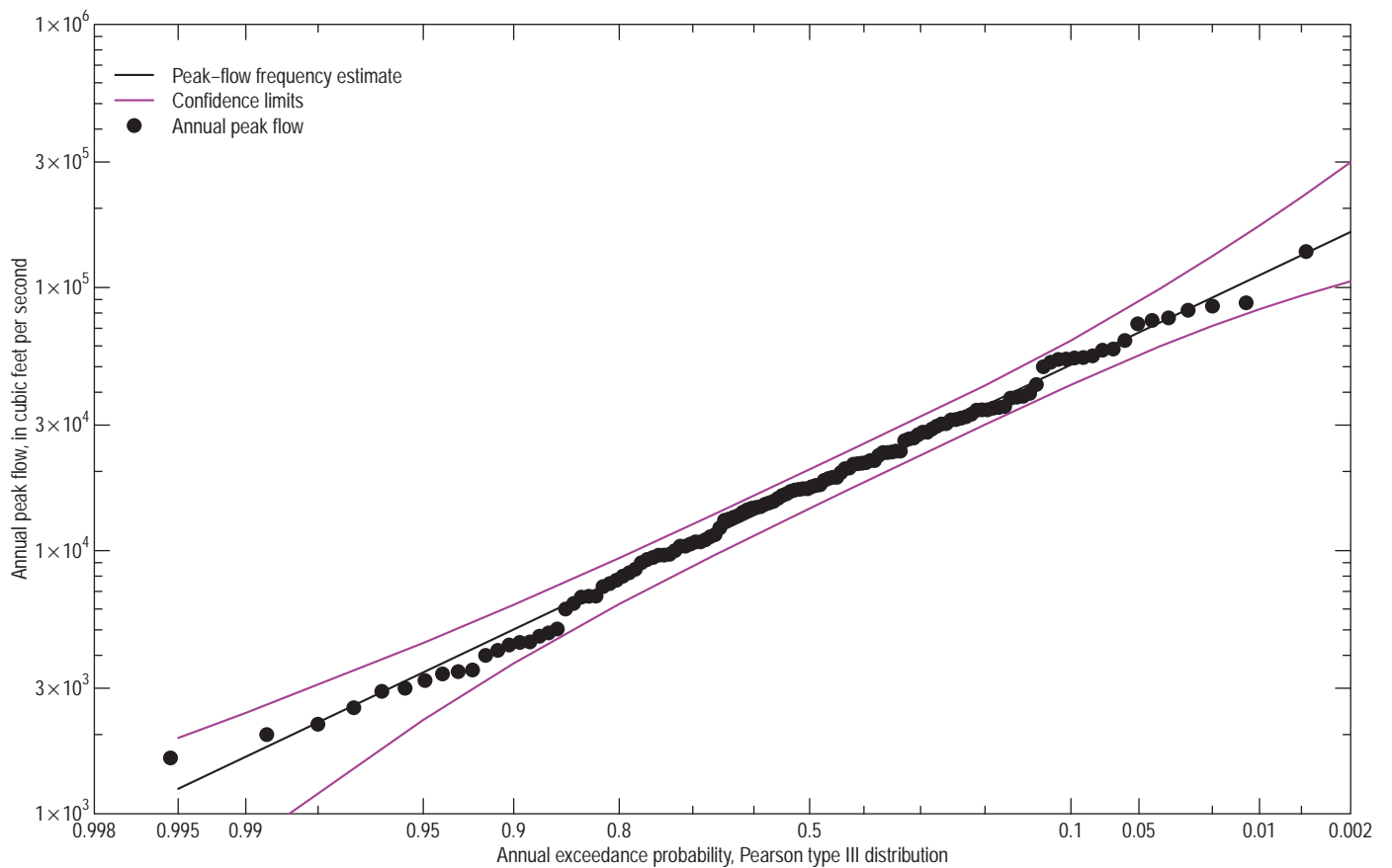
05082500 Red River of the North at Grand Forks, N. Dak.
