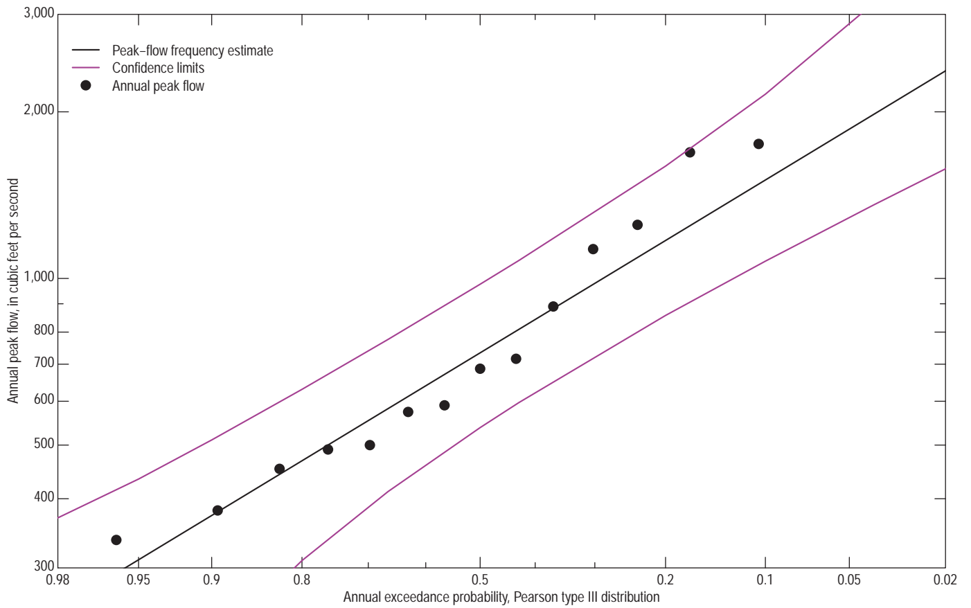
05128500 Pike River near Embarrass, Minn.
