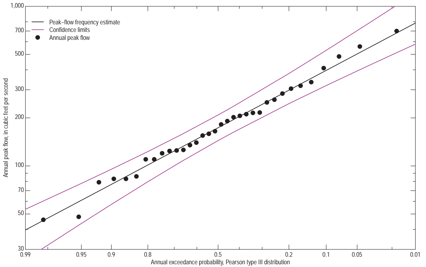
05130300 Boriin Creek near Chisholm, Minn.
