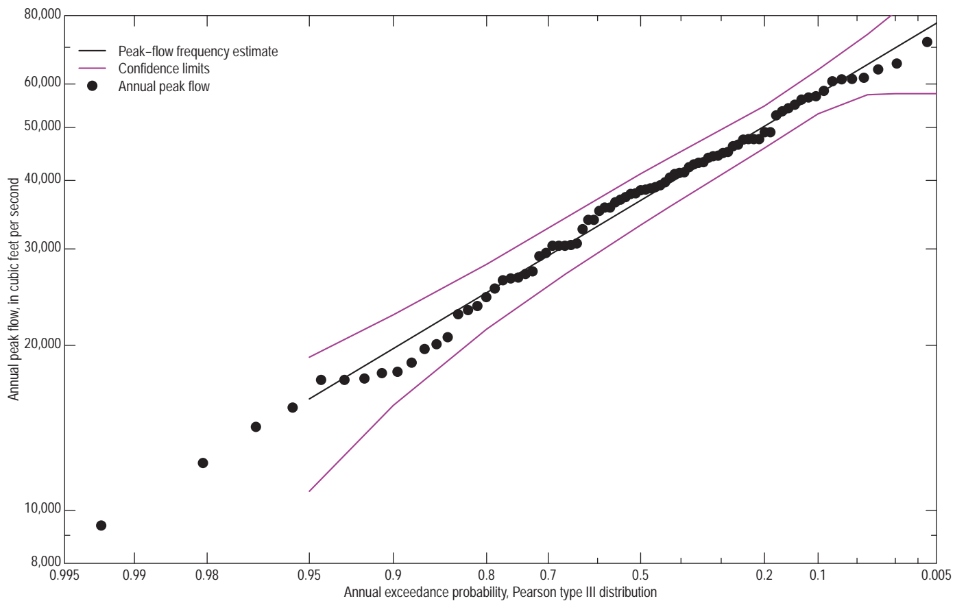
05133500 Rainy River at Manitou Rapids, Minn.
