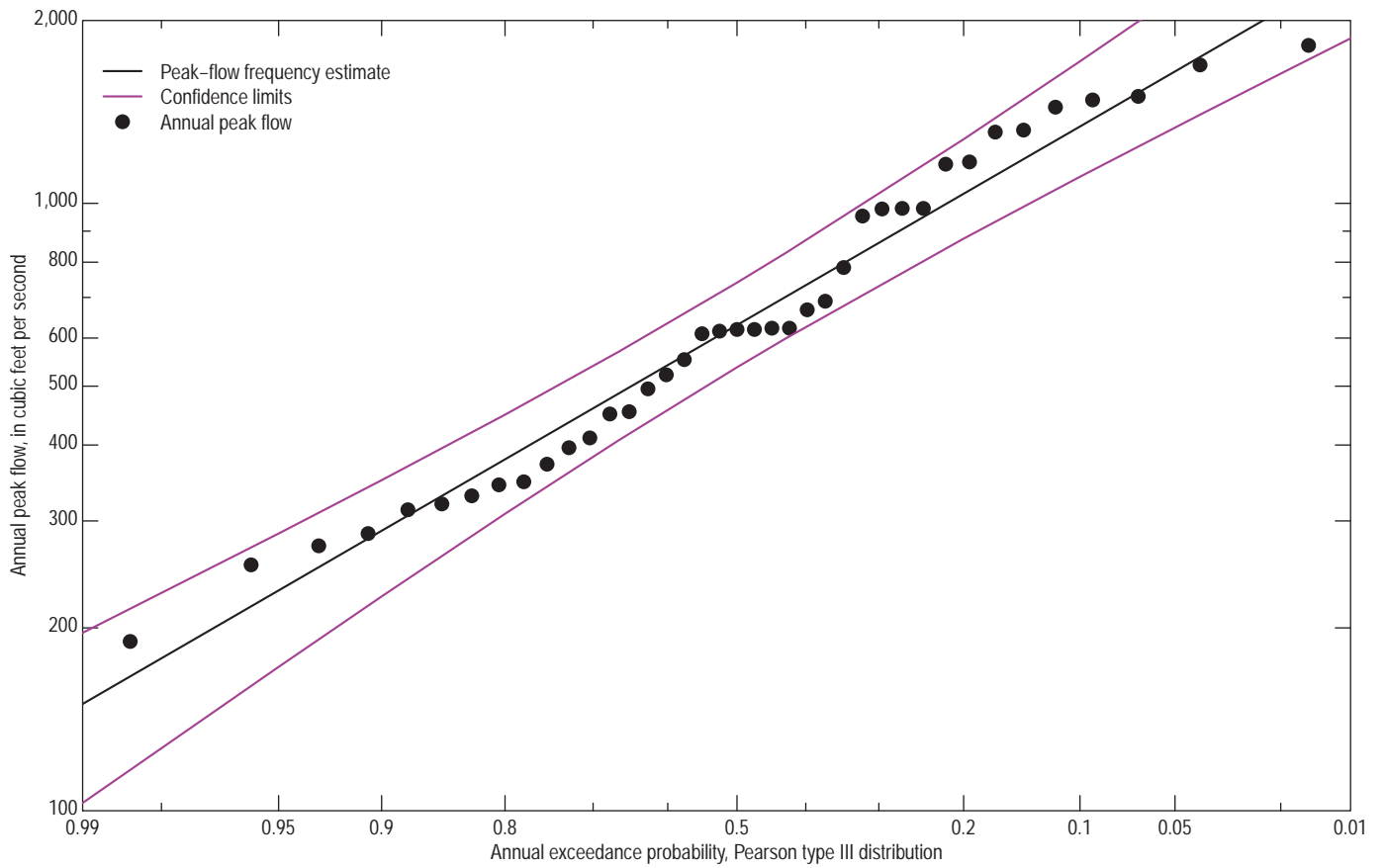
05200445 Mississippi River at Bemidji, Minn.
