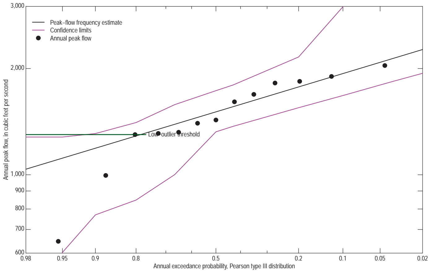
05219000 Sandy River at Sandy Lake Dam, at Libby, Minn.
