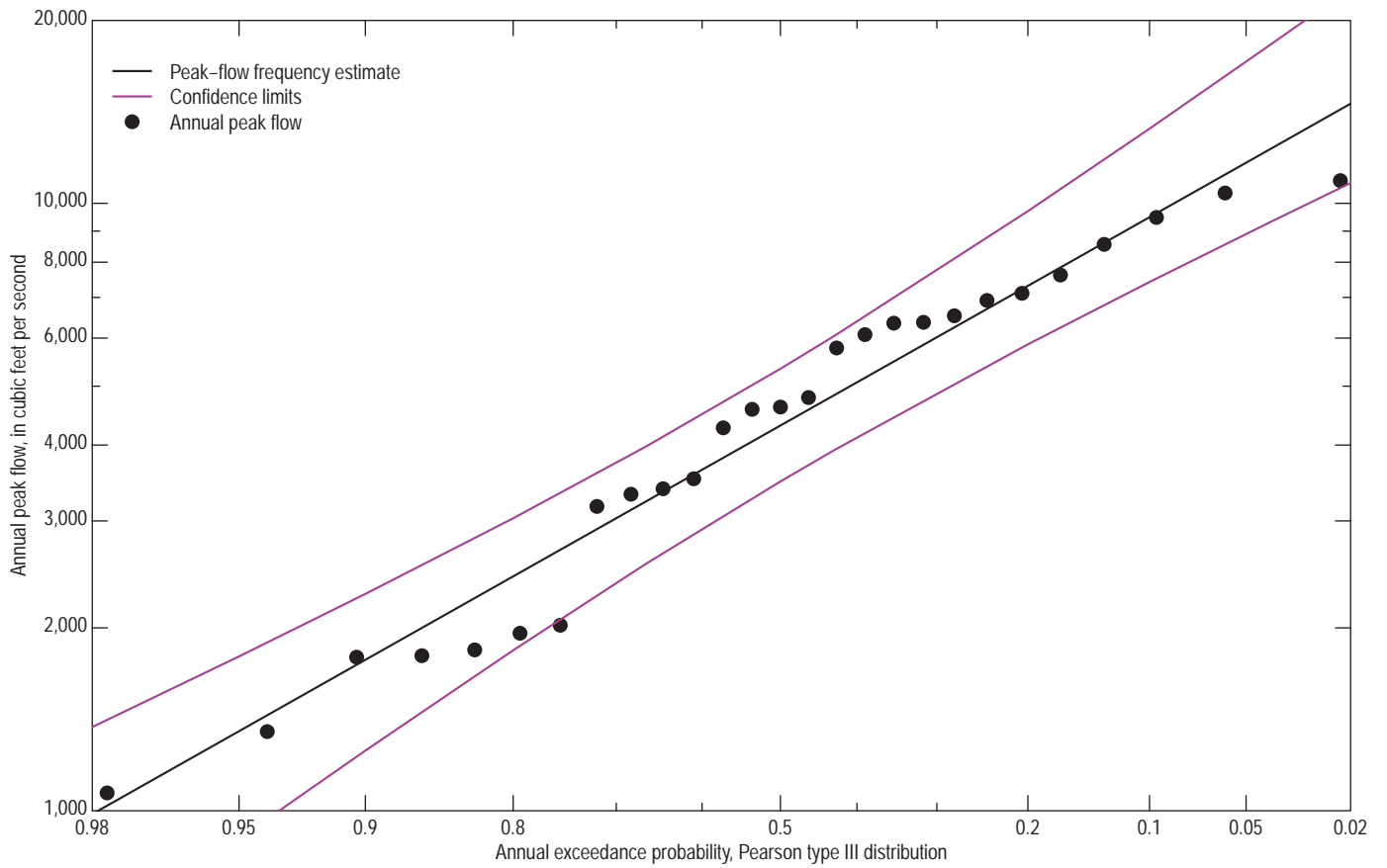
05246000 Crow Wing River at Pillager, Minn.
