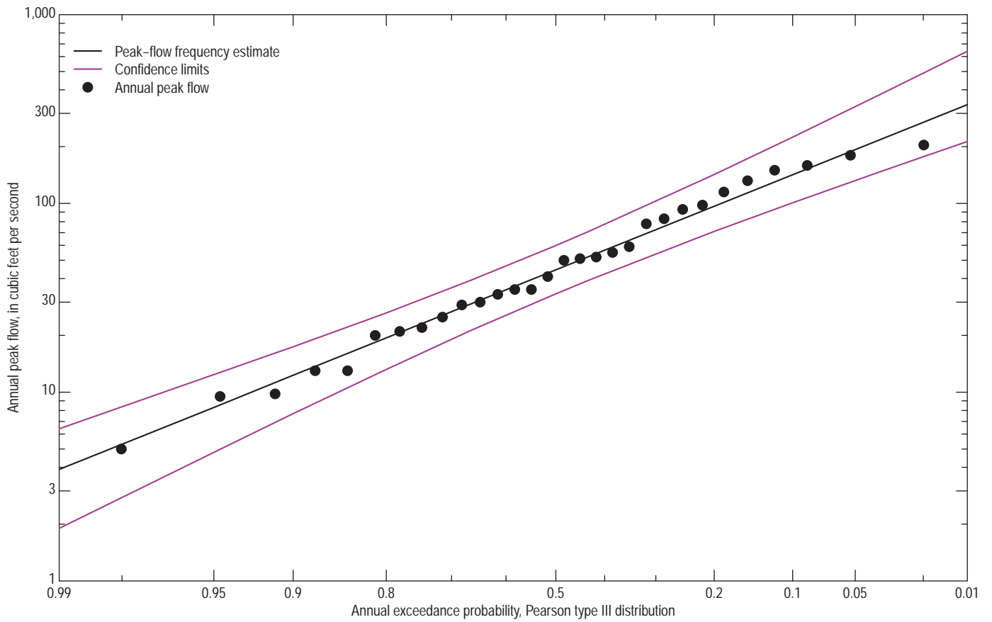
05274200 Stony Brook tributary near Foley, Minn.
