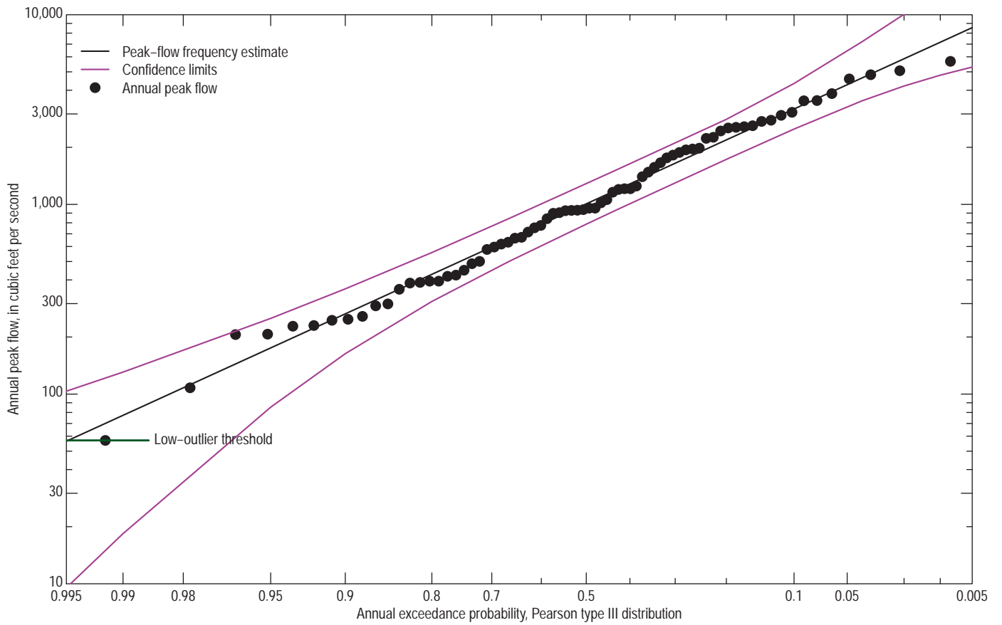
05292000 Minnesota River at Ortonville, Minn.
