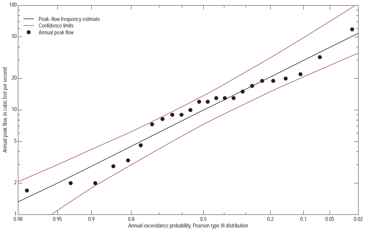
05302970 Outlet Creek tributary near Starbuck, Minn.
