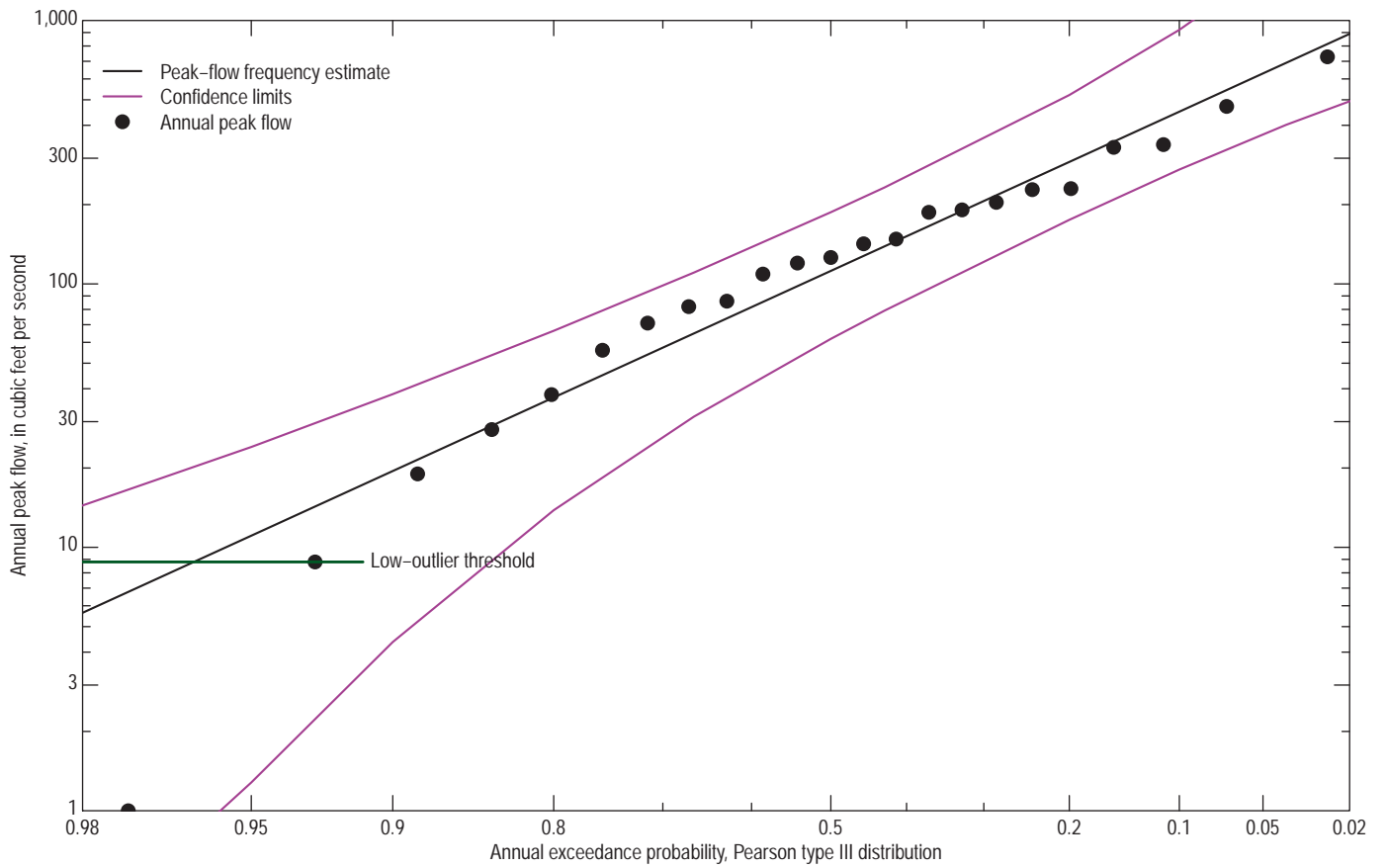
05314900 Redwood River at Ruthton, Minn.
