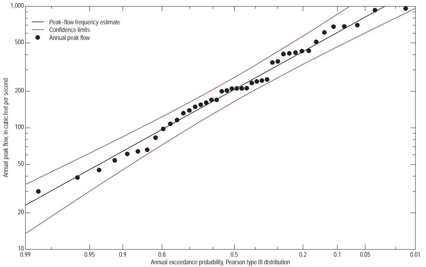
05316700 Spring Creek near Sleepy Eye, Minn.
