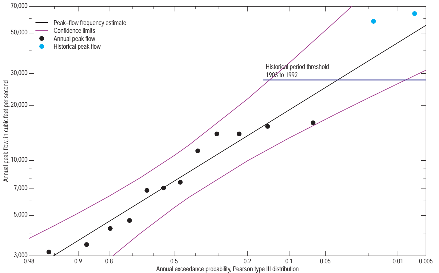
05317500 Minnesota River at Judson, Minn.
