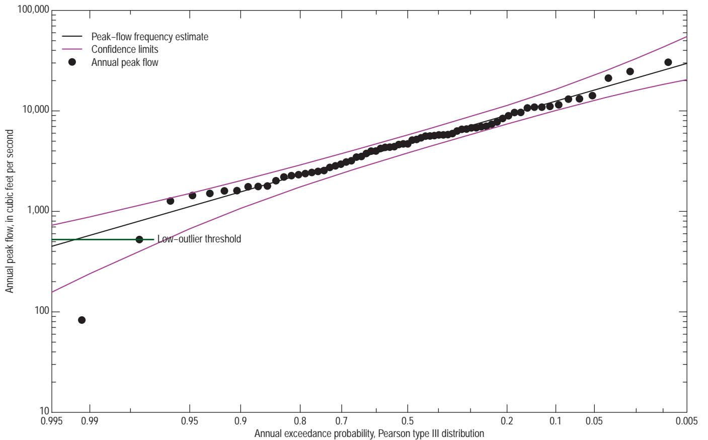
05320500 Le Sueur River near Rapidan, Minn.
