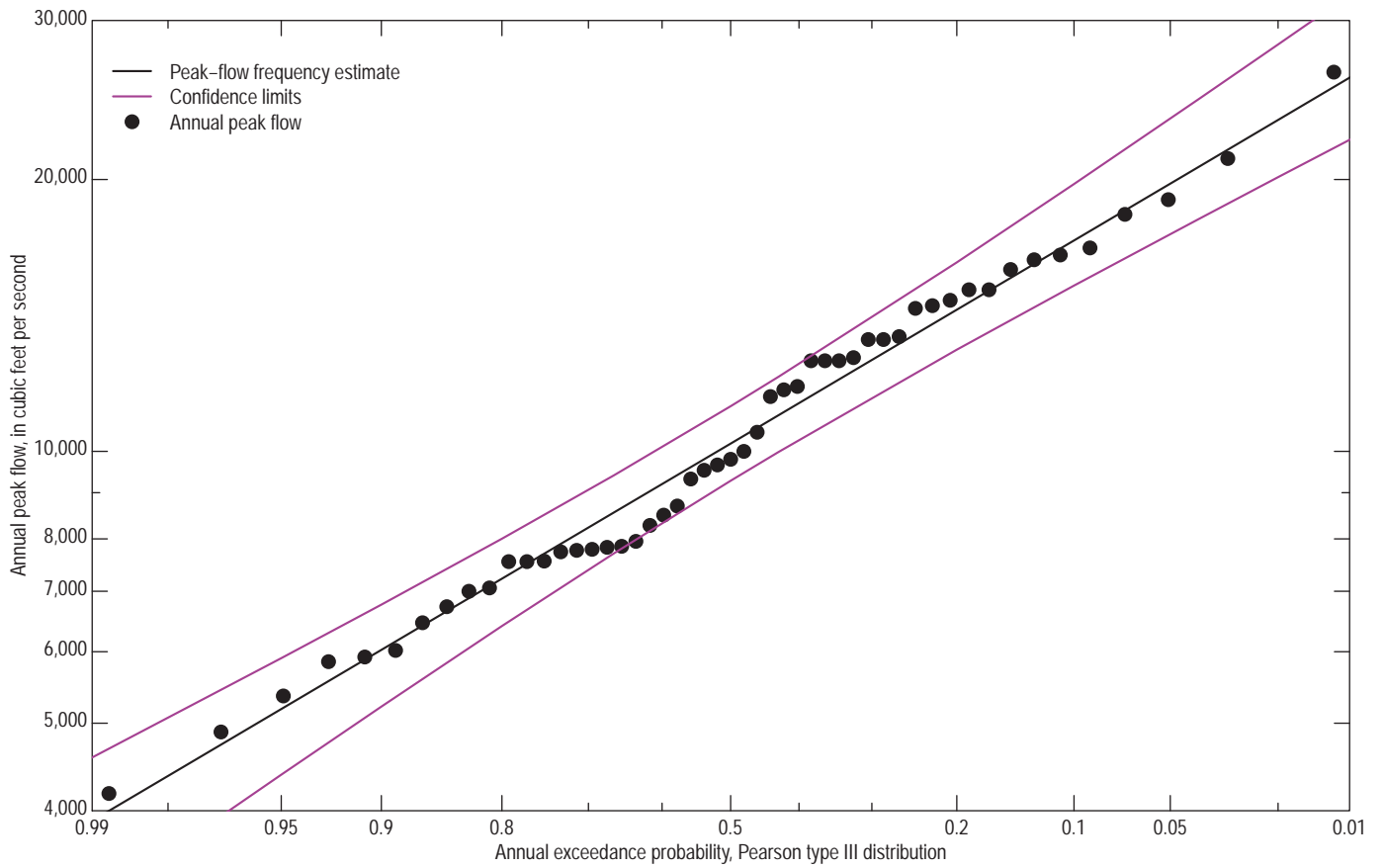
05336000 St. Croix River near Grantsburg, Wis.
