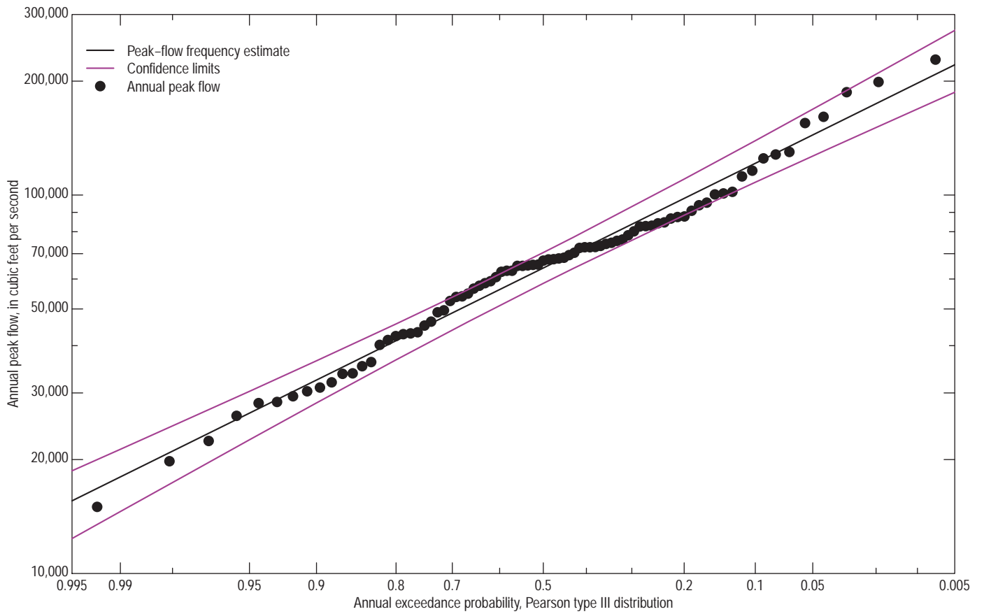
05344500 Mississippi River at Prescott, Wis.
