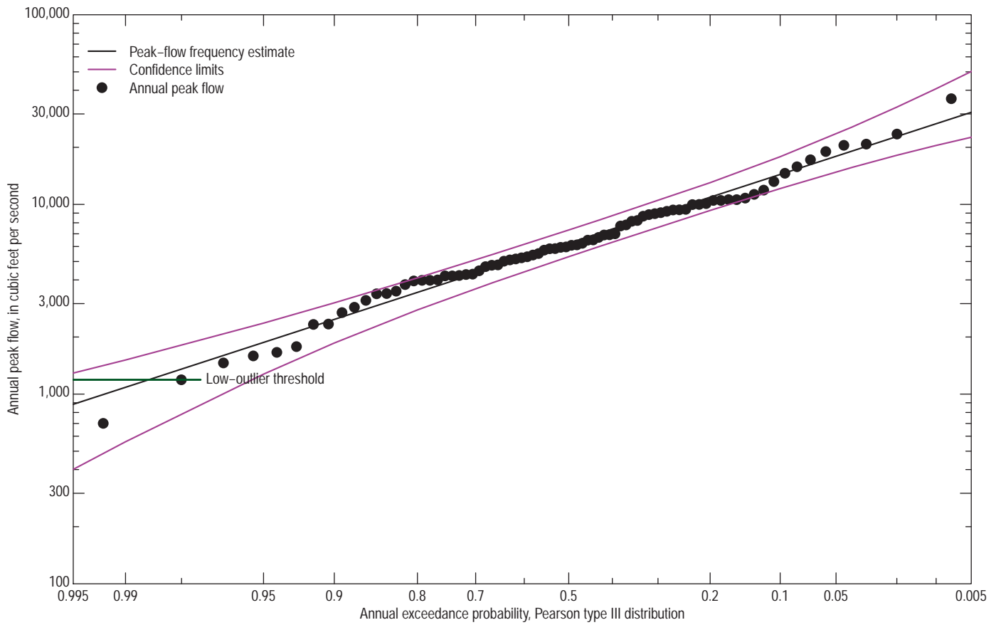
05355200 Cannon River at Welch, Minn.
