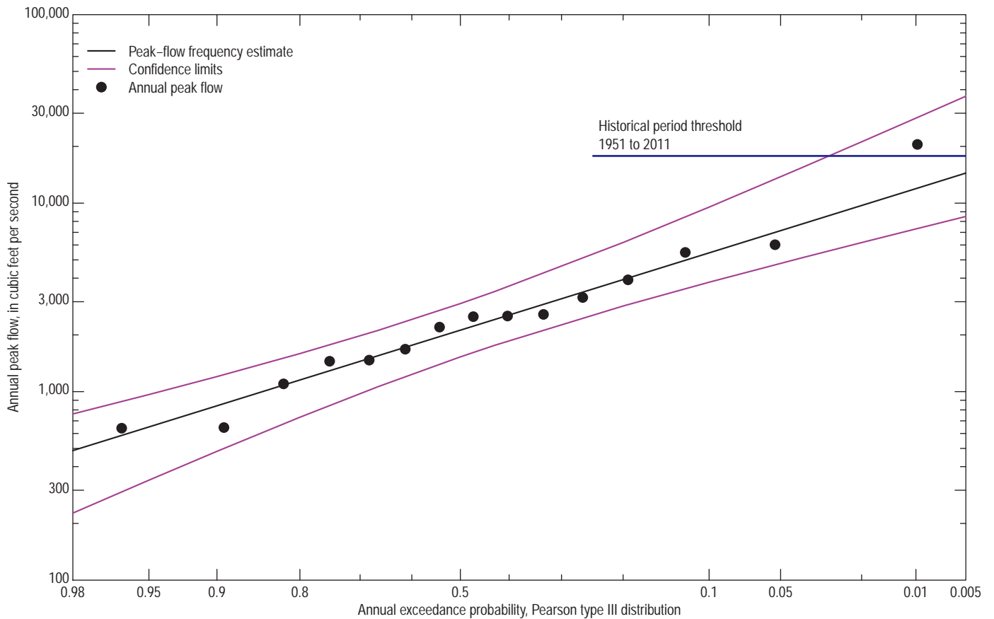
05372800 South Fork Zumbro River on belt line at Rochester, Minn.
