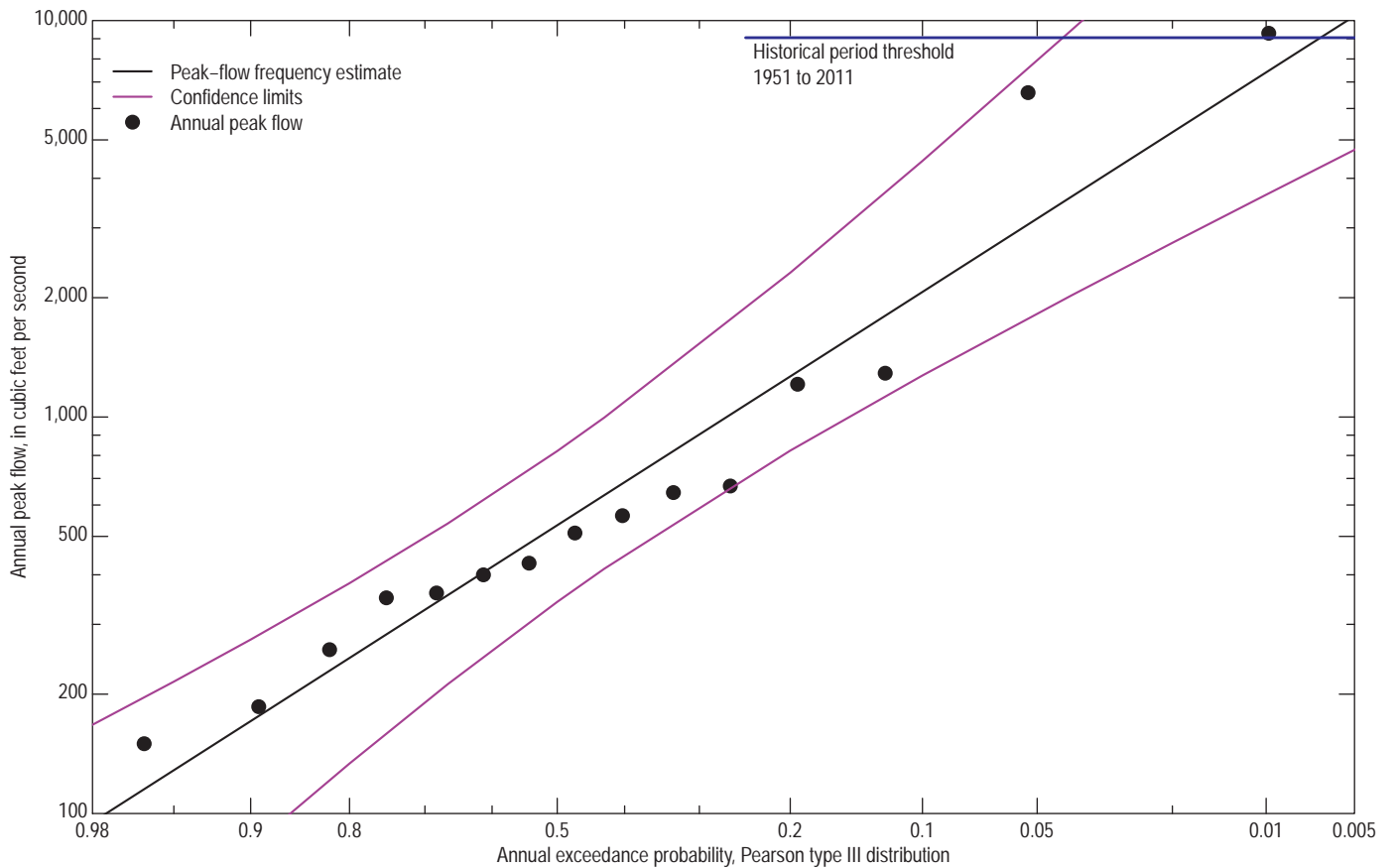
05372950 Silver Creek at Minnesota Department of Natural Resources gage in Rochester, Minn.
