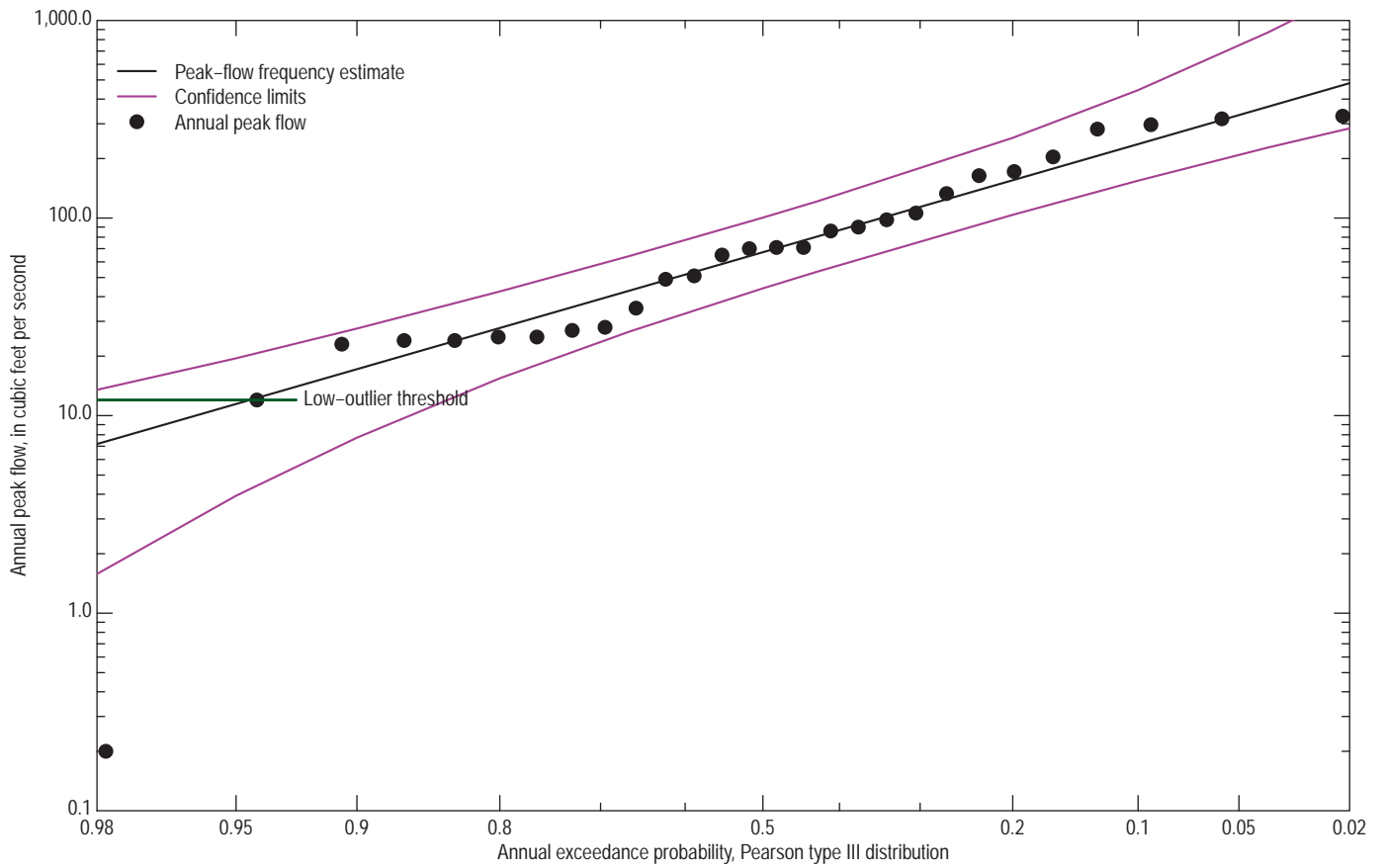
05383600 North Branch Root River tributary near Stewartville, Minn.
