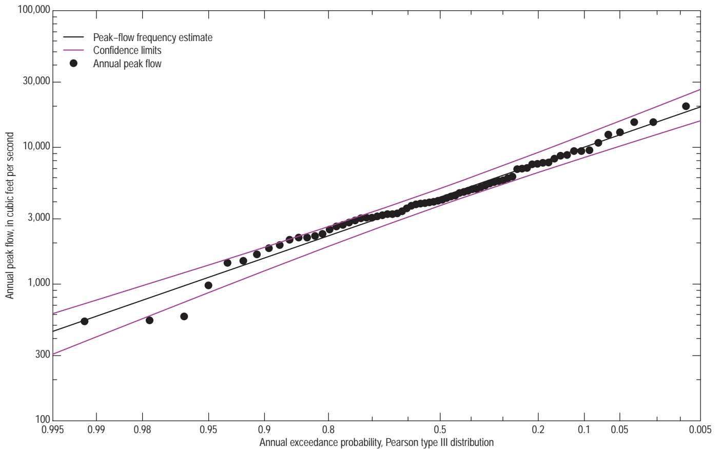
05457000 Cedar River near Austin, Minn.
