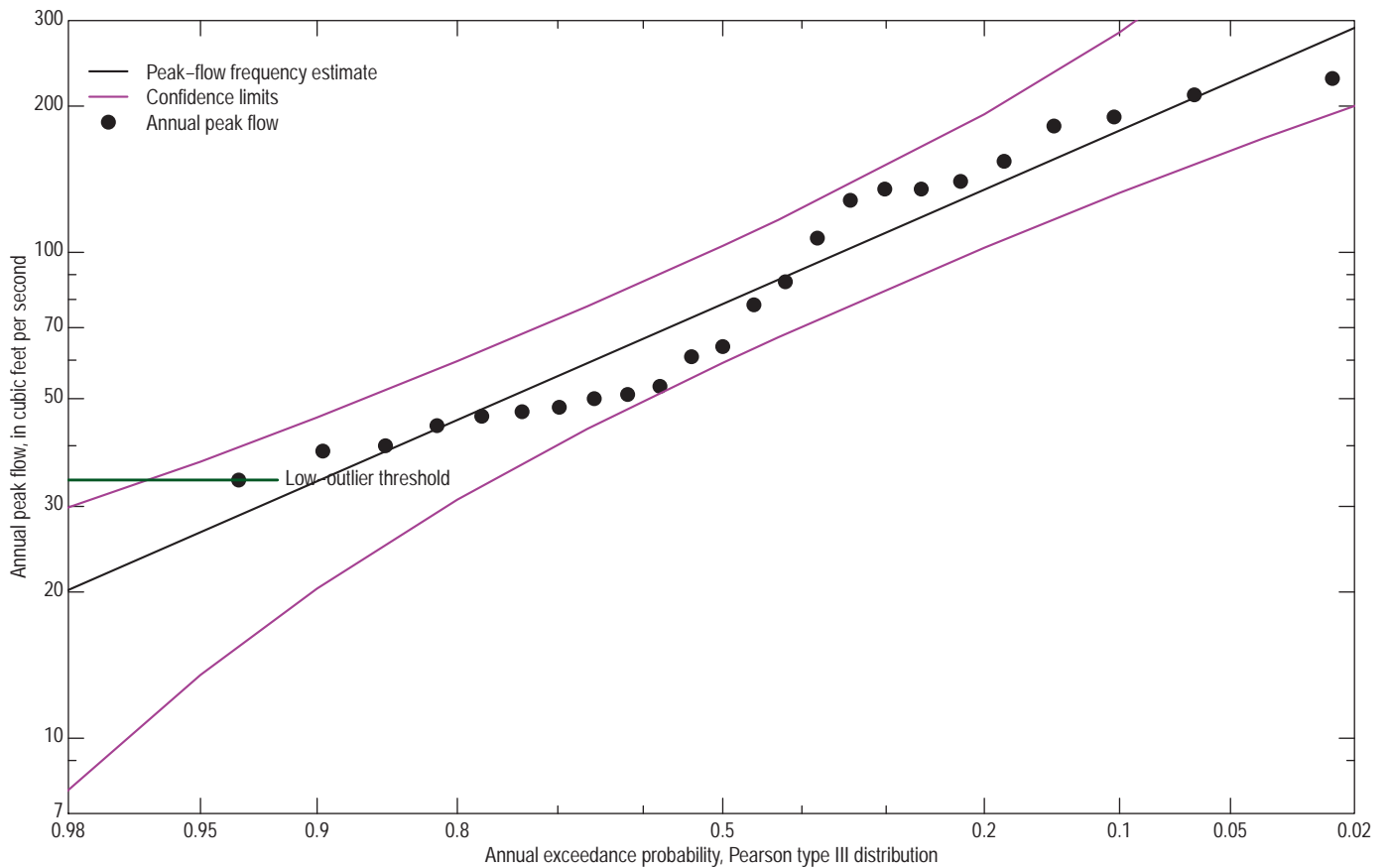
05474750 Beaver Creek tributary number 2 near Slayton, Minn.
